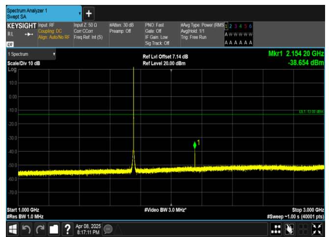
Band4-1.4MHz-QPSK-20393-1RB#0-1000~3000-PASS
