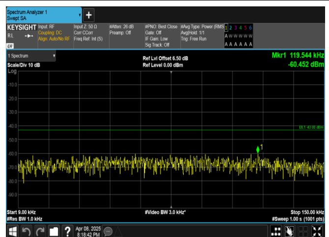
Band4-1.4MHz-QPSK-20393-1RB#5-0.009~0.15-PASS
