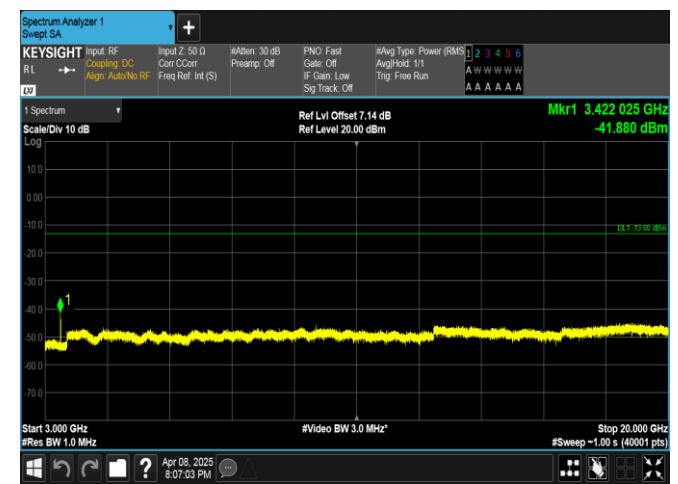
Band4-1.4MHz-QPSK-19957-1RB#5-3000~20000-PASS
