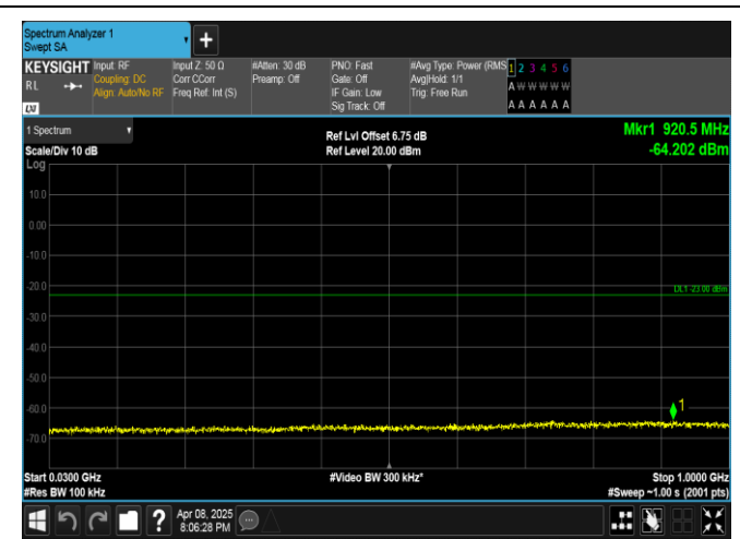
Band4-1.4MHz-QPSK-19957-1RB#5-30~1000-PASS
