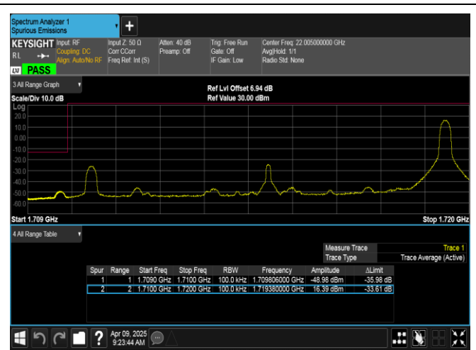
Band4-10MHz-16QAM-20000-1RB#49-PASS
