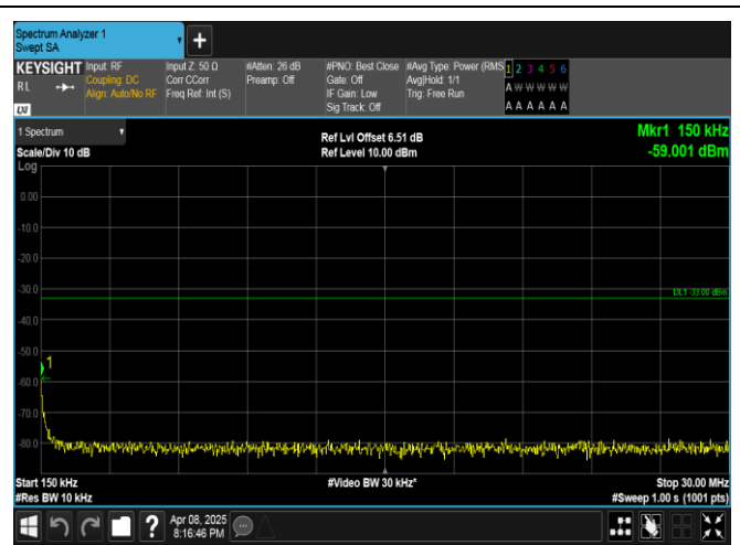
Band4-1.4MHz-QPSK-20393-1RB#0-0.15~30-PASS
