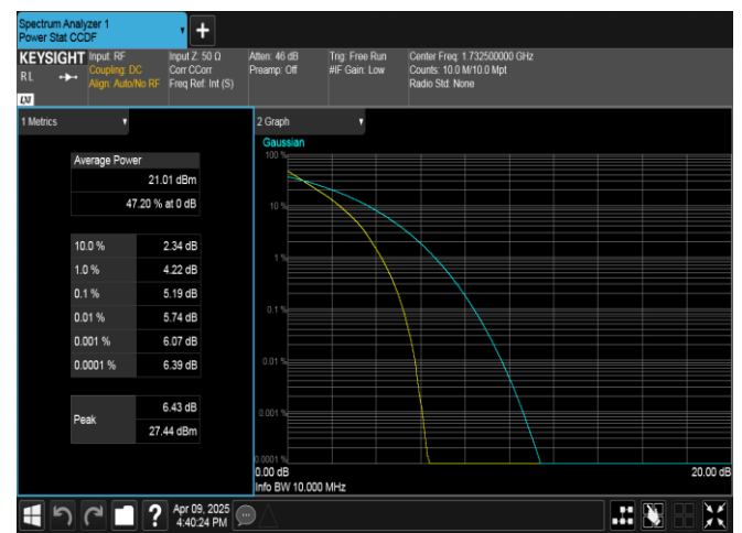
Band4-10MHz-QPSK-20175-50RB#0-PASS
