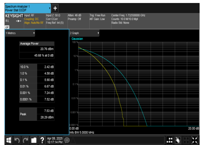
Band4-5MHz-QPSK-20175-25RB#0-PASS
