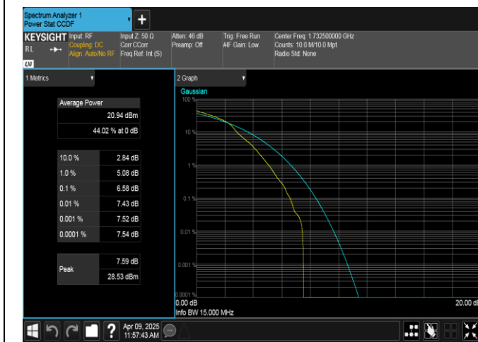
Band4-15MHz-16QAM-20175-1RB#0-PASS
