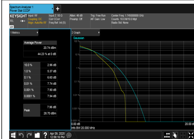
Band4-20MHz-16QAM-20300-1RB#0-PASS
