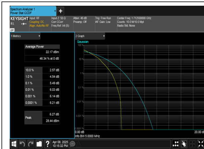
Band4-5MHz-QPSK-19975-1RB#0-PASS
