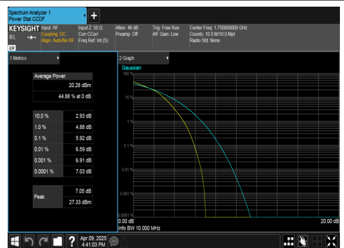
Band4-10MHz-16QAM-20350-50RB#0-PASS
