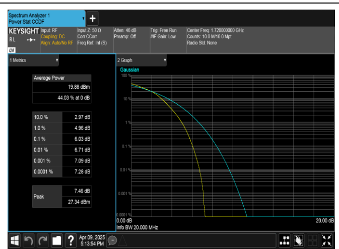
Band4-20MHz-16QAM-20050-100RB#0-PASS
