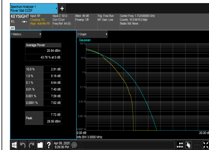
Band4-3MHz-16QAM-20175-1RB#0-PASS
