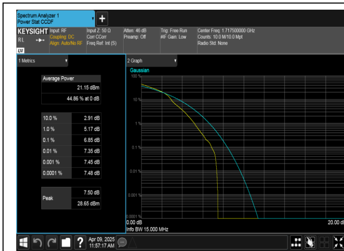
Band4-15MHz-16QAM-20025-1RB#0-PASS
