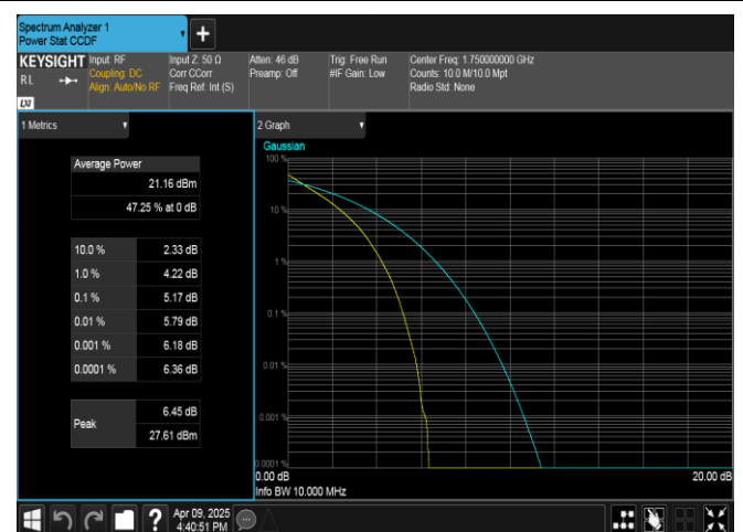
Band4-10MHz-QPSK-20350-50RB#0-PASS
