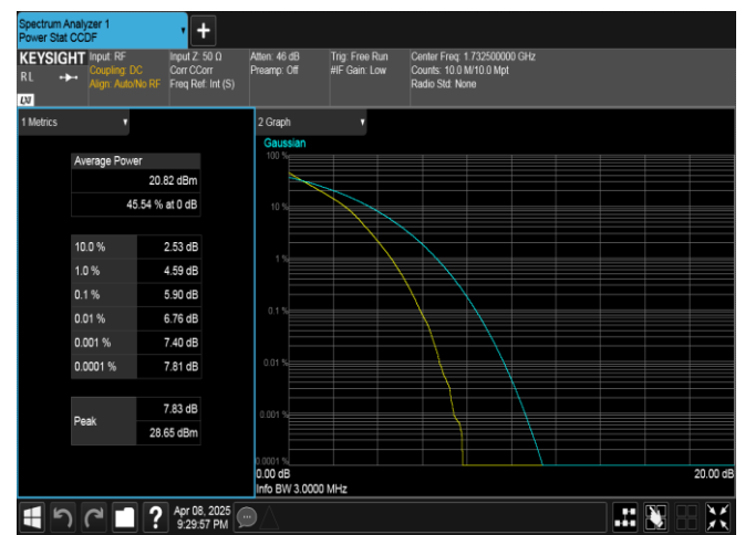
Band4-3MHz-QPSK-20175-15RB#0-PASS
