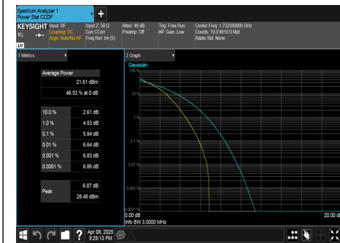
Band4-3MHz-QPSK-20175-1RB#0-PASS
