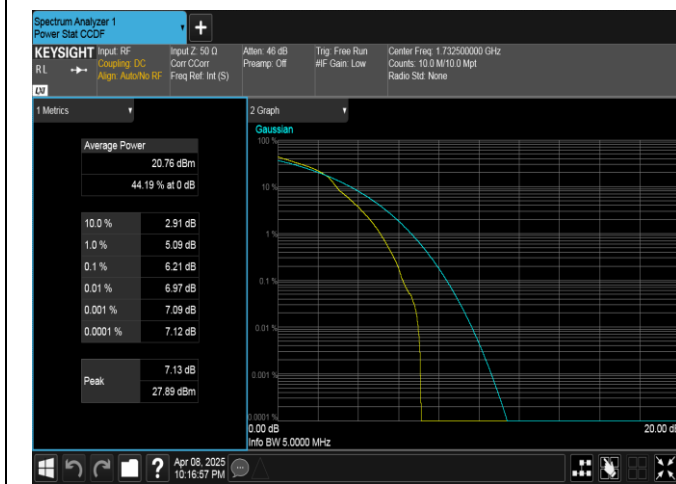
Band4-5MHz-16QAM-20175-1RB#0-PASS
