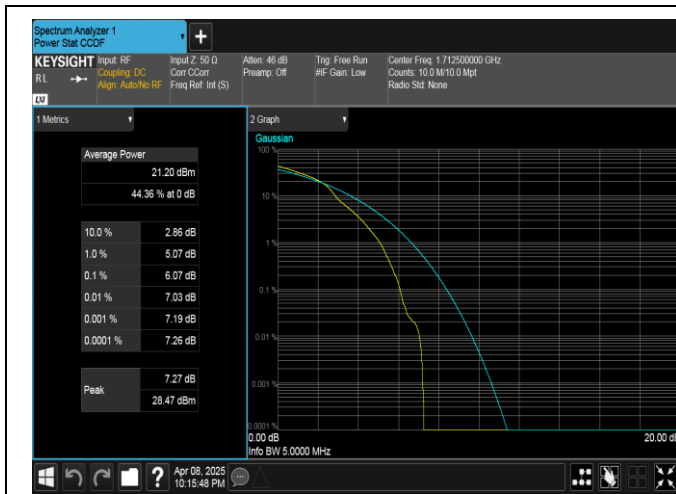
Band4-5MHz-16QAM-19975-1RB#0-PASS
