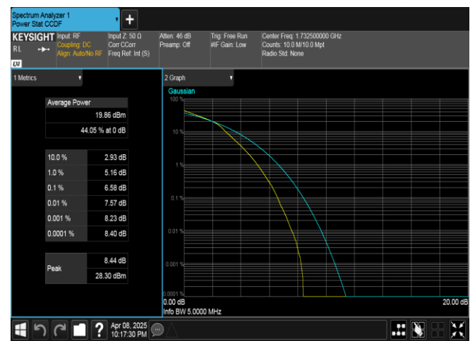
Band4-5MHz-16QAM-20175-25RB#0-PASS
