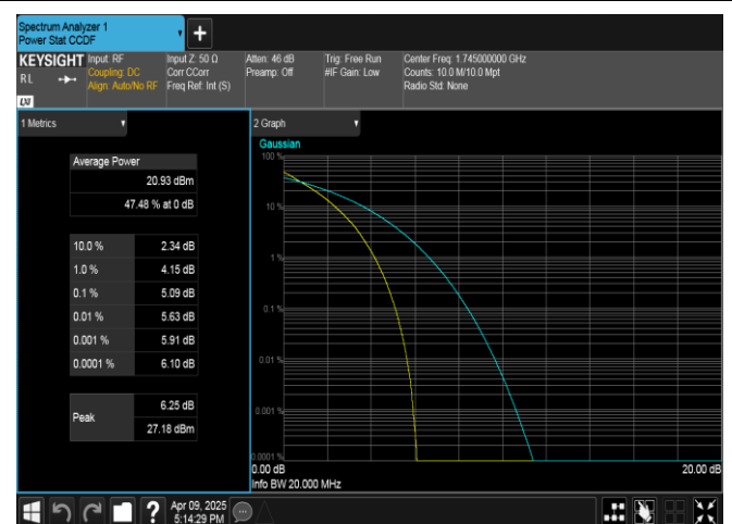
Band4-20MHz-QPSK-20300-100RB#0-PASS
