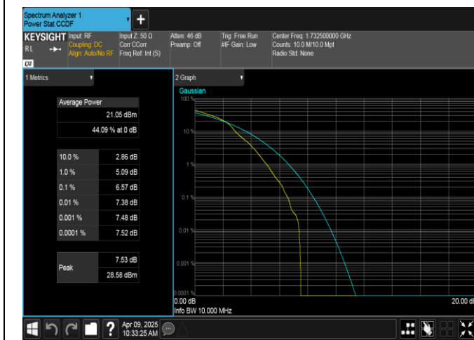
Band4-10MHz-16QAM-20175-1RB#0-PASS
