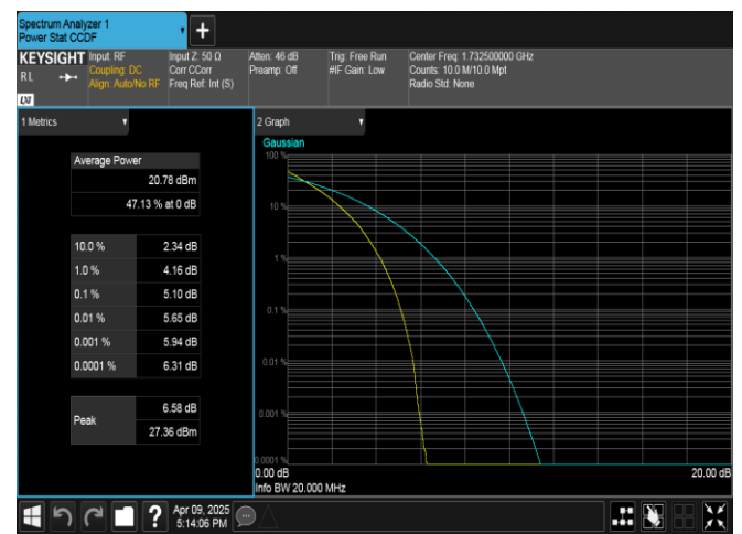
Band4-20MHz-QPSK-20175-100RB#0-PASS
