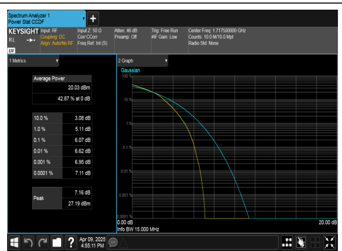
Band4-15MHz-16QAM-20025-75RB#0-PASS
