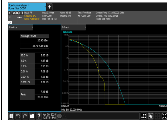
Band4-20MHz-16QAM-20175-1RB#0-PASS
