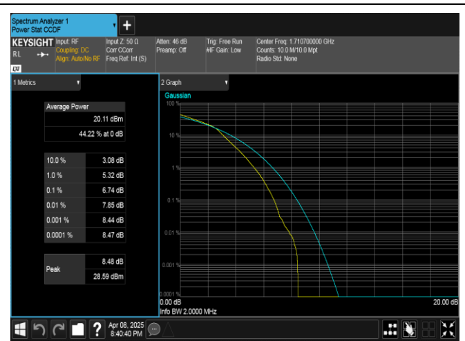
Band4-1.4MHz-16QAM-19957-6RB#0-PASS
