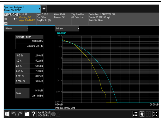
Band4-3MHz-16QAM-19965-15RB#0-PASS
