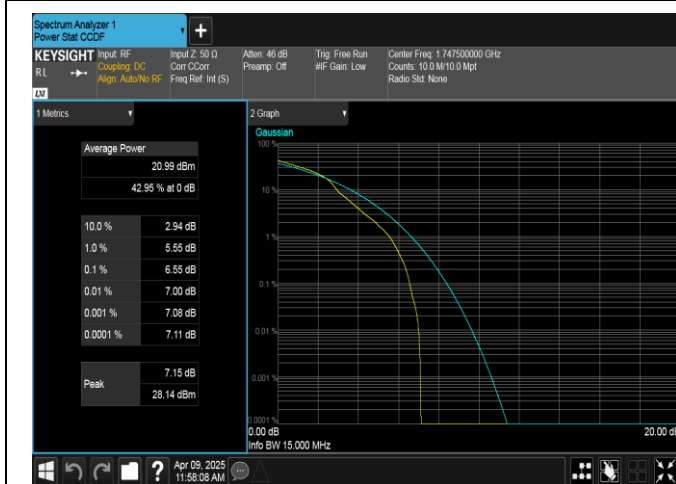
Band4-15MHz-16QAM-20325-1RB#0-PASS
