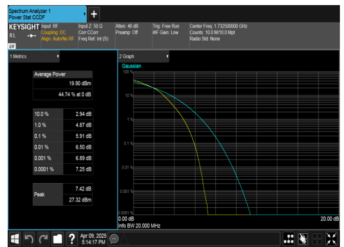
Band4-20MHz-16QAM-20175-100RB#0-PASS
