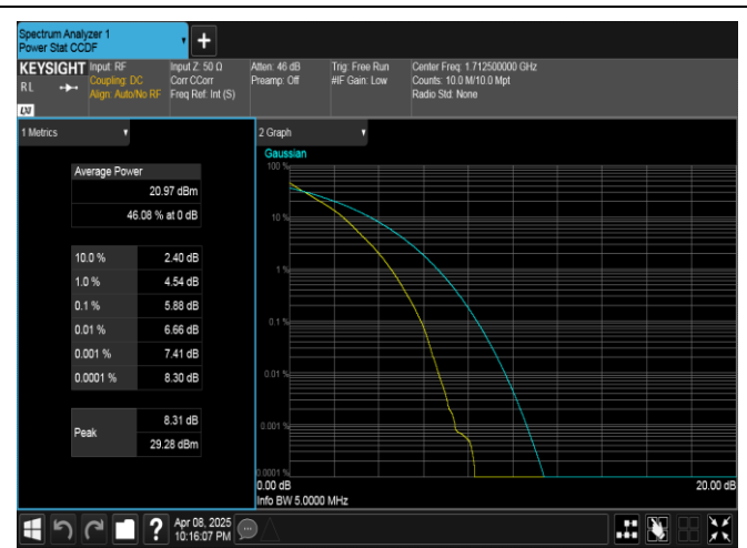
Band4-5MHz-QPSK-19975-25RB#0-PASS
