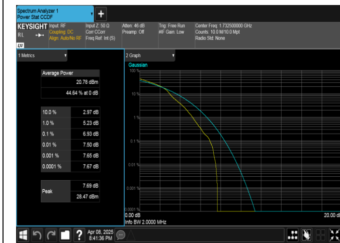
Band4-1.4MHz-16QAM-20175-1RB#0-PASS
