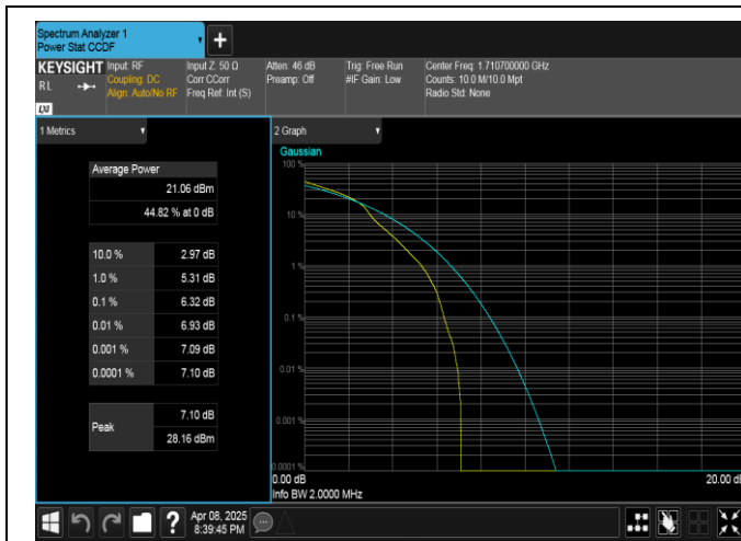
Band4-1.4MHz-16QAM-19957-1RB#0-PASS
