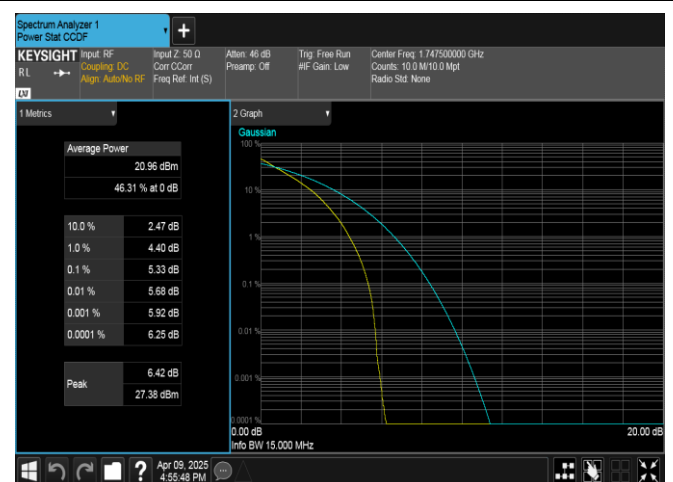
Band4-15MHz-QPSK-20325-75RB#0-PASS
