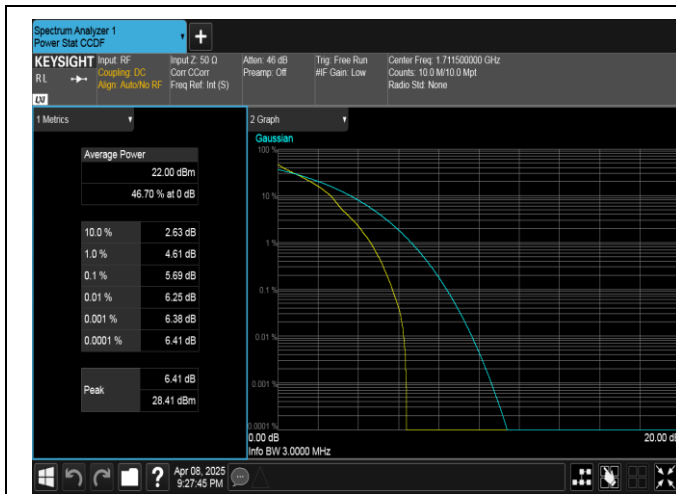
Band4-3MHz-QPSK-19965-1RB#0-PASS
