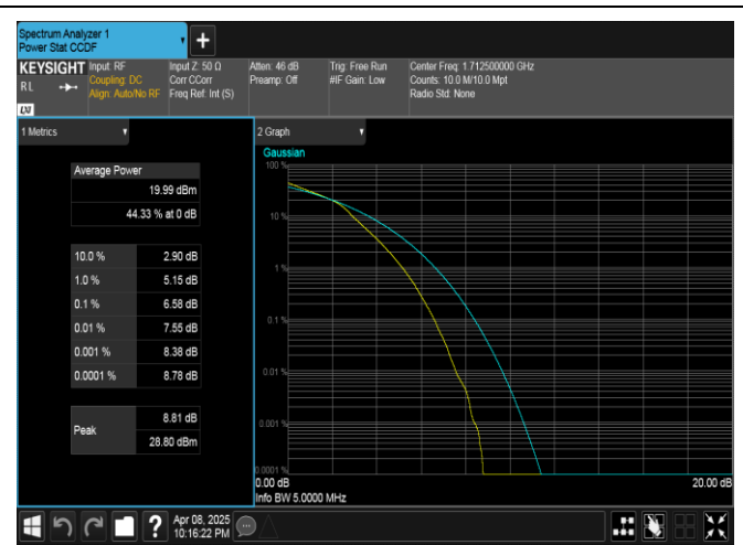
Band4-5MHz-16QAM-19975-25RB#0-PASS
