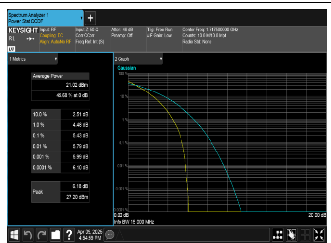
Band4-15MHz-QPSK-20025-75RB#0-PASS
