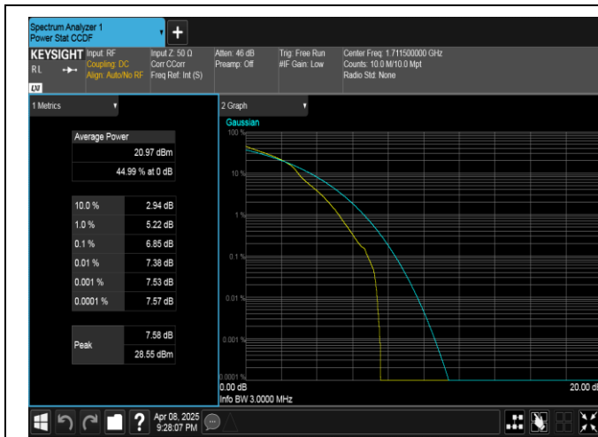
Band4-3MHz-16QAM-19965-1RB#0-PASS
