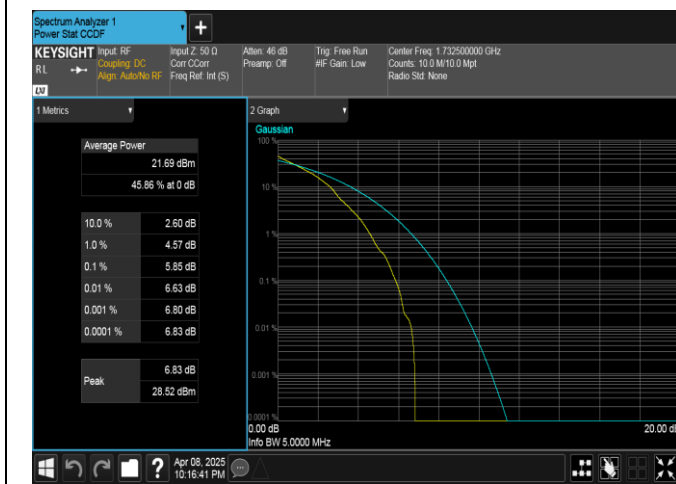
Band4-5MHz-QPSK-20175-1RB#0-PASS
