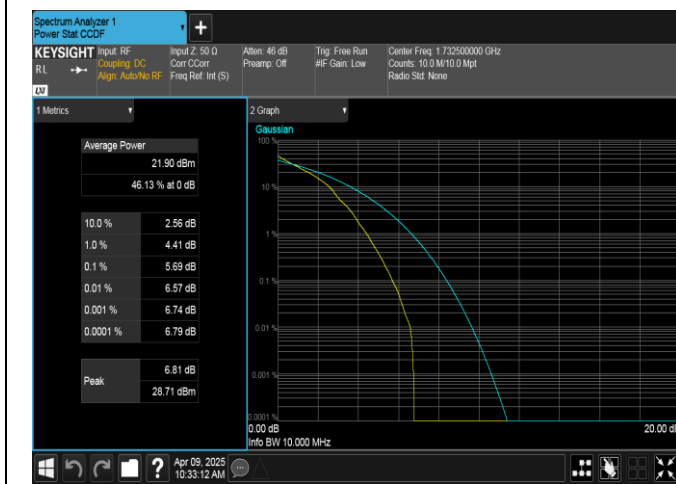
Band4-10MHz-QPSK-20175-1RB#0-PASS
