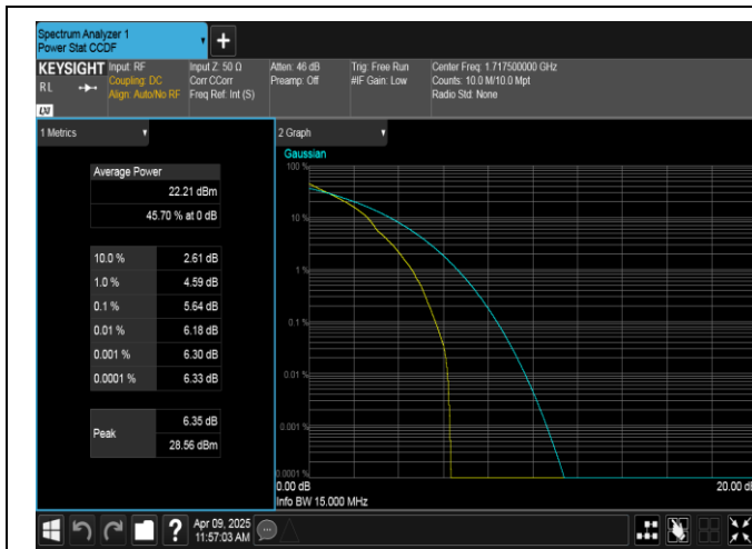
Band4-15MHz-QPSK-20025-1RB#0-PASS
