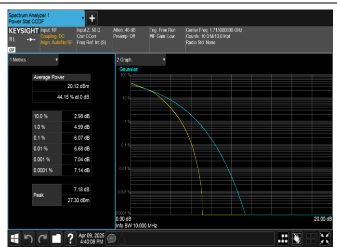
Band4-10MHz-16QAM-20000-50RB#0-PASS
