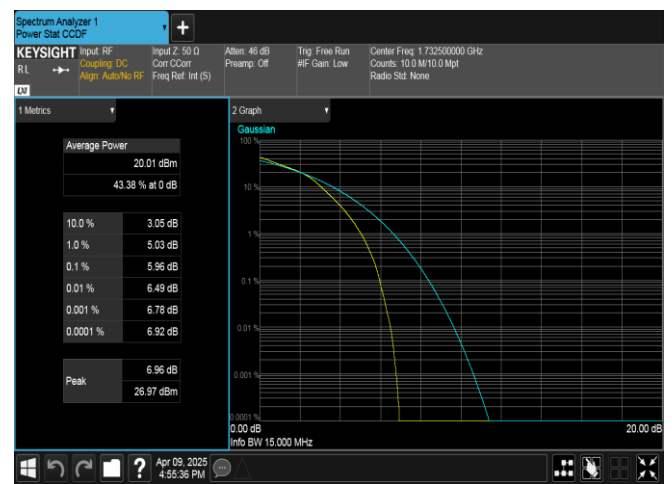
Band4-15MHz-16QAM-20175-75RB#0-PASS
