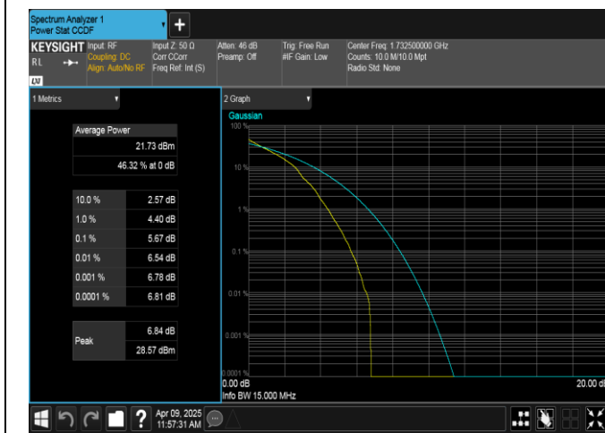
Band4-15MHz-QPSK-20175-1RB#0-PASS
