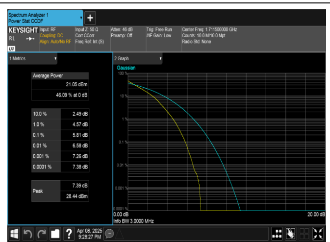
Band4-3MHz-QPSK-19965-15RB#0-PASS
