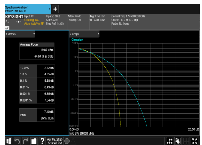
Band4-20MHz-16QAM-20300-100RB#0-PASS
