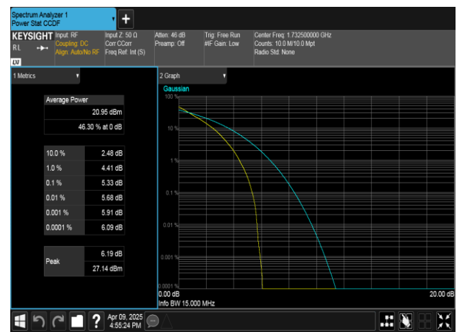
Band4-15MHz-QPSK-20175-75RB#0-PASS
