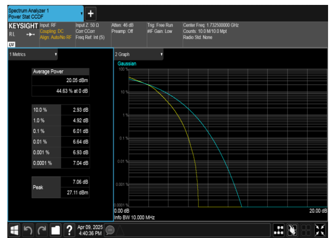
Band4-10MHz-16QAM-20175-50RB#0-PASS
