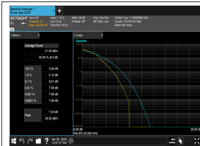
Band4-20MHz-16QAM-20050-1RB#0-PASS
