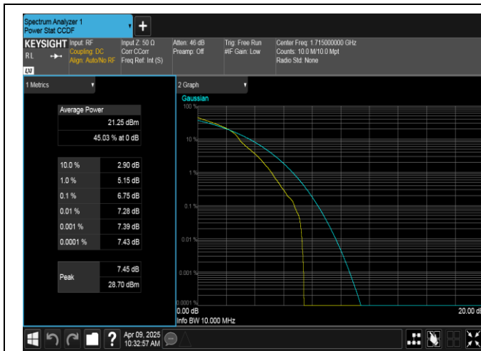
Band4-10MHz-16QAM-20000-1RB#0-PASS
