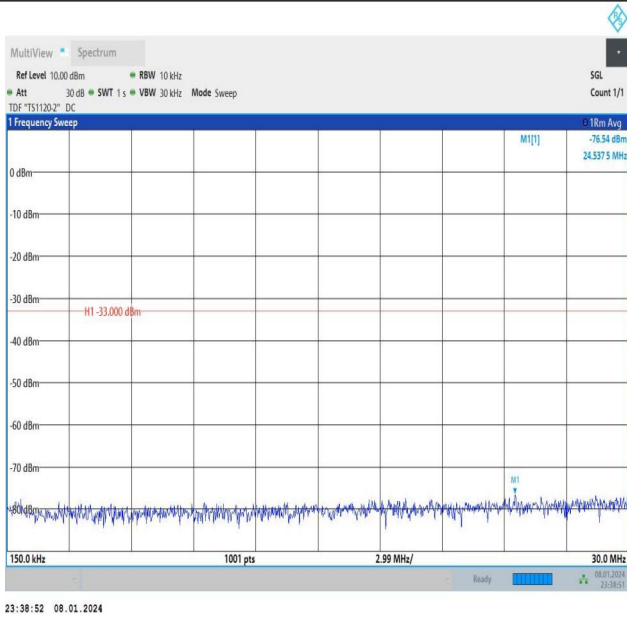
Band4_5MHz_16QAM_20375_25RB#0_0.15~30_0.15~30
