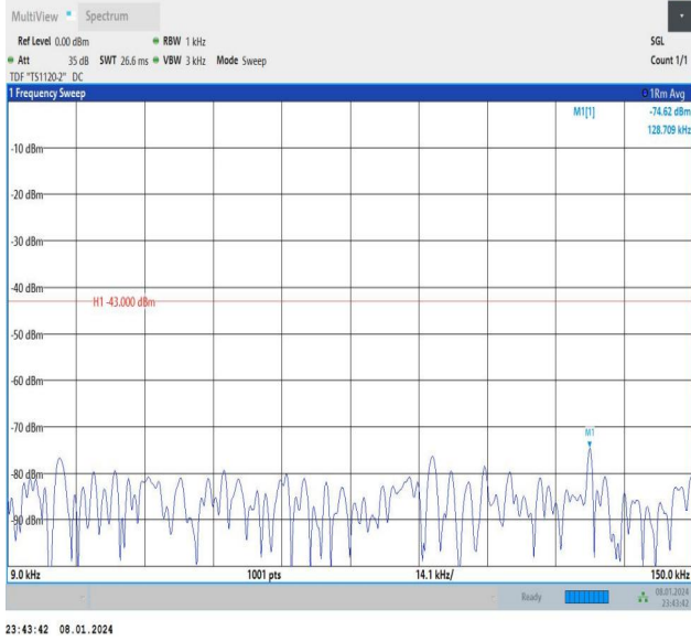
Band4_10MHz_QPSK_20175_1RB#49_0.009~0.15_0.009~0.15
