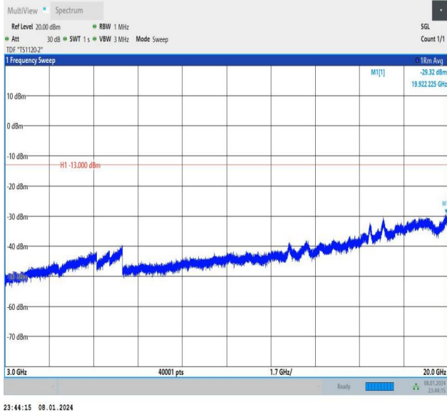
Band4_10MHz_QPSK_20175_1RB#49_3000~20000_3000~20000
