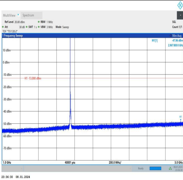
Band4_5MHz_16QAM_20375_1RB#0_1000~3000_1000~300 0
