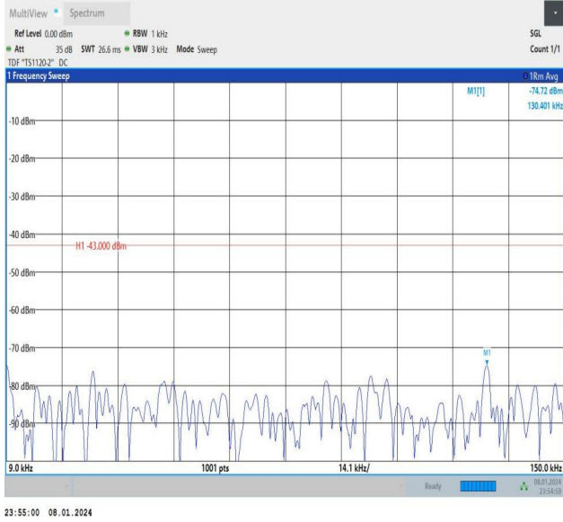
Band4_15MHz_16QAM_20175_1RB#74_0.009~0.15_0.009~0.15
