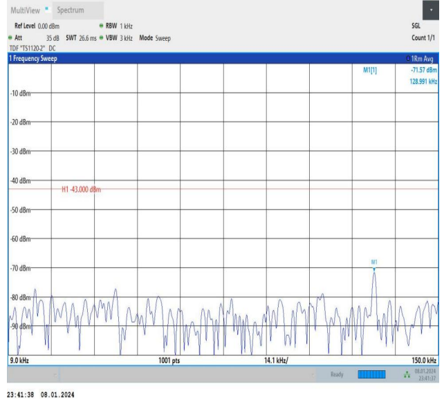
Band4_10MHz_16QAM_20000_1RB#49_0.009~0.15_0.009~0.15
