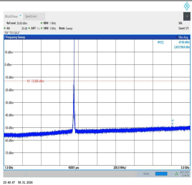
Band4_10MHz_QPSK_20350_1RB#49_1000~3000_1000~30
