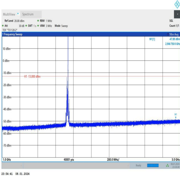
Band4_15MHz_QPSK_20175_1RB#74_1000~3000_1000~30 00
