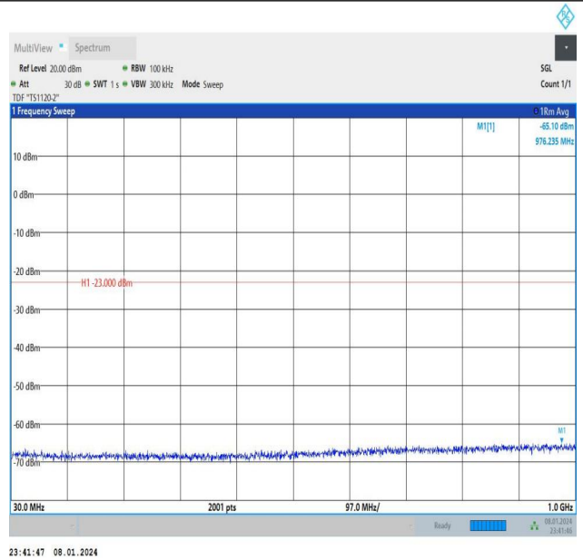
Band4_10MHz_16QAM_20000_1RB#49_30~1000_30~1000
