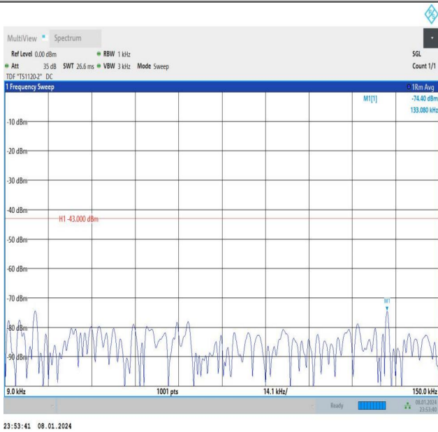
Band4_15MHz_16QAM_20175_1RB#0_0.009~0.15_0.009~0.15
