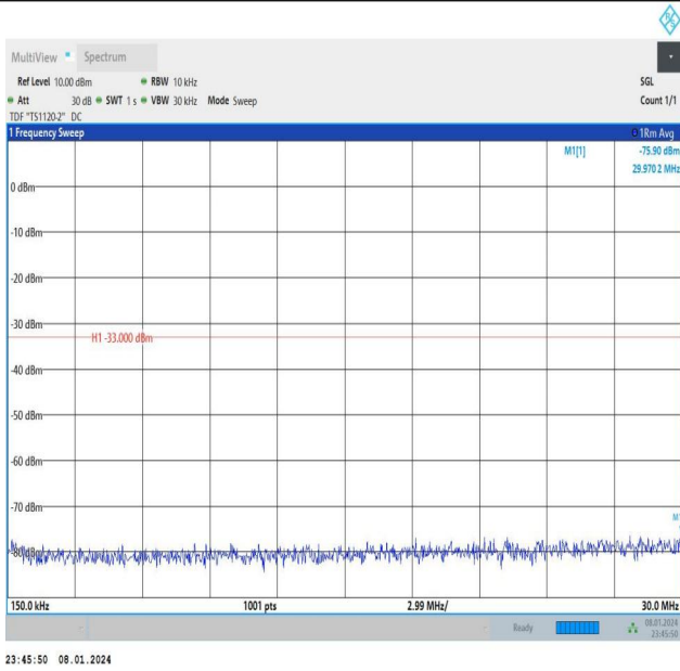
Band4_10MHz_16QAM_20350_1RB#0_0.15~30_0.15~30
