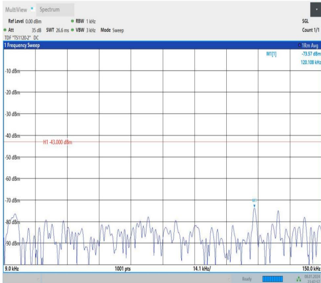
Band4_10MHz_QPSK_20000_50RB#0_0.009~0.15_0.009~0.15
