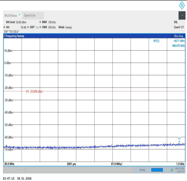
Band4_10MHz_16QAM_20350_1RB#49_30~1000_30~1000
