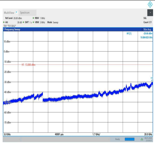
Band4_15MHz_QPSK_20025_1RB#0_3000~20000_3000~20
