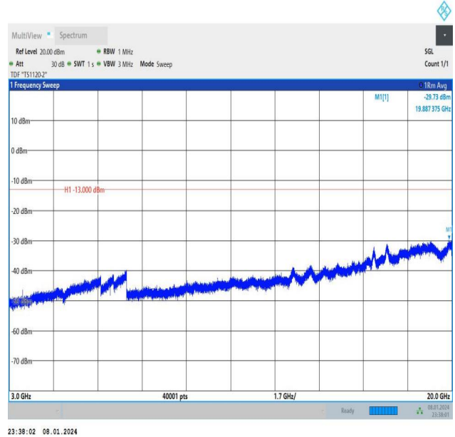
Band4_5MHz_16QAM_20375_1RB#24_3000~20000_3000~2 0000
