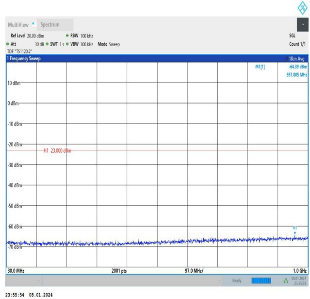
Band4_15MHz_QPSK_20325_1RB#0_30~1000_30~1000
