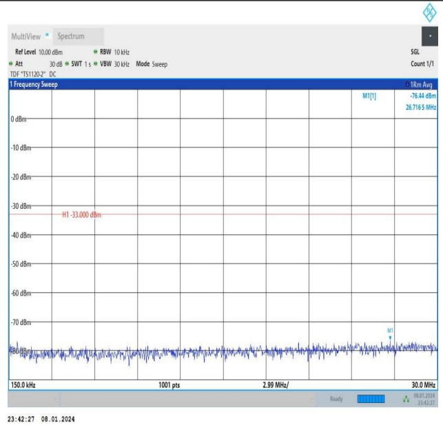
Band4_10MHz_QPSK_20175_1RB#0_0.15~30_0.15~30
