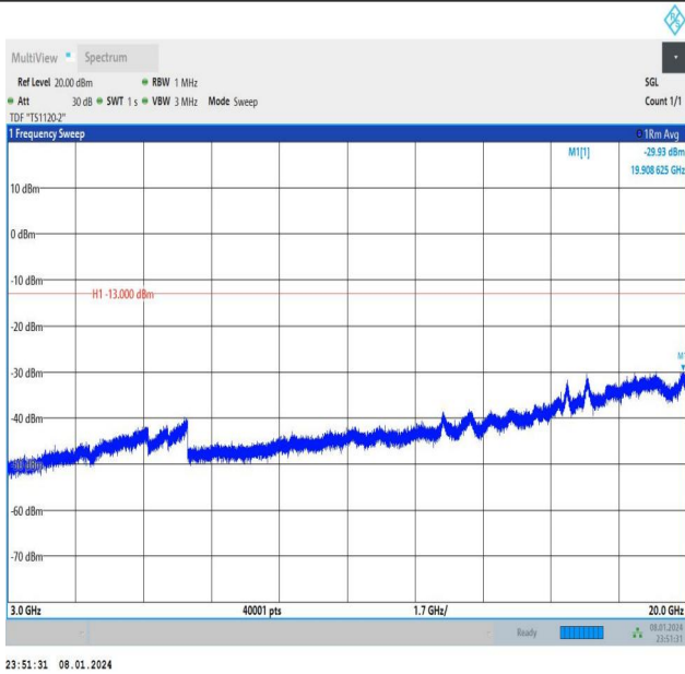
Band4_15MHz_16QAM_20025_1RB#0_3000~20000_3000~20000
