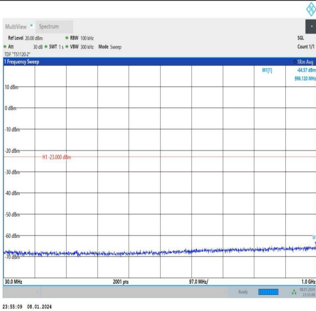
Band4_15MHz_16QAM_20175_1RB#74_30~1000_30~1000
