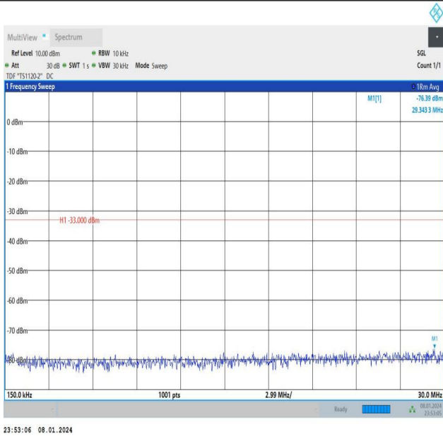
Band4_15MHz_QPSK_20175_1RB#0_0.15~30_0.15~30
