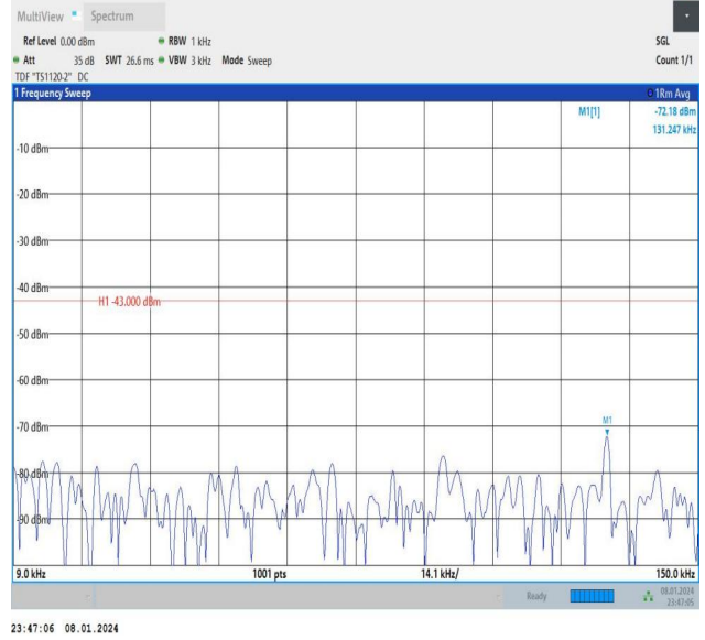
Band4_10MHz_16QAM_20350_1RB#49_0.009~0.15_0.009~0.15
