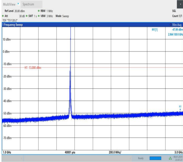
Band4_10MHz_16QAM_20350_1RB#49_1000~3000_1000~3000
