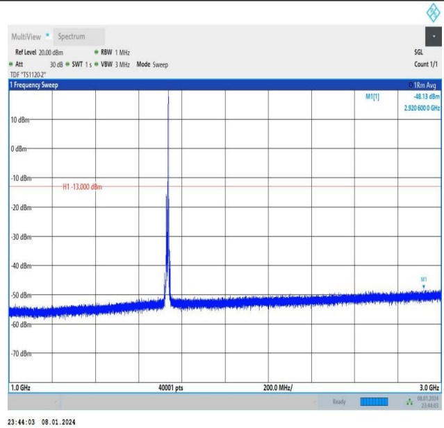
Band4_10MHz_QPSK_20175_1RB#49_1000~3000_1000~30
