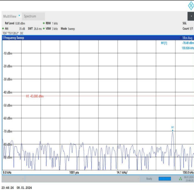
Band4_10MHz_QPSK_20350_1RB#49_0.009~0.15_0.009~0.15
