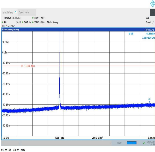
Band4_5MHz_16QAM_20375_1RB#24_1000~3000_1000~30 00
