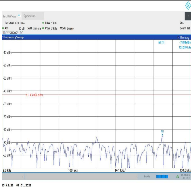
Band4_10MHz_QPSK_20175_1RB#0_0.009~0.15_0.009~0.15
