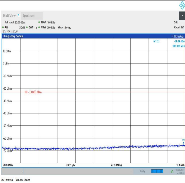
Band4_10MHz_QPSK_20000_1RB#0_30~1000_30~1000
