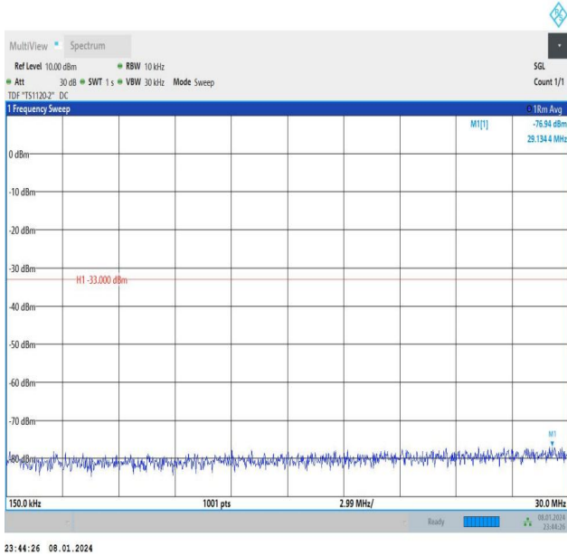
Band4_10MHz_16QAM_20175_1RB#49_0.15~30_0.15~30
