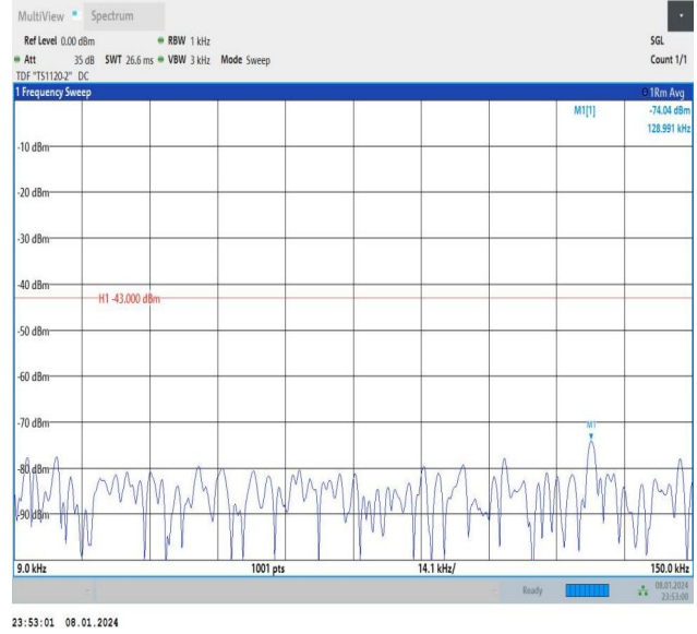
Band4_15MHz_QPSK_20175_1RB#0_0.009~0.15_0.009~0.1 5
