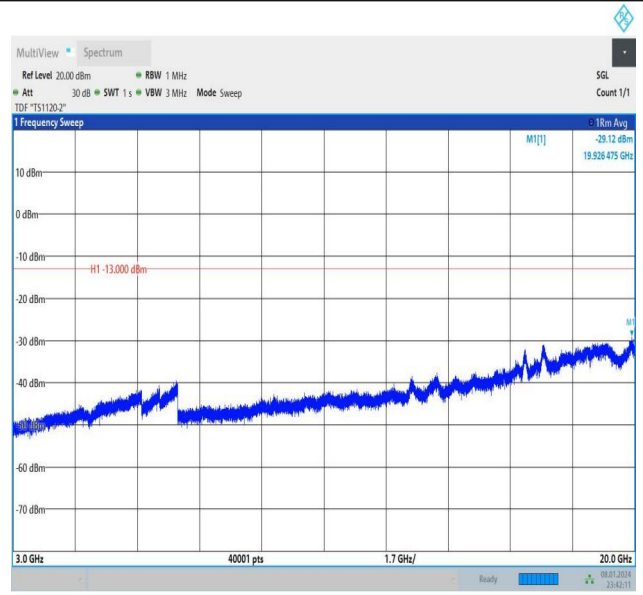
Band4_10MHz_16QAM_20000_1RB#49_3000~20000_3000~20000
