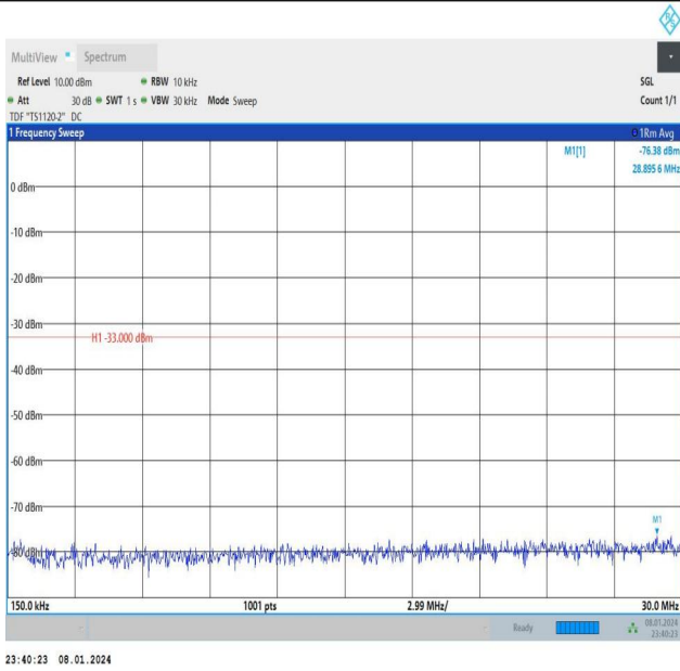
Band4_10MHz_16QAM_20000_1RB#0_0.15~30_0.15~30
