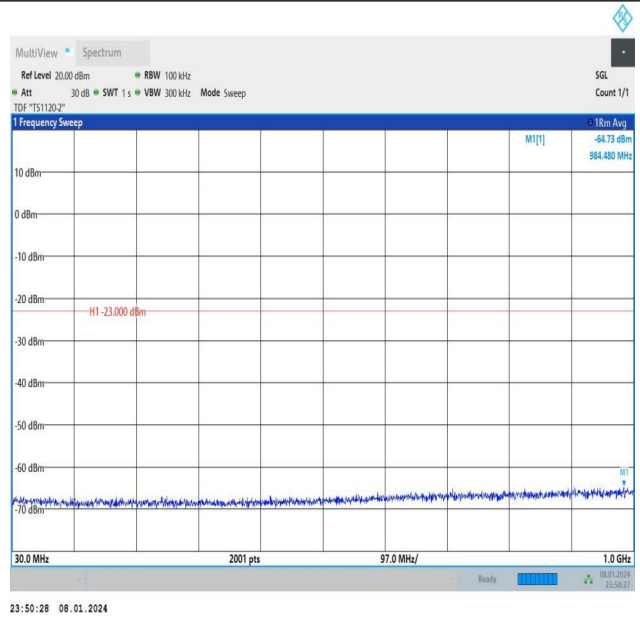
Band4_15MHz_QPSK_20025_1RB#0_30~1000_30~1000
