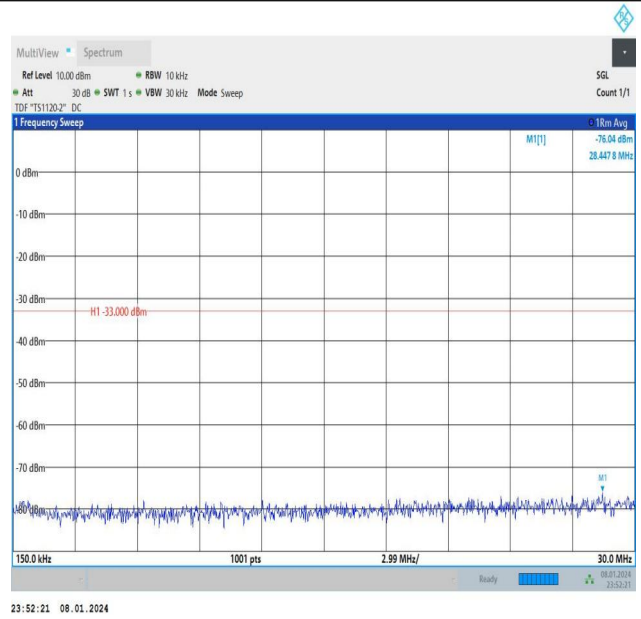
Band4_15MHz_16QAM_20025_1RB#74_0.15~30_0.15~30
