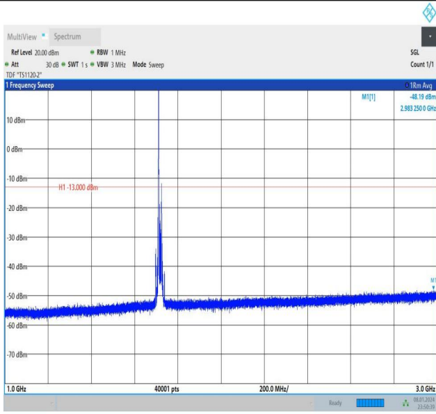
Band4_15MHz_QPSK_20025_1RB#0_1000~3000_1000~300
