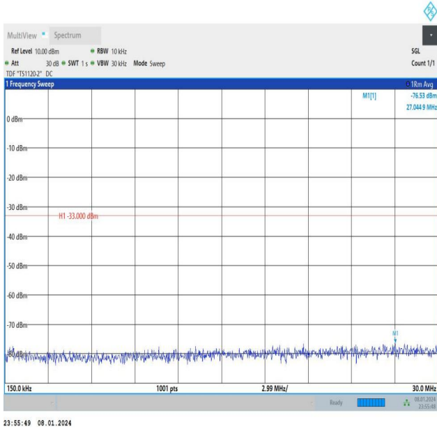
Band4_15MHz_QPSK_20325_1RB#0_0.15~30_0.15~30
