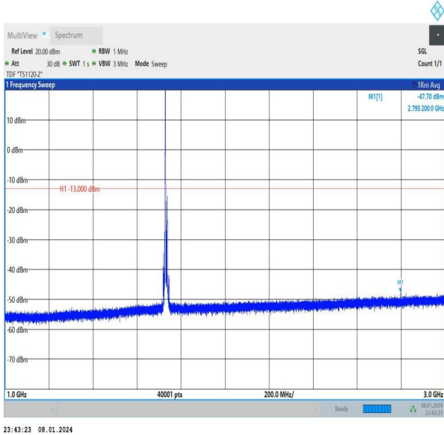
Band4_10MHz_16QAM_20175_1RB#0_1000~3000_1000~30 00
