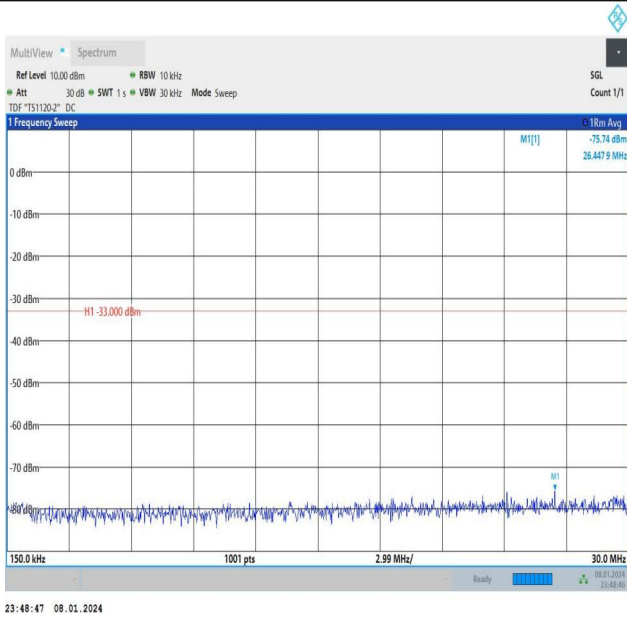
Band4_10MHz_QPSK_20175_50RB#0_0.15~30_0.15~30
