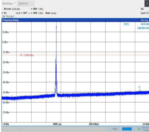
Band4_10MHz_16QAM_20175_1RB#49_1000~3000_1000~3000
