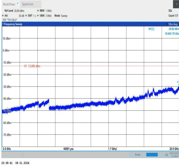
Band4_5MHz_QPSK_20375_25RB#0_3000~20000_3000~20000
