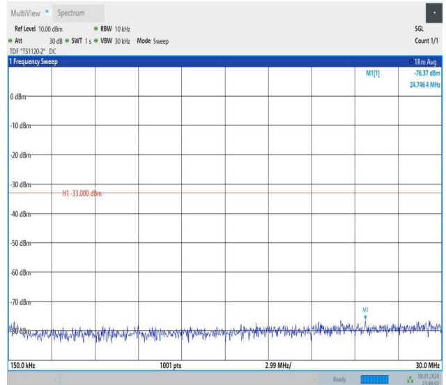
Band4_10MHz_QPSK_20000_50RB#0_0.15~30_0.15~30
