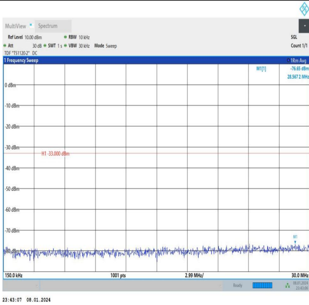
Band4_10MHz_16QAM_20175_1RB#0_0.15~30_0.15~30
