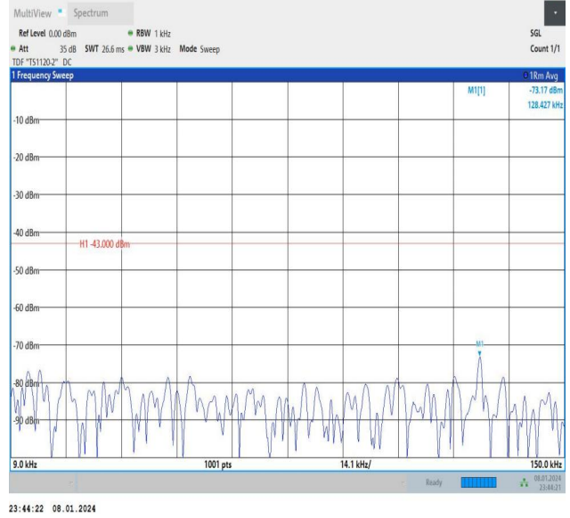
Band4_10MHz_16QAM_20175_1RB#49_0.009~0.15_0.009~0.15
