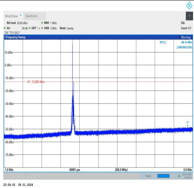
Band4_15MHz_16QAM_20175_1RB#0_1000~3000_1000~3000
