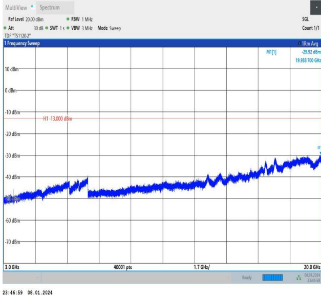
Band4_10MHz_QPSK_20350_1RB#49_3000~20000_3000~20000
