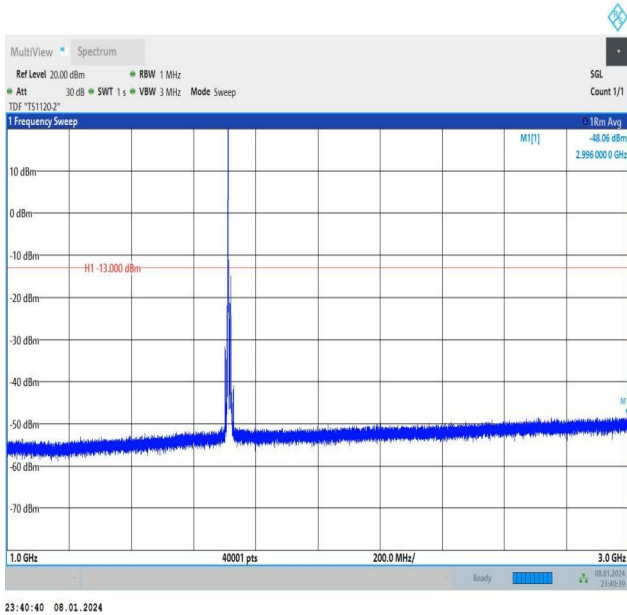
Band4_10MHz_16QAM_20000_1RB#0_1000~3000_1000~3000
