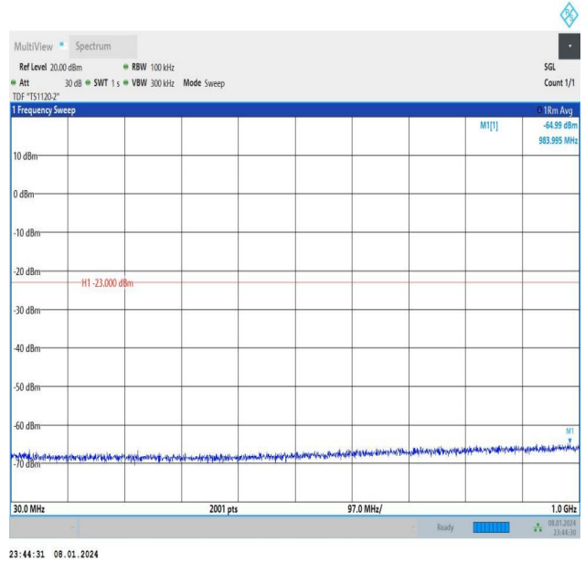
Band4_10MHz_16QAM_20175_1RB#49_30~1000_30~1000
