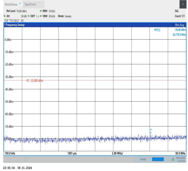
Band4_15MHz_16QAM_20175_1RB#74_0.15~30_0.15~30
