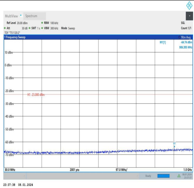
Band4_5MHz_16QAM_20375_1RB#24_30~1000_30~1000
