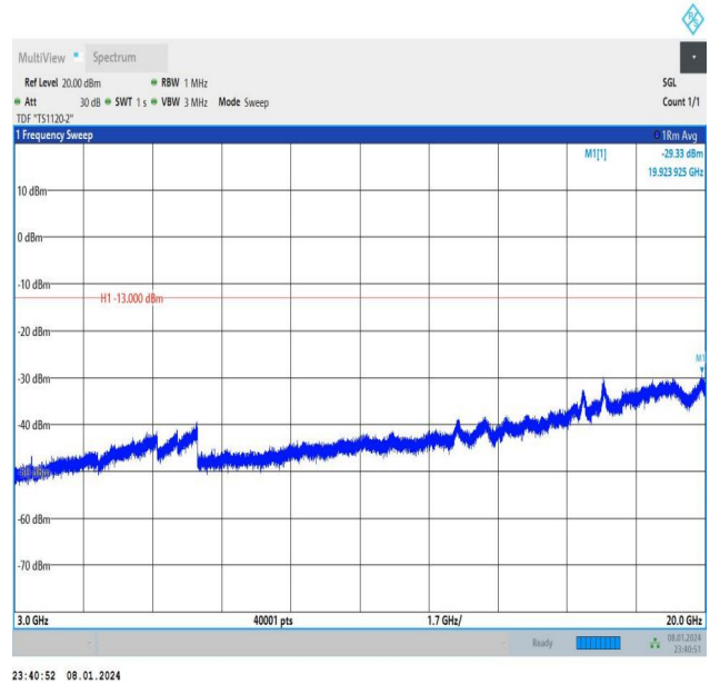
Band4_10MHz_16QAM_20000_1RB#0_3000~20000_3000~20000
