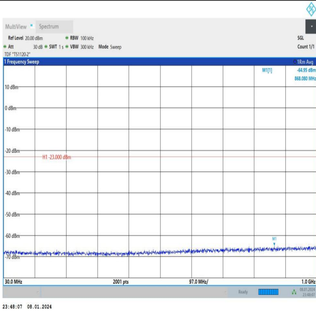
Band4_10MHz_QPSK_20000_50RB#0_30~1000_30~1000
