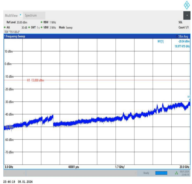
Band4_10MHz_16QAM_20350_1RB#0_3000~20000_3000~2 0000
