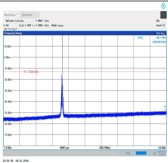
Band4_15MHz_16QAM_20025_1RB#74_1000~3000_1000~3000
