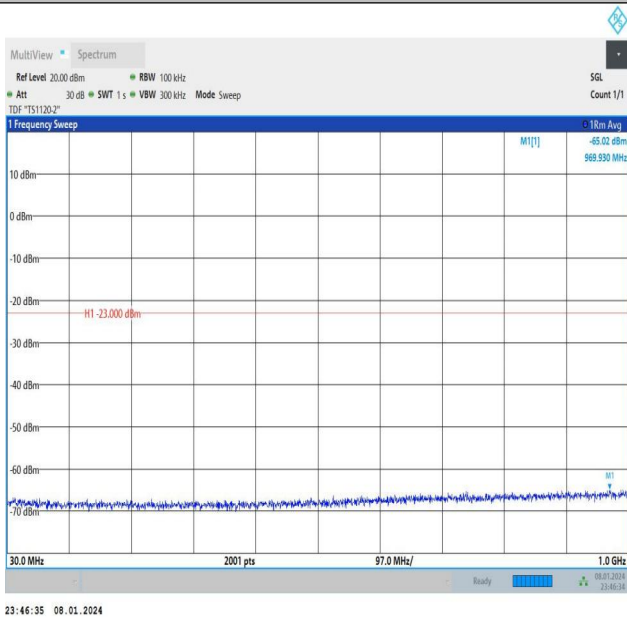
Band4_10MHz_QPSK_20350_1RB#49_30~1000_30~1000
