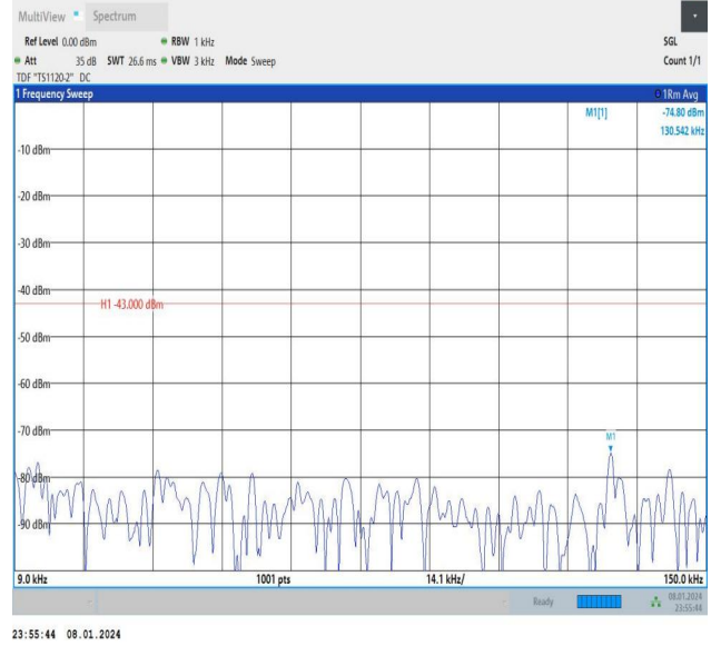
Band4_15MHz_QPSK_20325_1RB#0_0.009~0.15_0.009~0.1 5
