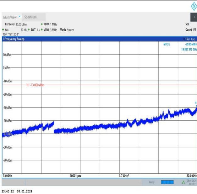
Band4_10MHz_QPSK_20000_1RB#0_3000~20000_3000~20000 000
