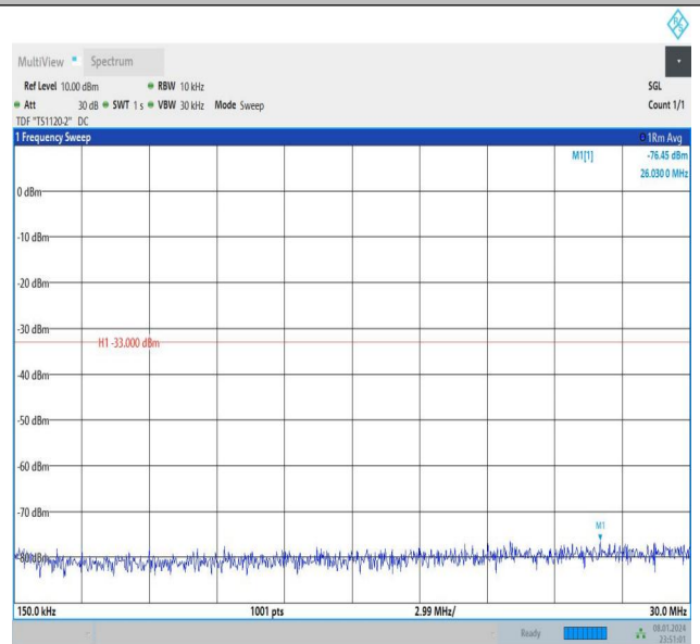
Band4_15MHz_16QAM_20025_1RB#0_0.15~30_0.15~30
