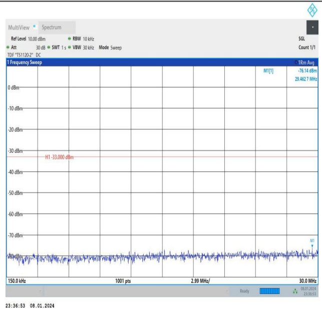
Band4_5MHz_QPSK_20375_1RB#24_0.15~30_0.15~30
