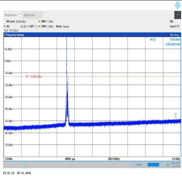
Band4_15MHz_16QAM_20025_1RB#0_1000~3000_1000~3000
