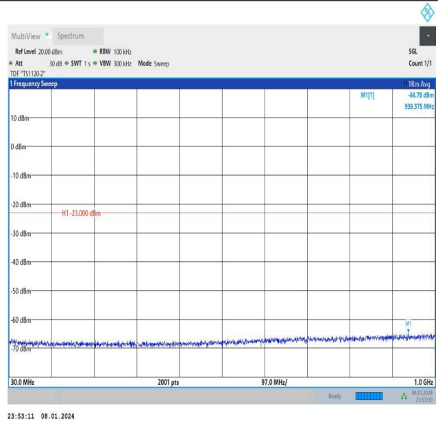
Band4_15MHz_QPSK_20175_1RB#0_30~1000_30~1000
