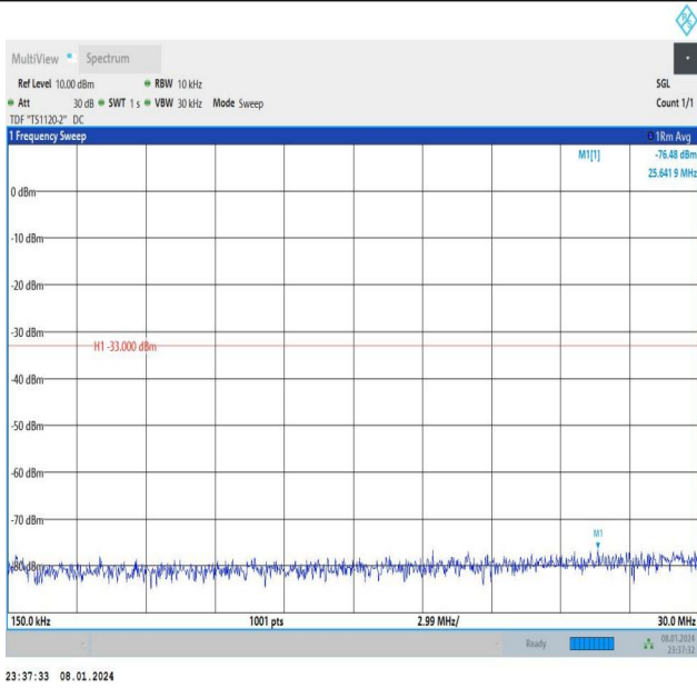
Band4_5MHz_16QAM_20375_1RB#24_0.15~30_0.15~30
