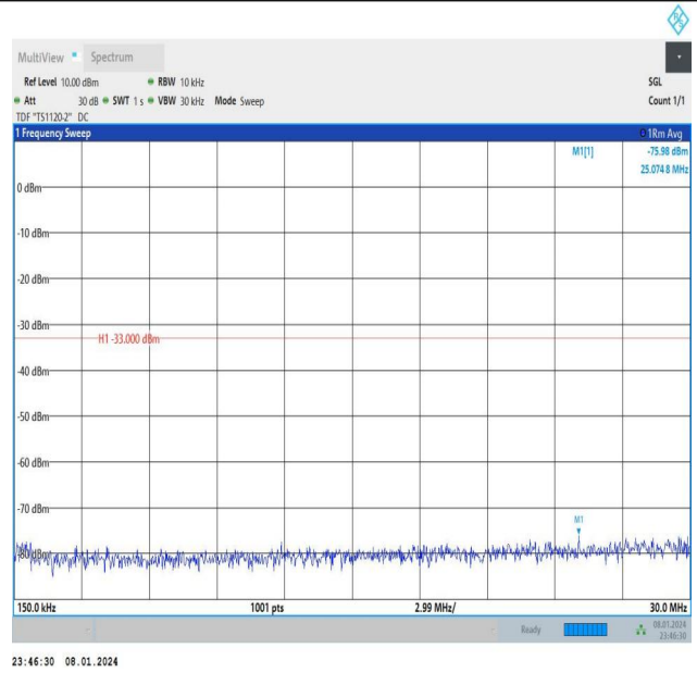
Band4_10MHz_QPSK_20350_1RB#49_0.15~30_0.15~30
