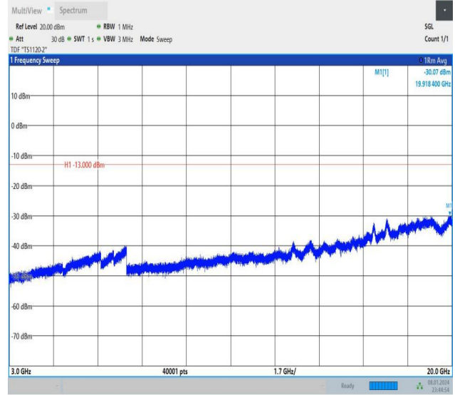
Band4_10MHz_16QAM_20175_1RB#49_3000~20000_3000~20000
