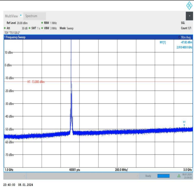
Band4_10MHz_QPSK_20000_1RB#0_1000~3000_1000~300 0
