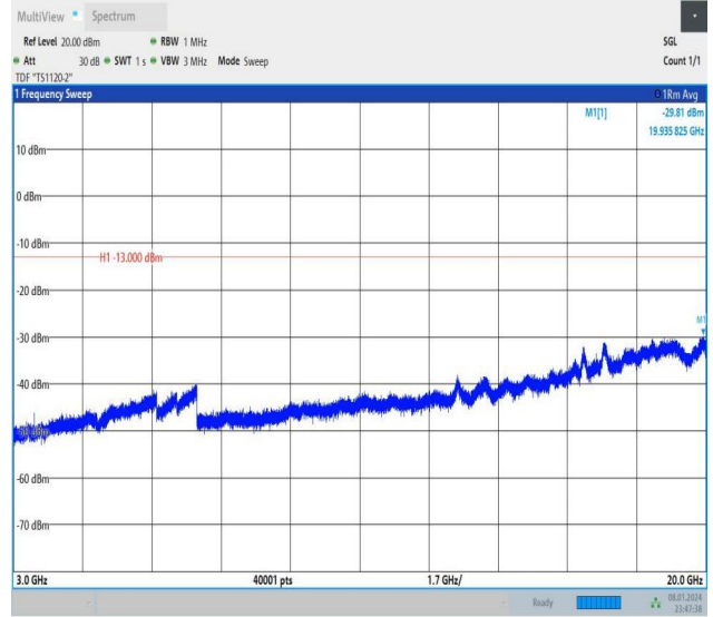
Band4_10MHz_16QAM_20350_1RB#49_3000~20000_3000~20000
