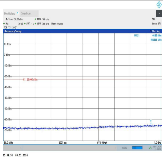
Band4_15MHz_QPSK_20175_1RB#74_30~1000_30~1000
