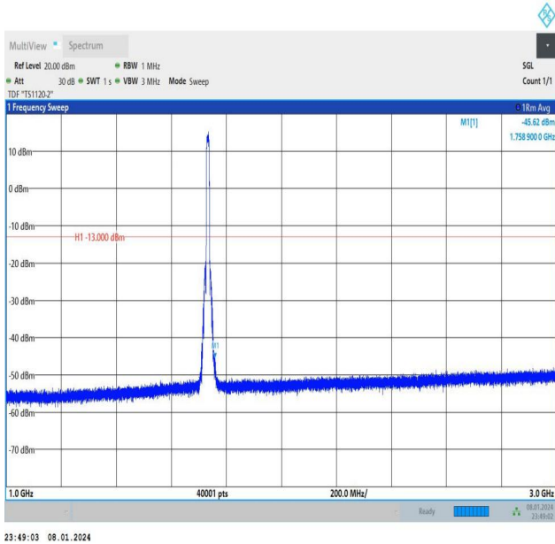
Band4_10MHz_QPSK_20175_50RB#0_1000~3000_1000~30 00
