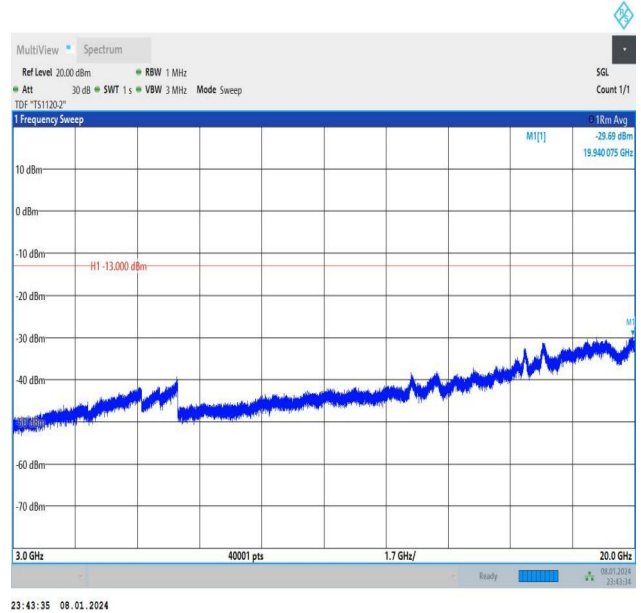
Band4_10MHz_16QAM_20175_1RB#0_3000~20000_3000~2 0000
