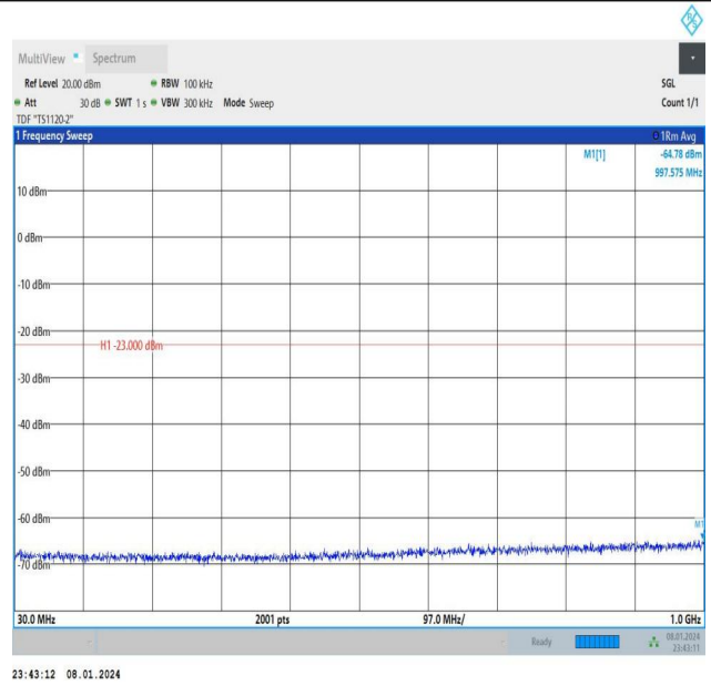
Band4_10MHz_16QAM_20175_1RB#0_30~1000_30~1000
