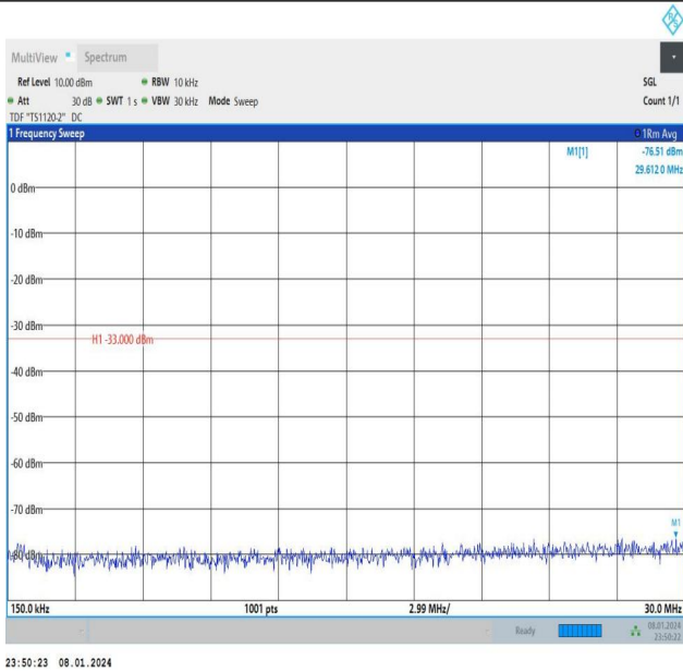
Band4_15MHz_QPSK_20025_1RB#0_0.15~30_0.15~30
