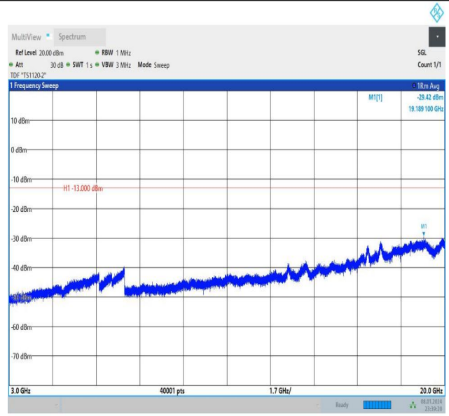
Band4_5MHz_16QAM_20375_25RB#0_3000~20000_3000~20000 0000
