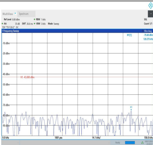
Band4_15MHz_16QAM_20025_1RB#0_0.009~0.15_0.009~0.15
