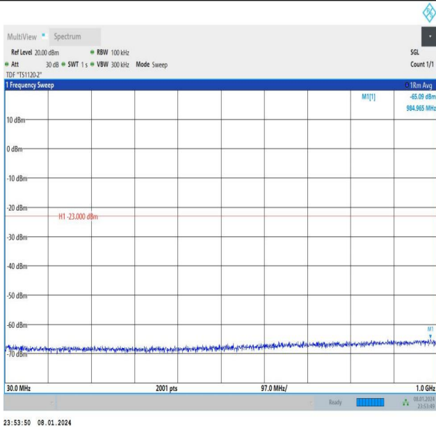
Band4_15MHz_16QAM_20175_1RB#0_30~1000_30~1000
