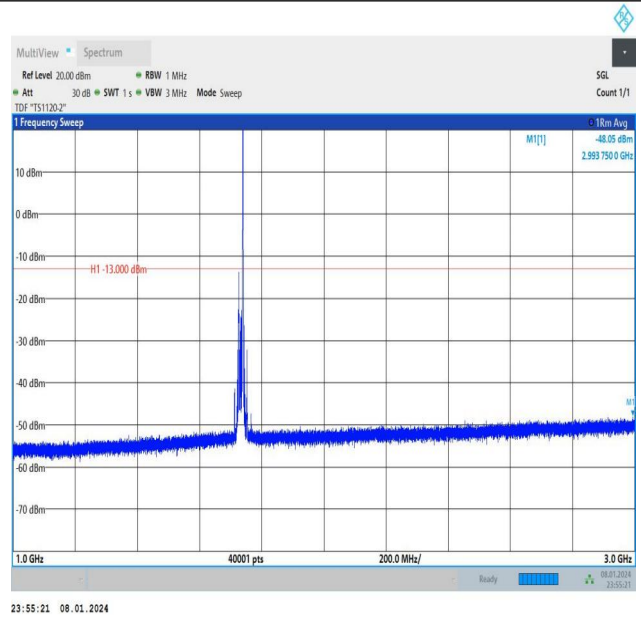
Band4_15MHz_16QAM_20175_1RB#74_1000~3000_1000~3000
