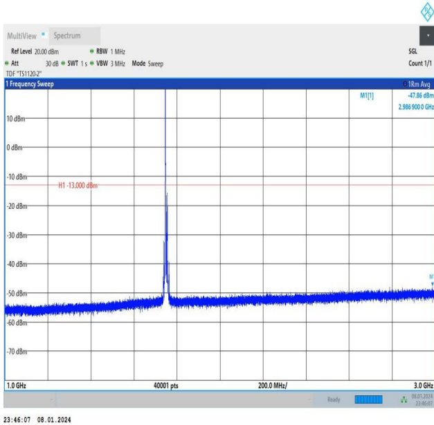
Band4_10MHz_16QAM_20350_1RB#0_1000~3000_1000~30 00
