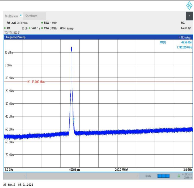
Band4_10MHz_QPSK_20000_50RB#0_1000~3000_1000~3000
