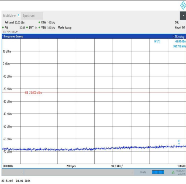
Band4_15MHz_16QAM_20025_1RB#0_30~1000_30~1000
