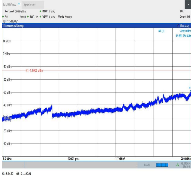
Band4_15MHz_16QAM_20025_1RB#74_3000~20000_3000~20000
