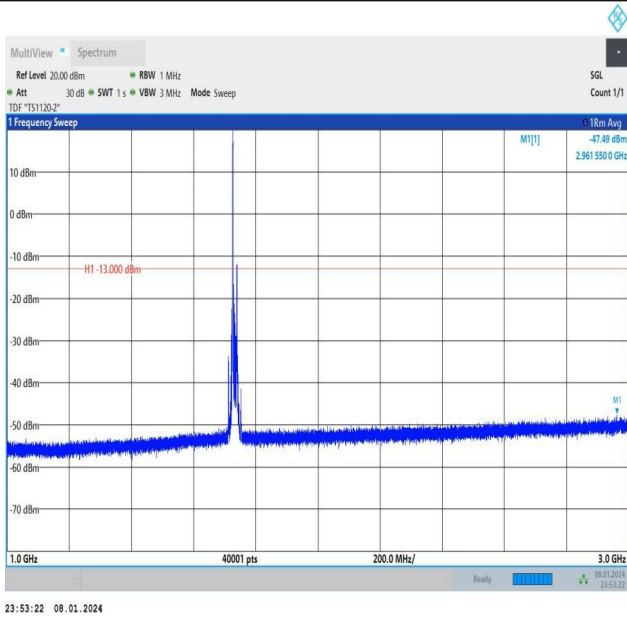
Band4_15MHz_QPSK_20175_1RB#0_1000~3000_1000~3000
