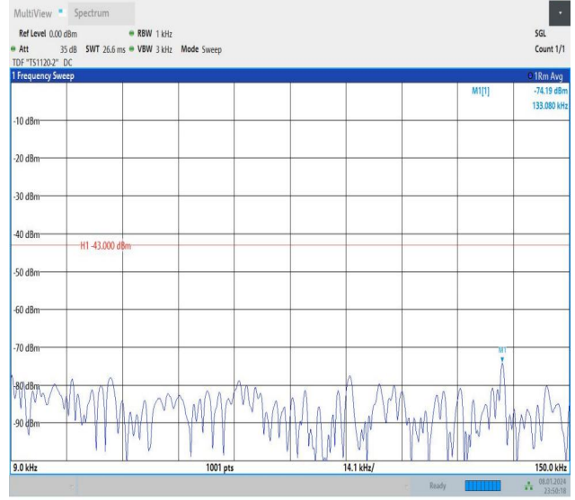
Band4_15MHz_QPSK_20025_1RB#0_0.009~0.15_0.009~0.15
