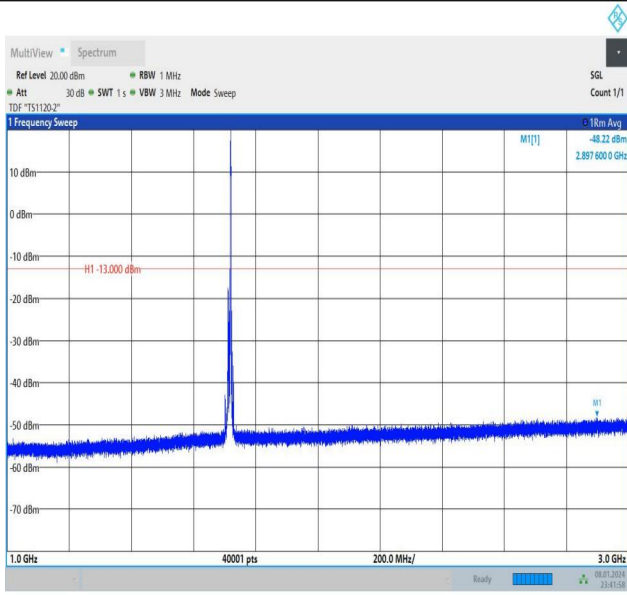
Band4_10MHz_16QAM_20000_1RB#49_1000~3000_1000~3000
