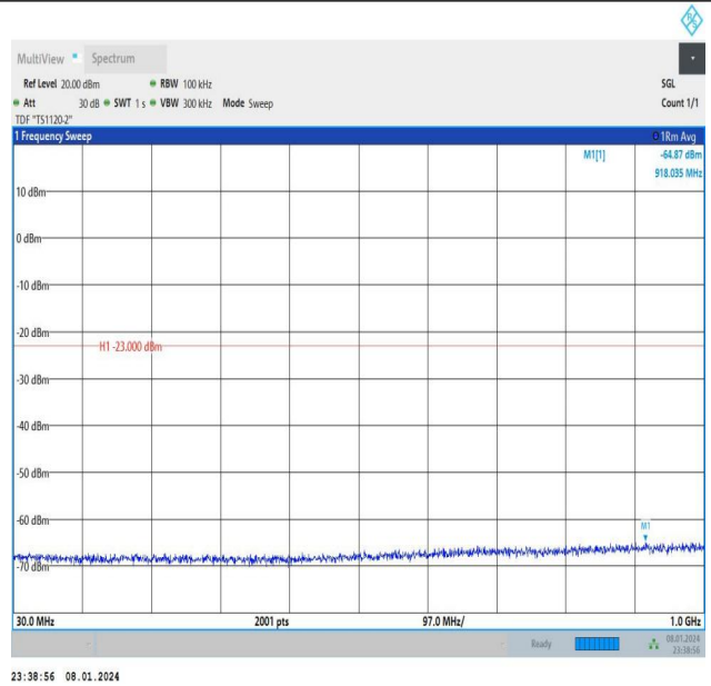
Band4_5MHz_16QAM_20375_25RB#0_30~1000_30~1000
