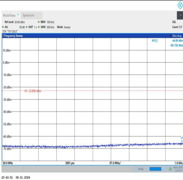
Band4_10MHz_QPSK_20175_1RB#49_30~1000_30~1000
