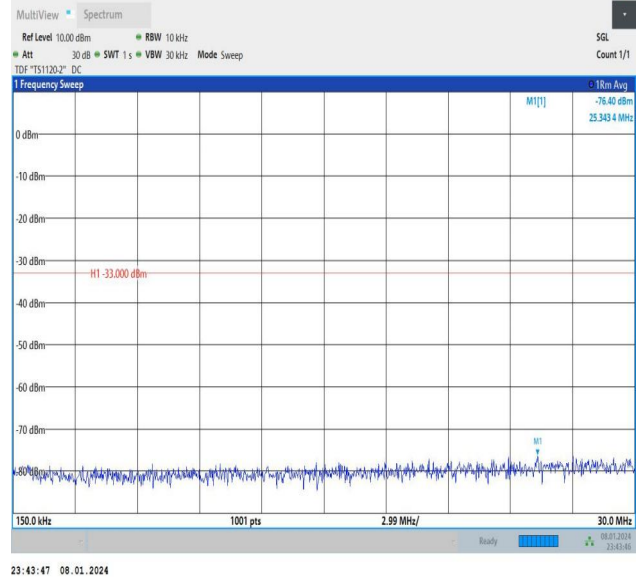
Band4_10MHz_QPSK_20175_1RB#49_0.15~30_0.15~30
