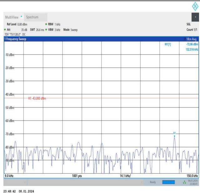
Band4_10MHz_QPSK_20175_50RB#0_0.009~0.15_0.009~0.15
