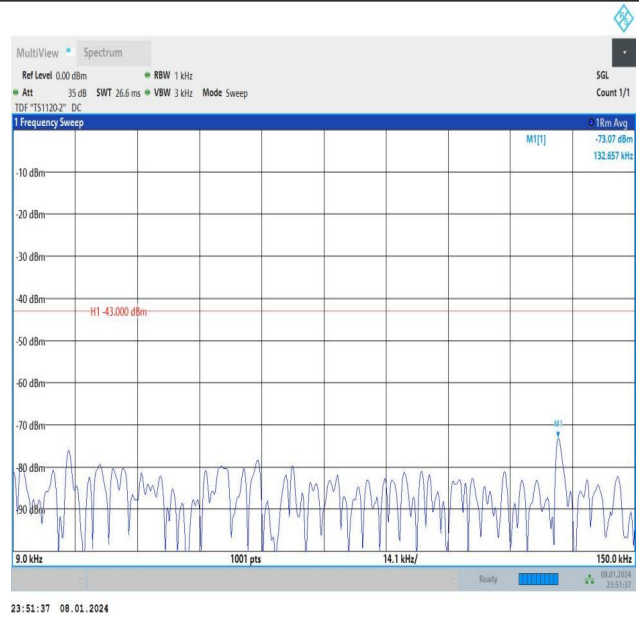
Band4_15MHz_QPSK_20025_1RB#74_0.009~0.15_0.009~0.15
