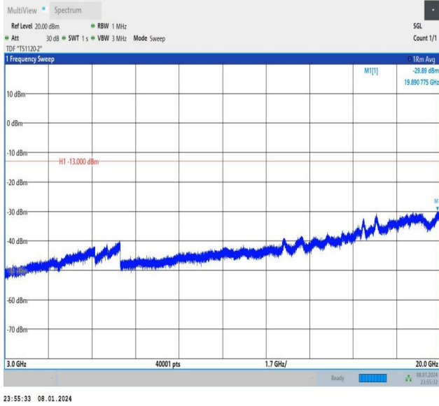
Band4_15MHz_16QAM_20175_1RB#74_3000~20000_3000~20000
