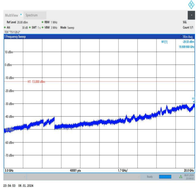
Band4_15MHz_QPSK_20175_1RB#74_3000~20000_3000~2 0000
