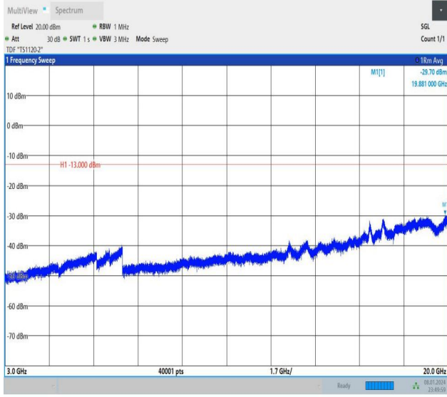
Band4_10MHz_QPSK_20350_50RB#0_3000~20000_3000~20000
