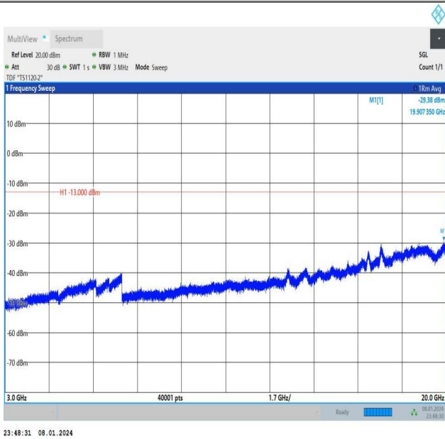
Band4_10MHz_QPSK_20000_50RB#0_3000~20000_3000~20000
