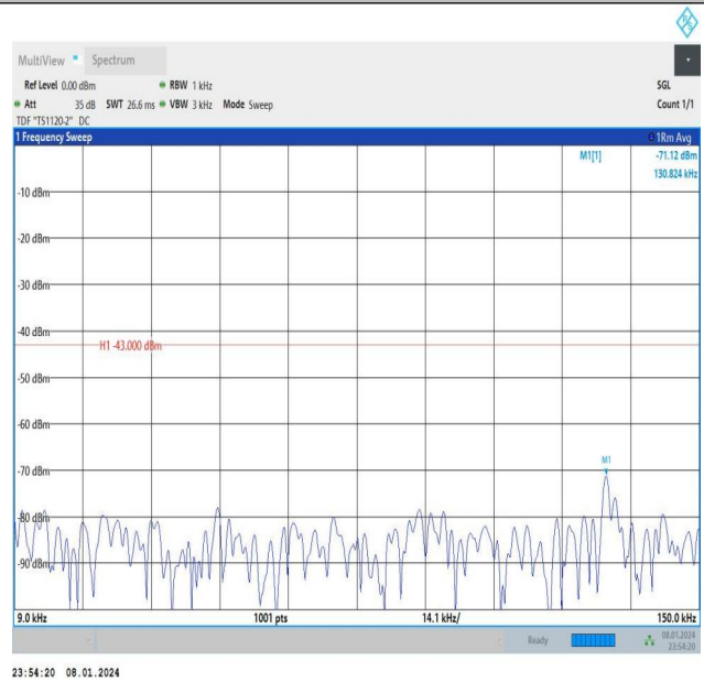
Band4_15MHz_QPSK_20175_1RB#74_0.009~0.15_0.009~0.15
