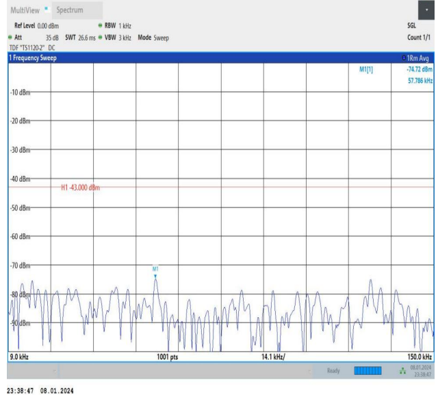
Band4_5MHz_16QAM_20375_25RB#0_0.009~0.15_0.009~0.15
