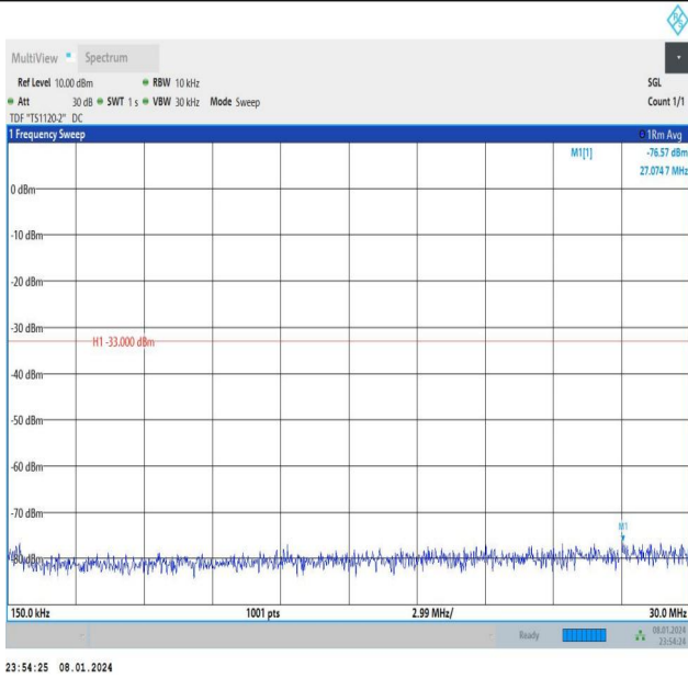
Band4_15MHz_QPSK_20175_1RB#74_0.15~30_0.15~30
