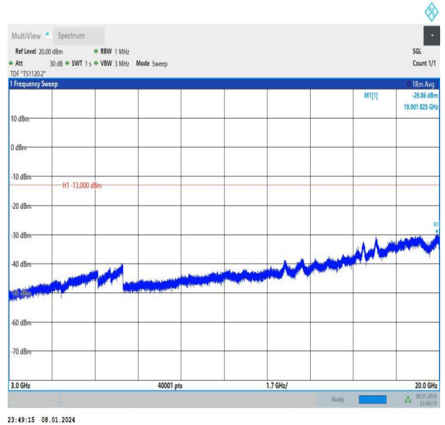
Band4_10MHz_QPSK_20175_50RB#0_3000~20000_3000~2 0000
