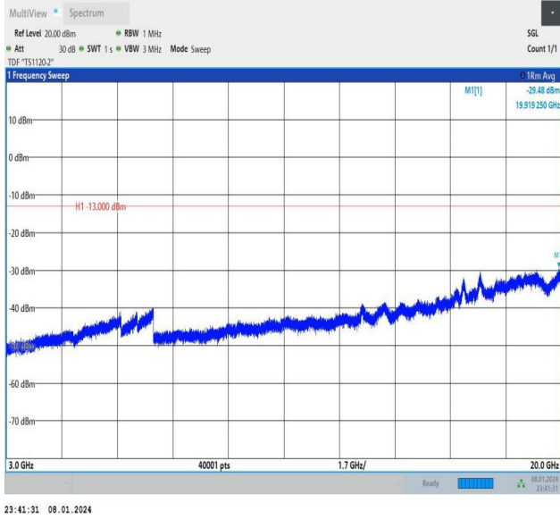
Band4_10MHz_QPSK_20000_1RB#49_3000~20000_3000~20000
