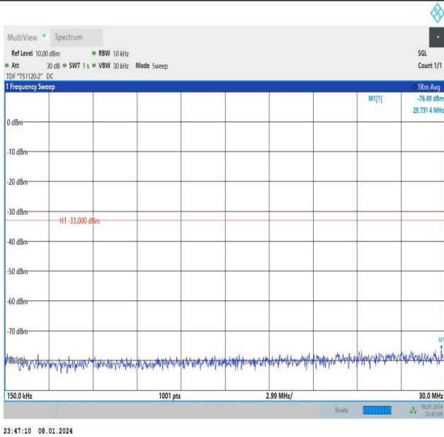
Band4_10MHz_16QAM_20350_1RB#49_0.15~30_0.15~30
