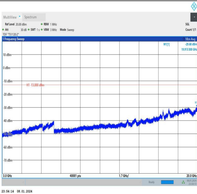
Band4_15MHz_16QAM_20175_1RB#0_3000~20000_3000~20000
