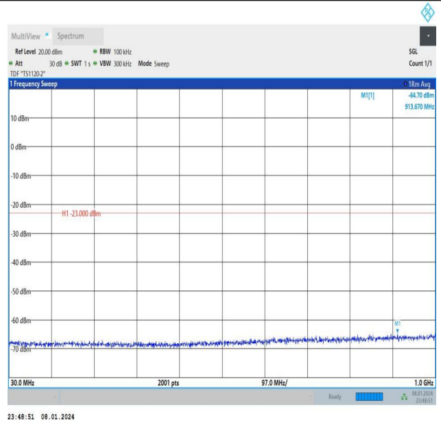
Band4_10MHz_QPSK_20175_50RB#0_30~1000_30~1000
