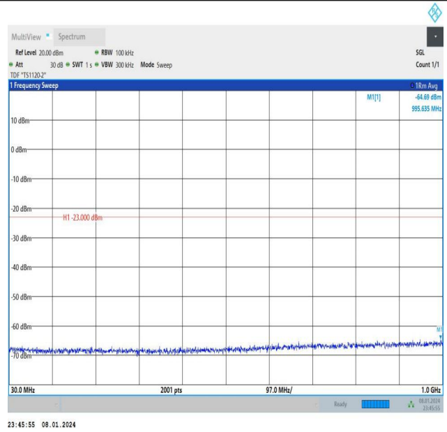
Band4_10MHz_16QAM_20350_1RB#0_30~1000_30~1000
