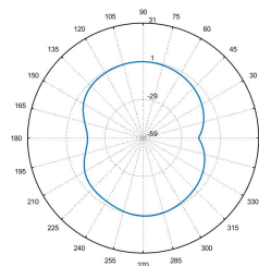
Total_Polar_E1_2.5GHz
