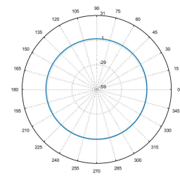
Total_3D_H_2.5GHz
