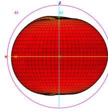
Total_3D_E1_2.5GHz
