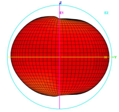
Total_3D_E2_2.5GHz
