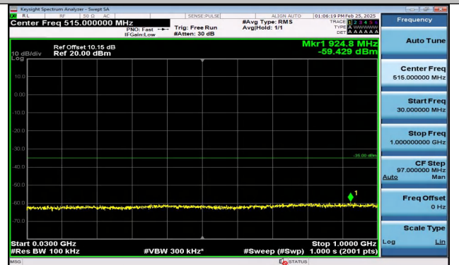
Band41_5MHz_QPSK_39675_1RB#24_30~1000_30~1000
