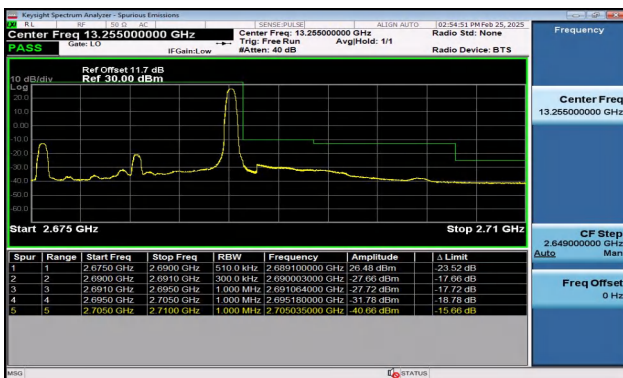
Band41_15MHz_QPSK_41515_1RB#74
