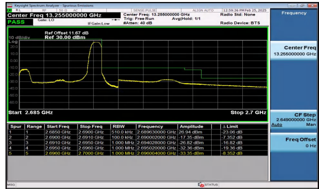
Band41_5MHz_QPSK_41565_1RB#24
