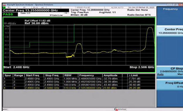
Band41_10MHz_16QAM_39700_1RB#49
