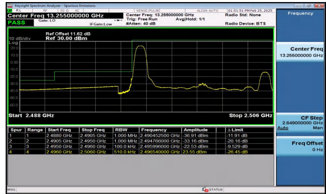
Band41_10MHz_16QAM_39700_1RB#0
