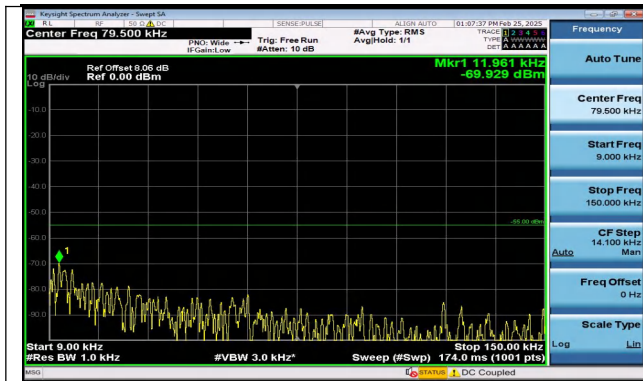
Band41_5MHz_QPSK_39675_25RB#0_0.009~0.15_0.009 ~0.15
