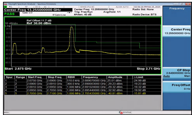
Band41_15MHz_16QAM_41515_1RB#74
