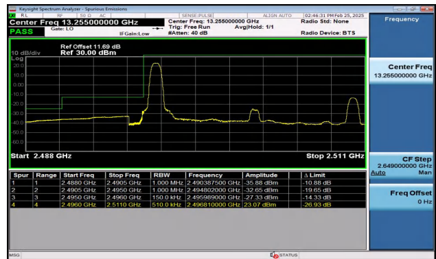
Band41_15MHz_16QAM_39725_1RB#0
