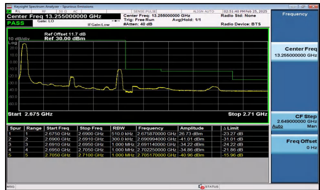
Band41_15MHz_QPSK_41515_1RB#0
