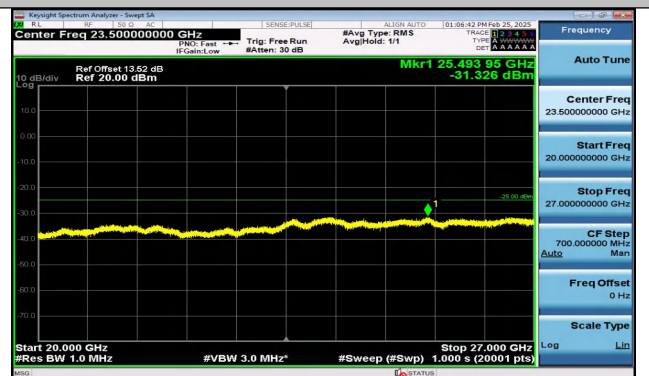
Band41_5MHz_QPSK_39675_1RB#24_20000~27000_20000~27000
