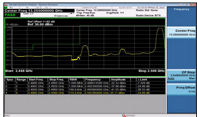
Band41_10MHz_QPSK_39700_1RB#49
