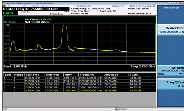
Band41_10MHz_QPSK_41540_1RB#49
