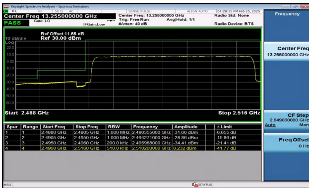
Band41_20MHz_QPSK_39750_100RB#0
