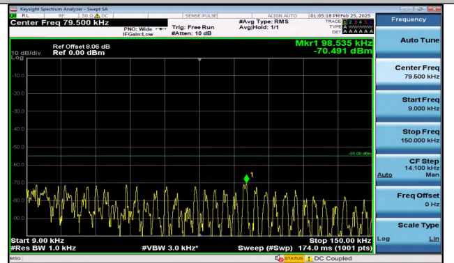
Band41_5MHz_16QAM_39675_1RB#0_0.009~0.15_0.009 ~0.15
