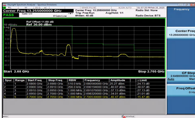
Band41_10MHz_16QAM_41540_1RB#0
