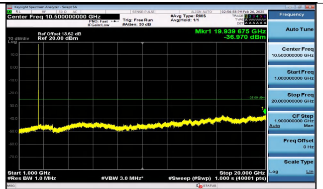
Band41_5MHz_QPSK_39675_1RB#0_1000~20000_1000~20000
