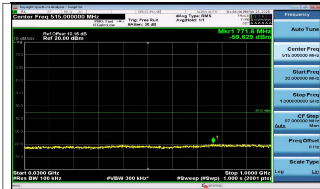
Band41_5MHz_QPSK_39675_1RB#0_30~1000_30~1000
