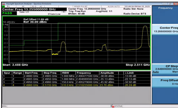
Band41_15MHz_16QAM_39725_1RB#74
