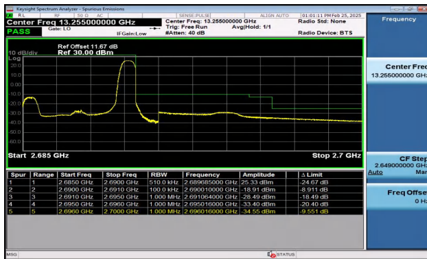
Band41_5MHz_16QAM_41565_1RB#24
