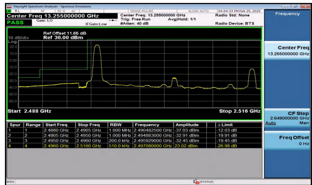
Band41_20MHz_16QAM_39750_1RB#0
