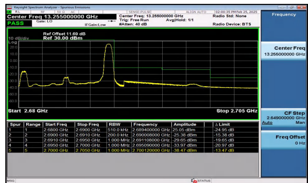
Band41_10MHz_16QAM_41540_1RB#49
