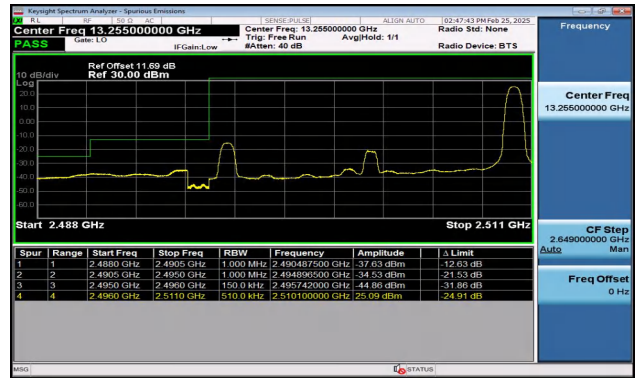
Band41_15MHz_QPSK_39725_1RB#74
