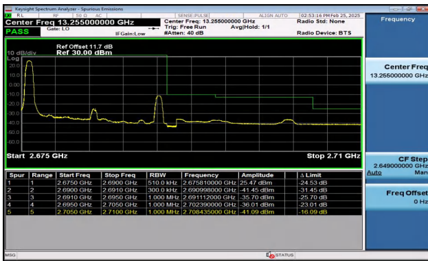
Band41_15MHz_16QAM_41515_1RB#0
