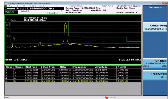
Band41_20MHz_16QAM_41490_1RB#99
