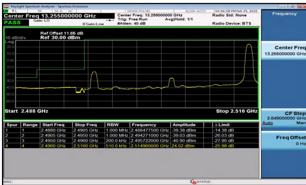
Band41_20MHz_16QAM_39750_1RB#99
