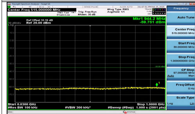
Band41_5MHz_QPSK_39675_25RB#0_30~1000_30~100 0
