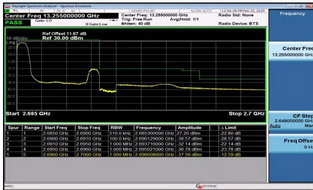
Band41_5MHz_QPSK_41565_1RB#0
