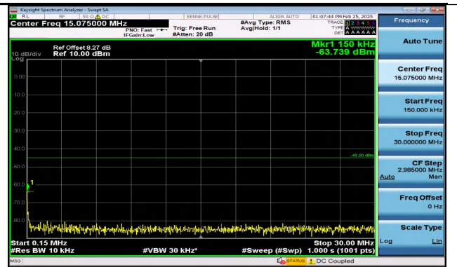
Band41_5MHz_QPSK_39675_25RB#0_0.15~30_0.15~30
