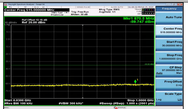
Band41_5MHz_16QAM_39675_1RB#0_30~1000_30~100 0
