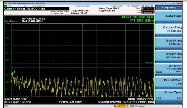
Band41_5MHz_QPSK_39675_1RB#24_0.009~0.15_0.009~0.15
