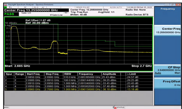
Band41_5MHz_16QAM_41565_1RB#0
