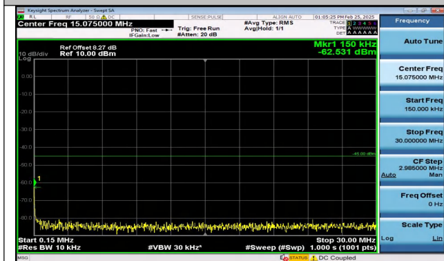
Band41_5MHz_16QAM_39675_1RB#0_0.15~30_0.15~30 0
