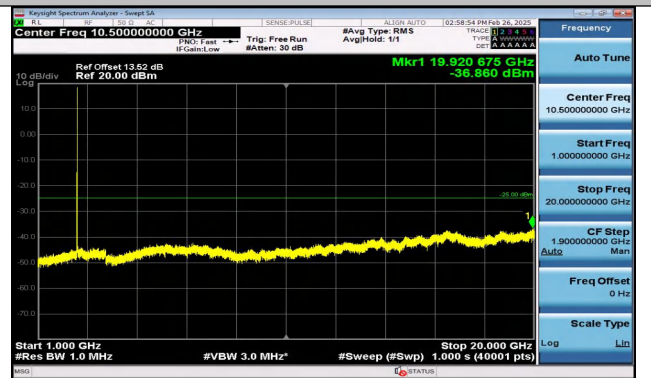
Band41_5MHz_QPSK_39675_25RB#0_1000~20000_100 0~20000
