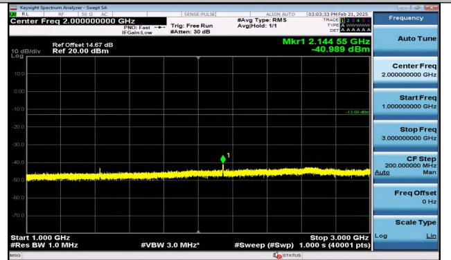
Band12_3MHz_QPSK_23165_15RB#0_1000~3000_1000~3000 ~3000
