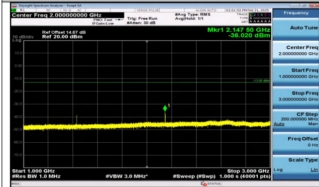
Band12_3MHz_QPSK_23165_1RB#14_1000~3000_1000~3000
