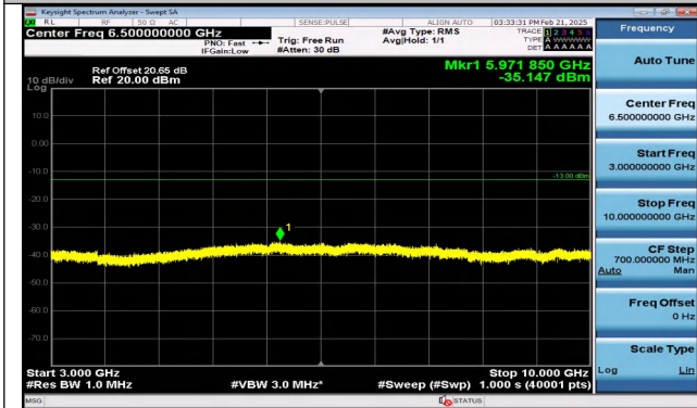
Band12_5MHz_QPSK_23035_1RB#0_3000~10000_3000~10000
