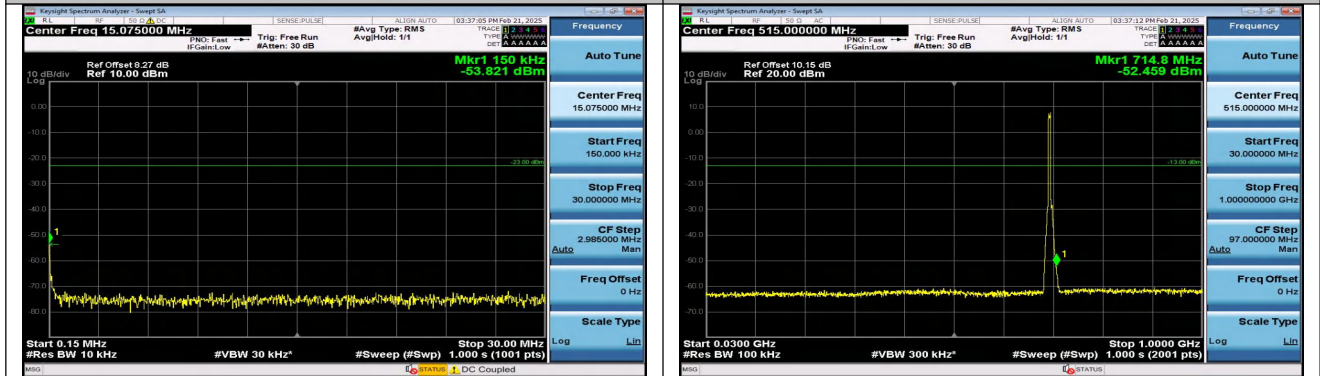
Band12_5MHz_16QAM_23035_25RB#0_0.15~30_0.15~30
