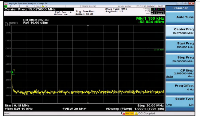
Band12_5MHz_QPSK_23035_1RB#0_0.15~30_0.15~30
