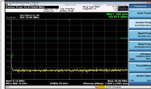
Band12_3MHz_QPSK_23165_1RB#14_0.15~30_0.15~30
