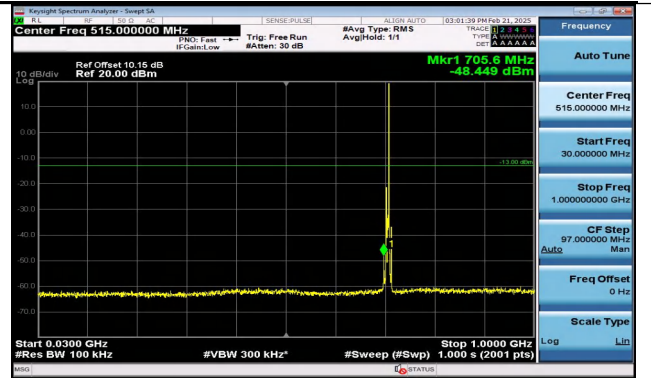
Band12_3MHz_QPSK_23165_1RB#14_30~1000_30~100 0
