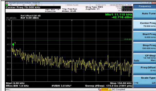
Band12_3MHz_QPSK_23165_15RB#0_0.009~0.15_0.009~0.15
