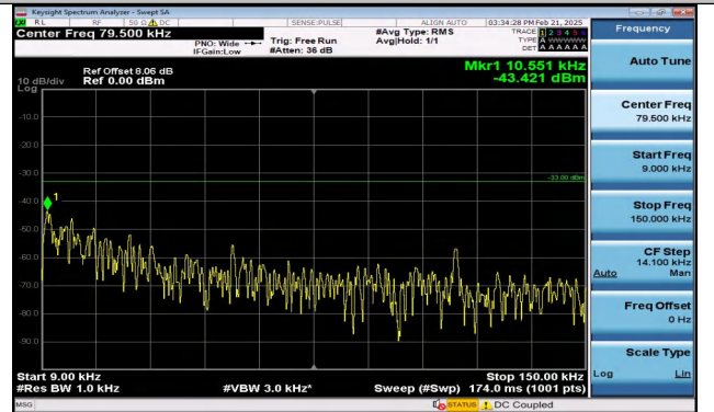
Band12_5MHz_QPSK_23035_1RB#24_0.009~0.15_0.009~0.15
