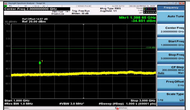
Band12_5MHz_QPSK_23035_1RB#0_1000~3000_1000~3000
