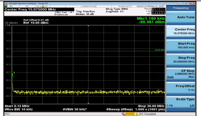
Band12_3MHz_QPSK_23165_15RB#0_0.15~30_0.15~30
