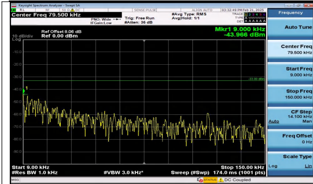
Band12_5MHz_QPSK_23035_1RB#0_0.009~0.15_0.009~0.15
