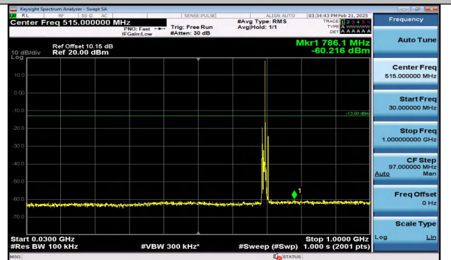
Band12_5MHz_QPSK_23035_1RB#24_30~1000_30~1000
