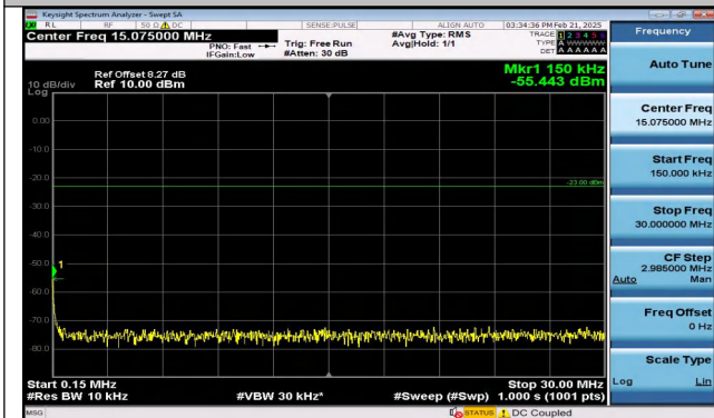
Band12_5MHz_QPSK_23035_1RB#24_0.15~30_0.15~30
