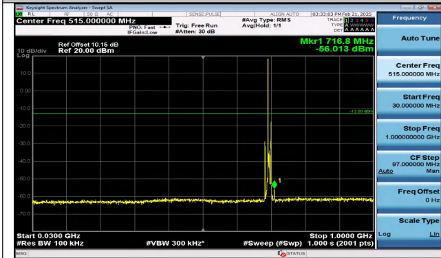
Band12_5MHz_QPSK_23035_1RB#0_30~1000_30~1000
