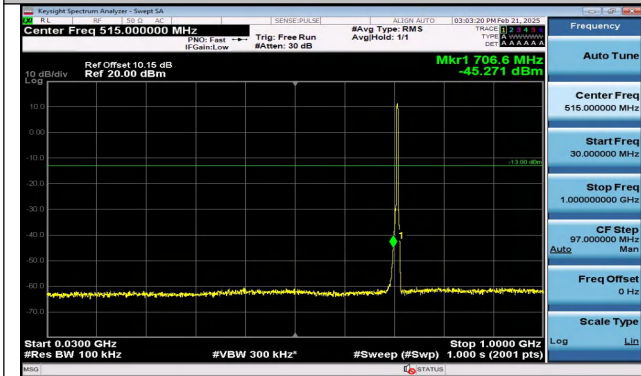
Band12_3MHz_QPSK_23165_15RB#0_30~1000_30~1000 0
