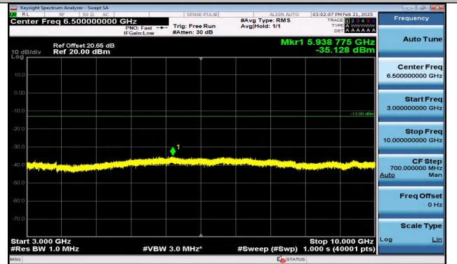
Band12_3MHz_QPSK_23165_1RB#14_3000~10000_3000~10000 0~10000
