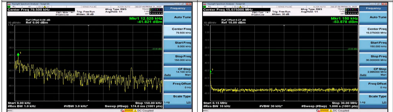
Band12_5MHz_QPSK_23095_1RB#0_0.009~0.15_0.009~0.15
