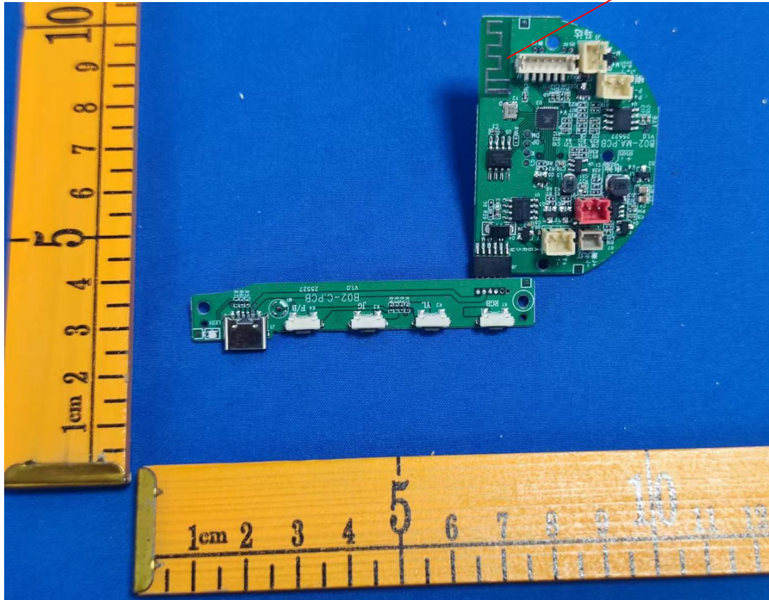
EUT Internal View 5
