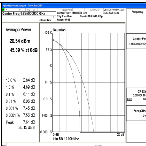
Band25-10MHz-16QAM-26090-50RB#0-PASS
