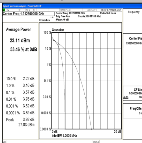
Band25-5MHz-QPSK-26665-1RB#0-PASS
