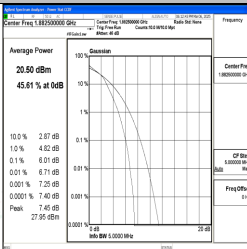
Band25-3MHz-16QAM-26365-15RB#0-PASS
