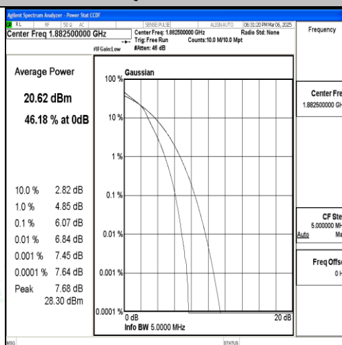
Band25-5MHz-16QAM-26365-25RB#0-PASS
