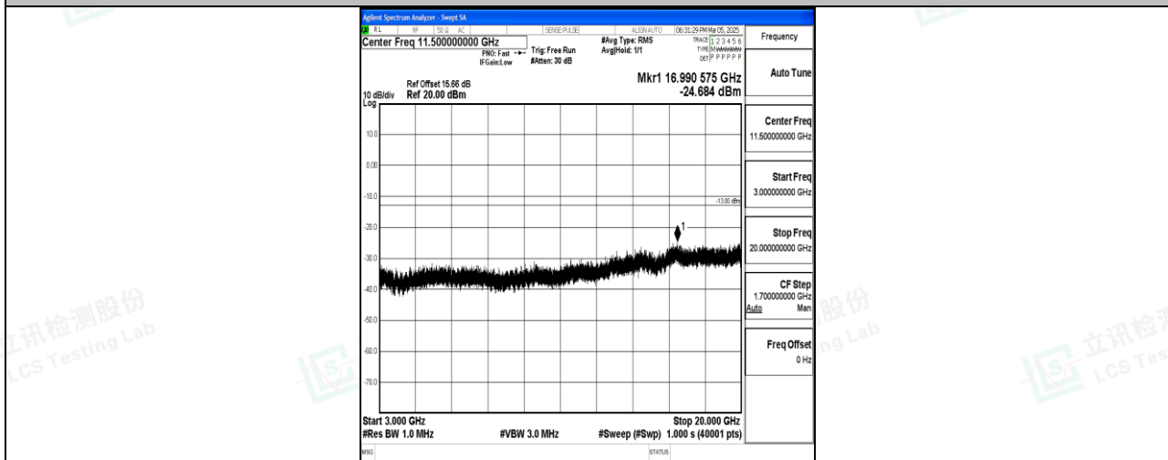
Band2_15MHz_QPSK_18900_1RB#0_3000~20000_3000~20000
