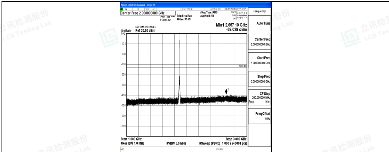
Band2_10MHz_QPSK_18900_1RB#0_1000~3000_1000~3000
