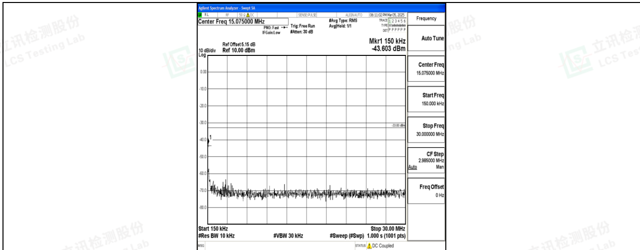
Band2_10MHz_QPSK_18650_1RB#0_0.15~30_0.15~30
