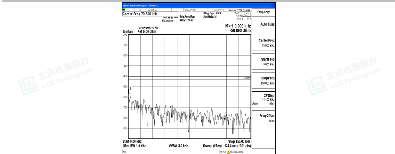
Band2_15MHz_16QAM_18900_1RB#0_0.009~0.15_0.009~0.15
