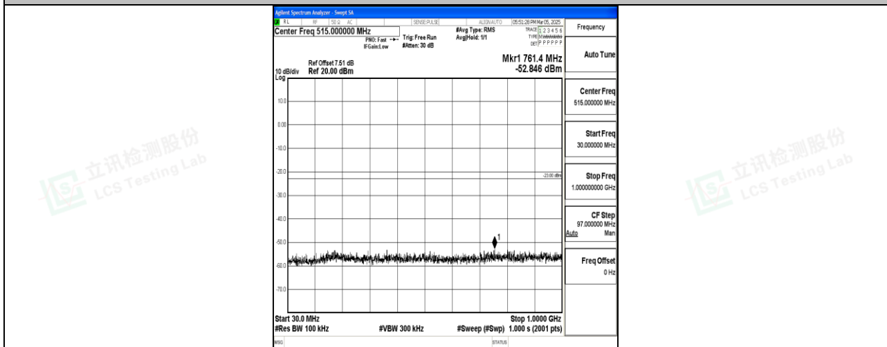
Band2_5MHz_QPSK_18900_1RB#0_30-1000_30-1000
