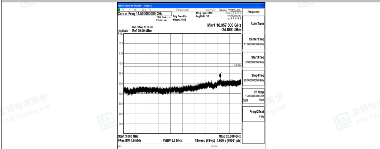
Band2_10MHz_QPSK_18900_1RB#0_3000~20000_3000~20000
