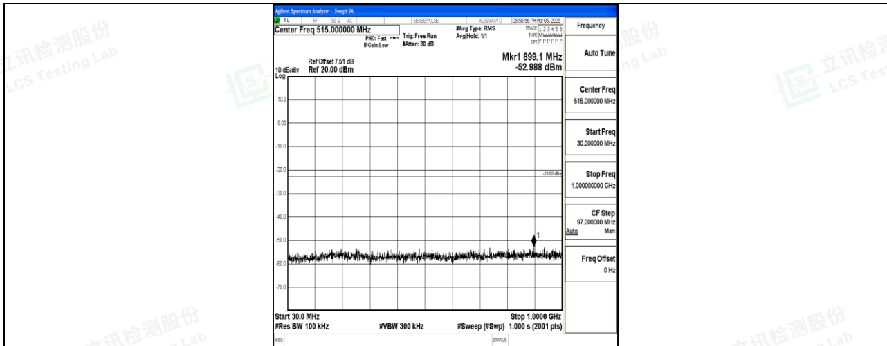
Band2_5MHz_16QAM_18625_1RB#0_30~1000_30~1000
