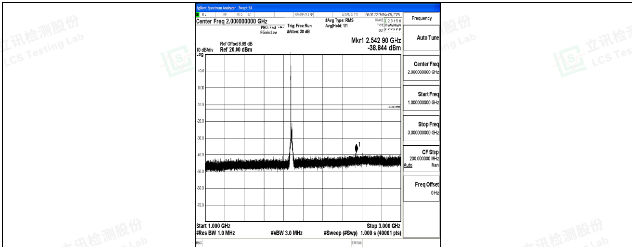
Band2_15MHz_QPSK_18900_1RB#0_1000~3000_1000~3000
