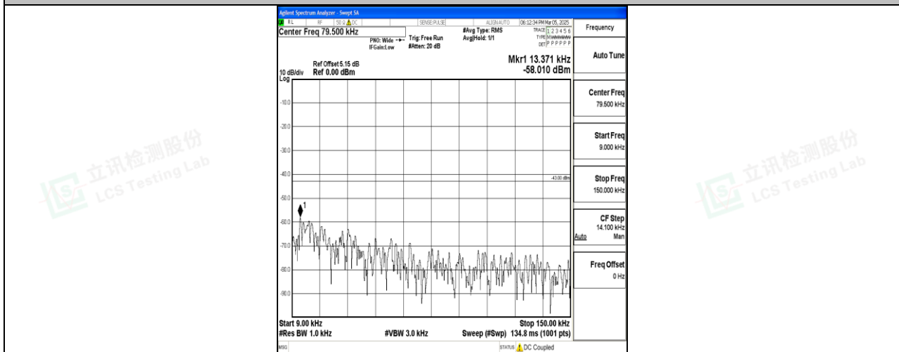
Band2_10MHz_16QAM_18900_1RB#0_0.009~0.15_0.009~0.15
