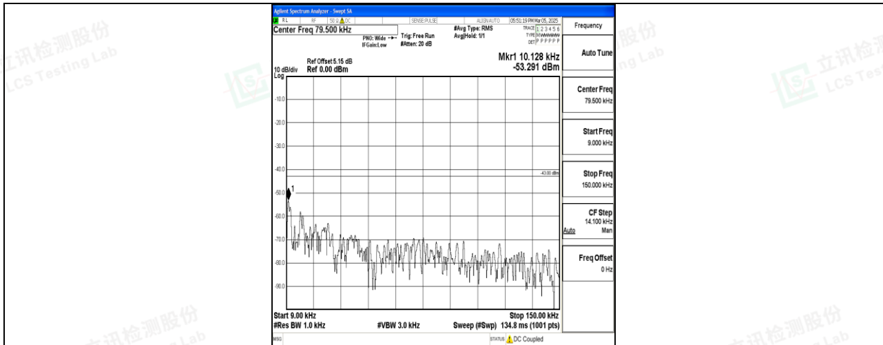
Band2_5MHz_QPSK_18900_1RB#0_0.009-0.15_0.009-0.15
