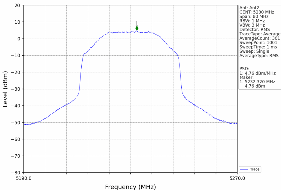
40M_HCH_5230MHz_Ant2_NTNV
