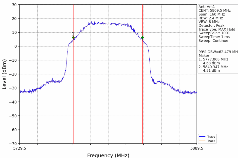
80M_HCH_5809.5MHz_Ant1_NTNV
