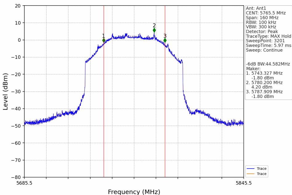
80M_LCH_5765.5MHz_Ant1_NTN
