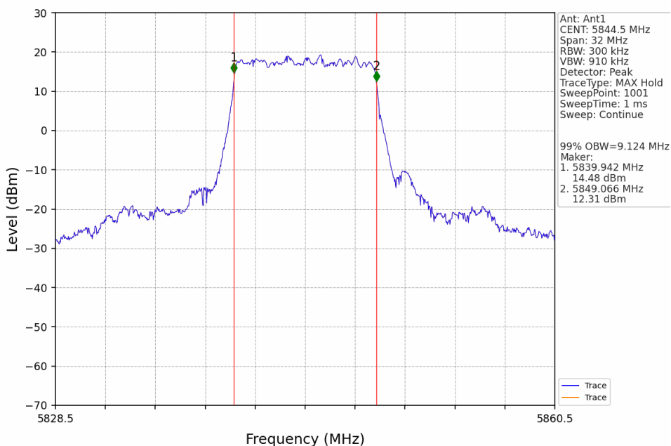
10M_HCH_5844.5MHz_Ant1_NTNV
