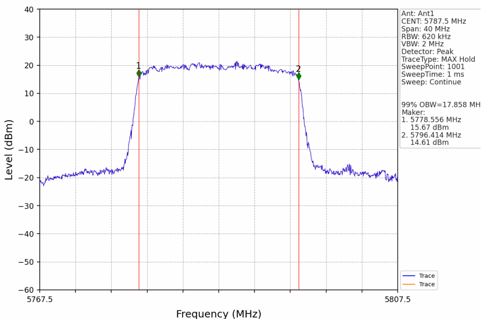
20M_MCH_5787.5MHz_Ant1_NTNV
