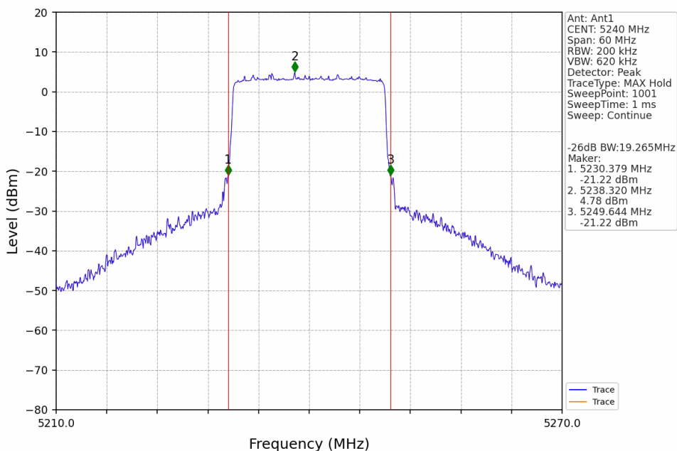
20M_HCH_5240MHz_Ant1_NTNV
