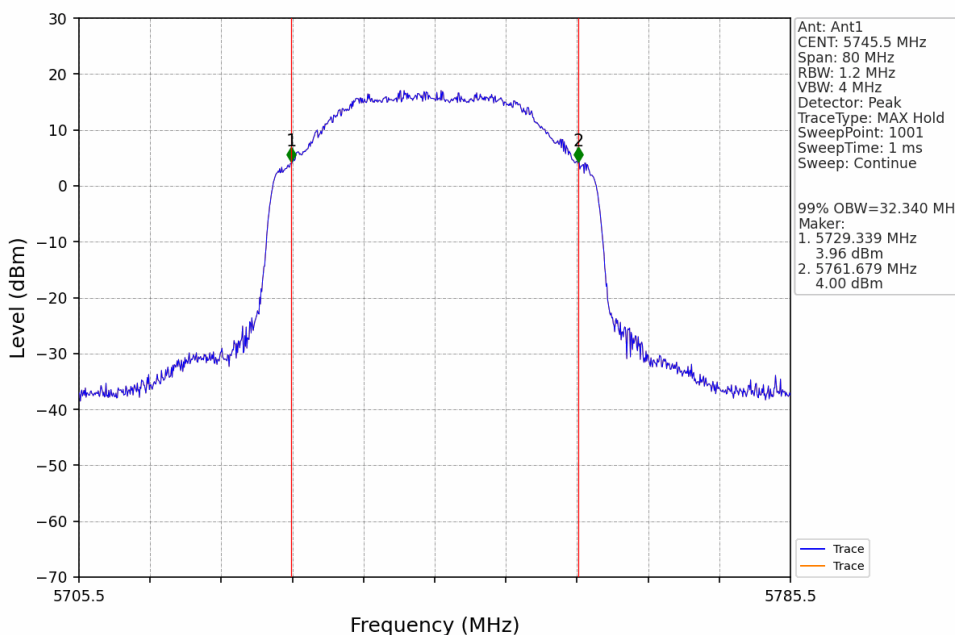
40M_LCH_5745.5MHz_Ant1_NTNV
