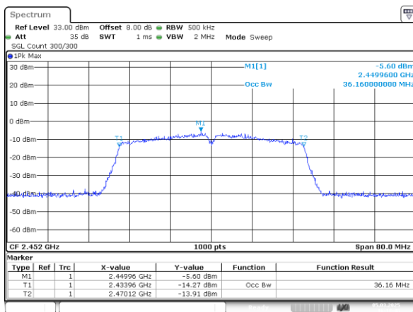
802.11n40_2452MHz_Chain 0
