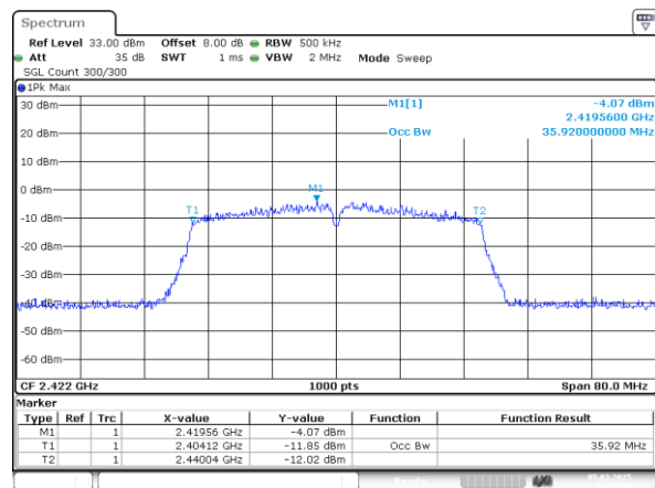
802.11n40_2422MHz_Chain 1
