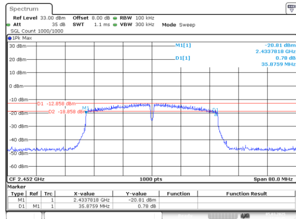
802.11n40_2452MHz_Chain 1
