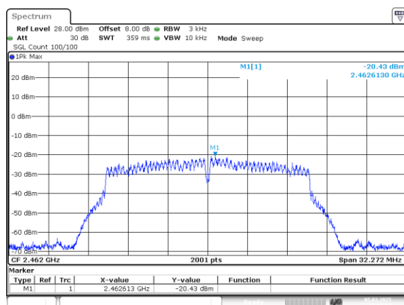
802.11g_2462MHz_Chain 0
