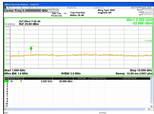
1000.0MHz-10000.0MHz Band 13 10MHz/782.0/High QPSK 1@0
