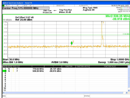
30.0MHz-1000.0MHz Band 13 10MHz/782.0/Low QPSK 1@0
