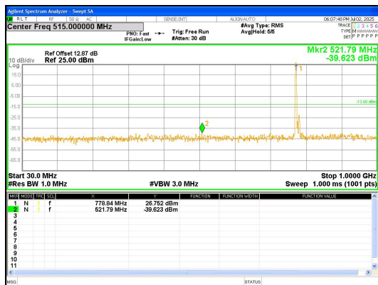
30.0MHz-1000.0MHz Band 13 10MHz/782.0/High QPSK 1@0
