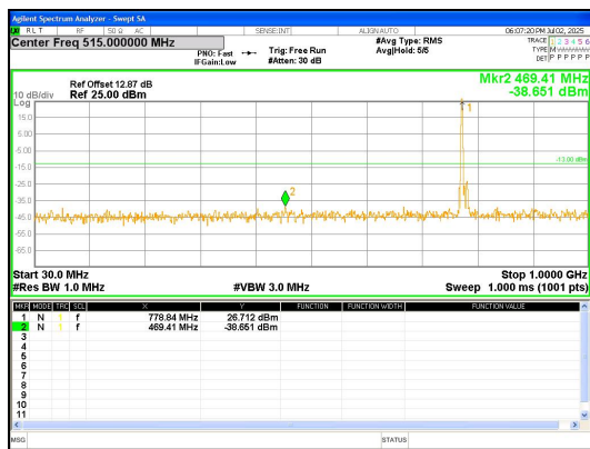
30.0MHz-1000.0MHz Band 13 10MHz/782.0/Mid QPSK 1@0
