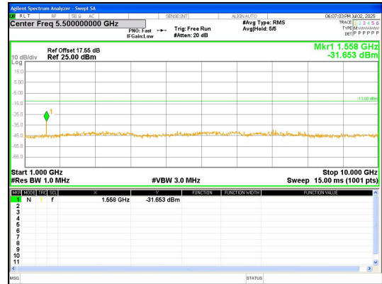
1000.0MHz-10000.0MHz Band 13 10MHz/782.0/Low QPSK 1@0
