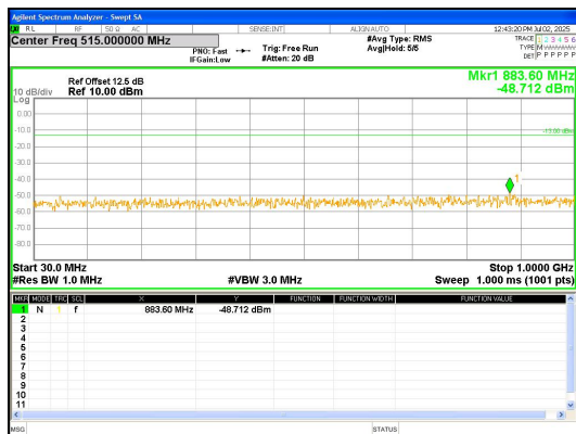
30.0MHz-1000.0MHz Band 4 10MHz/1750.0/High QPSK 1@0
