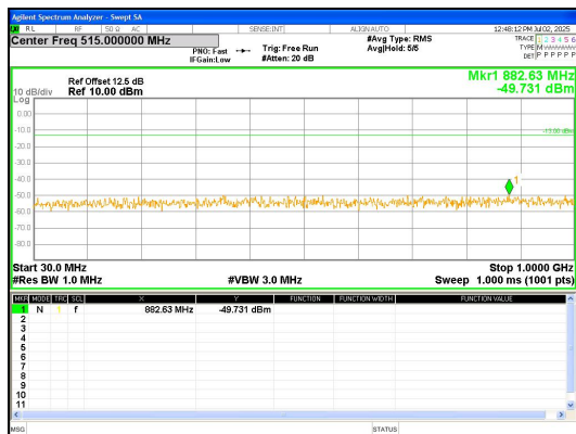
30.0MHz-1000.0MHz Band 4 20MHz/1745.0/High QPSK 1@0
