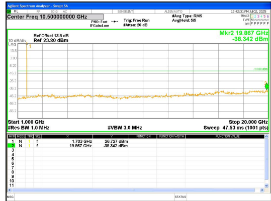
1000.0MHz-20000.0MHz Band 4 10MHz/1715.0/Low QPSK 1@0
