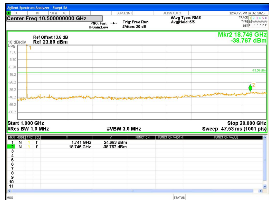
1000.0MHz-20000.0MHz Band 4 20MHz/1745.0/High QPSK 1@0
