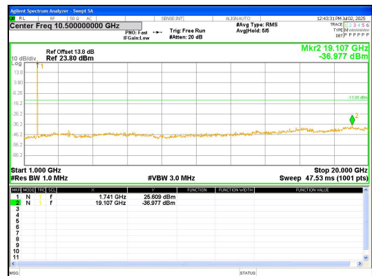
1000.0MHz-20000.0MHz Band 4 10MHz/1750.0/High QPSK 1@0
