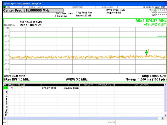
30.0MHz-1000.0MHz Band 4 20MHz/1720.0/Low QPSK 1@0
