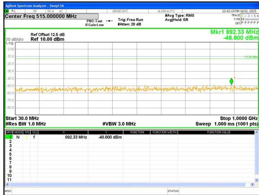
30.0MHz-1000.0MHz Band 4 10MHz/1715.0/Low QPSK 1@0
