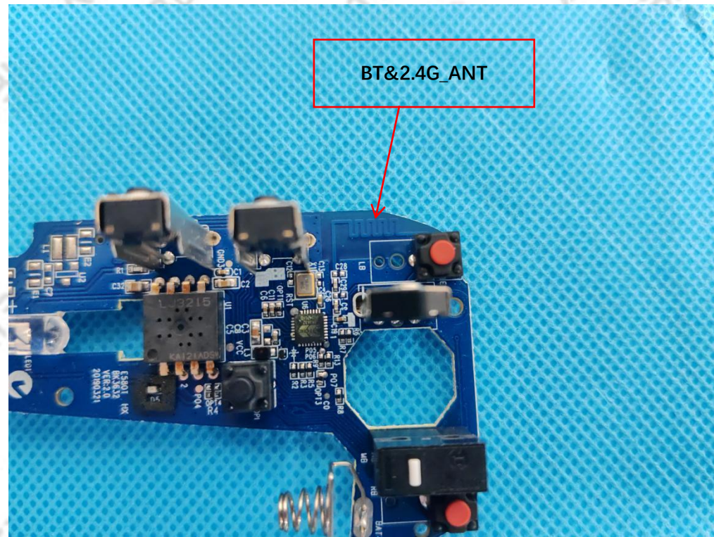
OPEN VIEW OF EUT(Figure 7)
