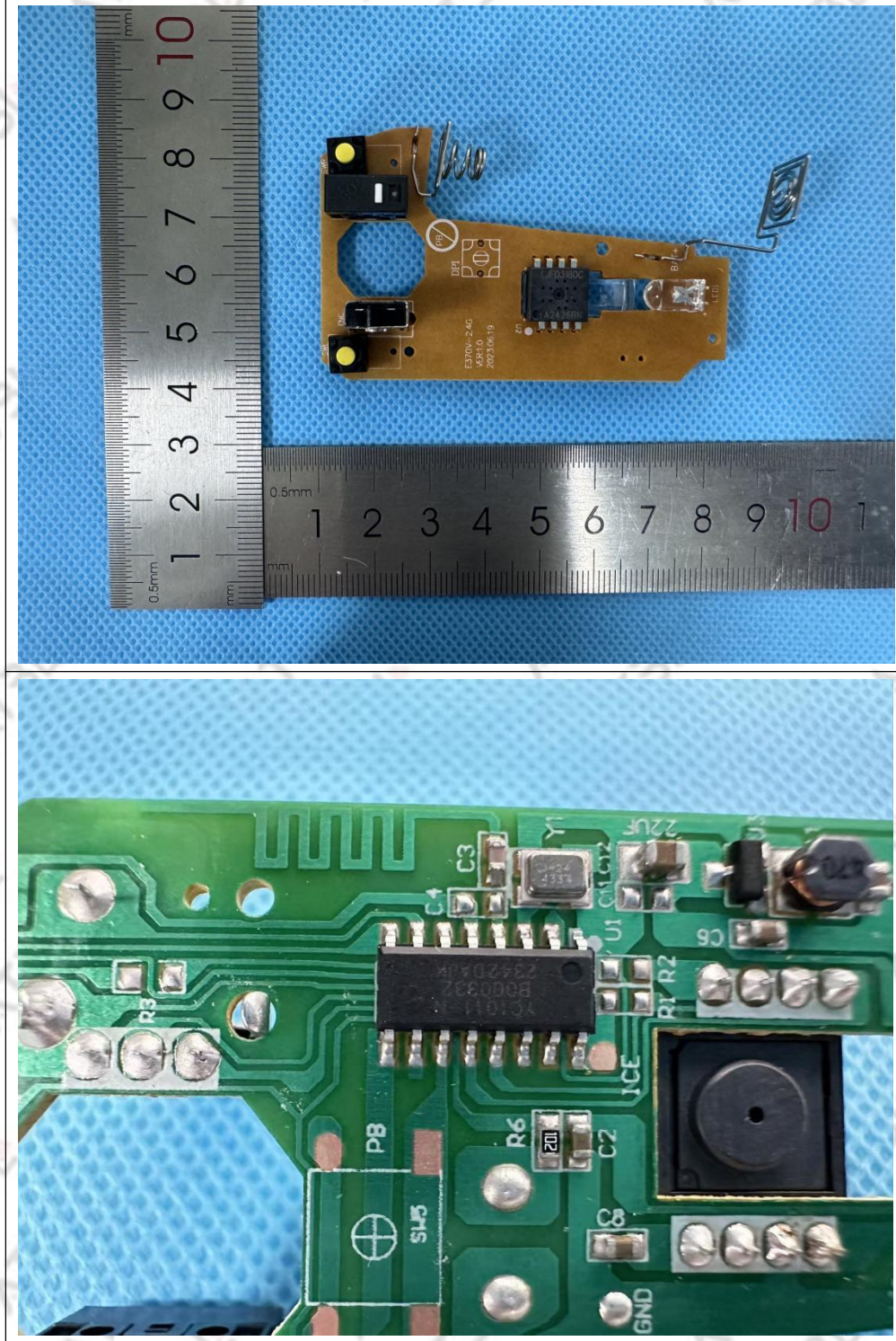
OPEN VIEW OF EUT(FIGURE 5)
