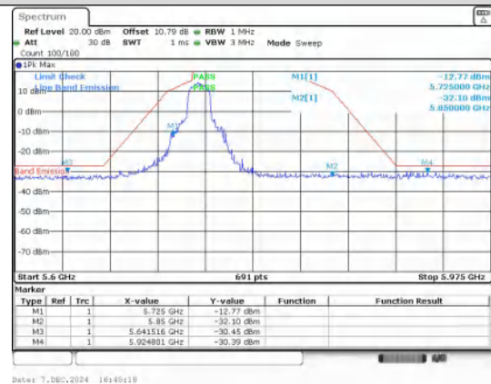
Out Of Band Emission IEEE 802.11ac_Channel 149_20MHz_Antenna 1
