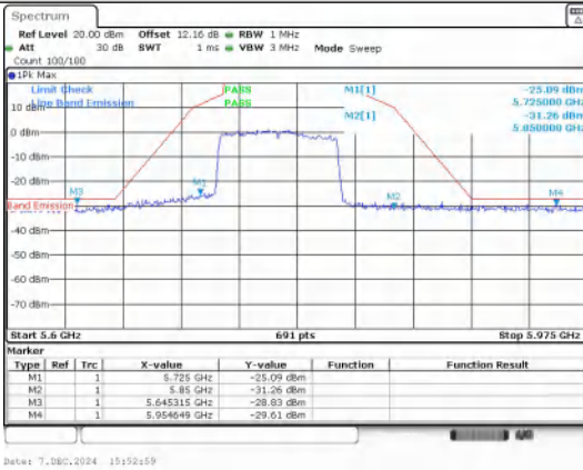
Out Of Band Emission IEEE 802.11ac_Channel 155_80MHz_Antenna 0
