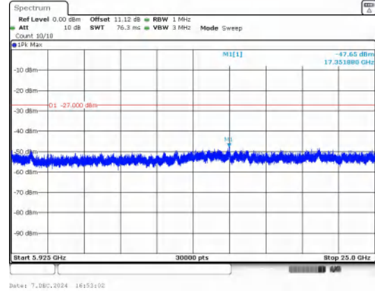
Spurious Emission:5925~25000.0 MHz IEEE 802.11ac_Channel 157_20MHz_Antenna 1
