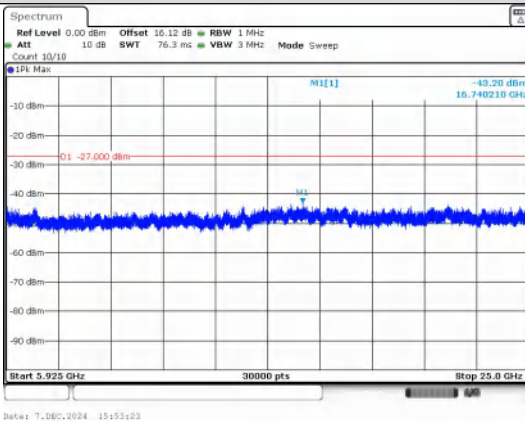
Spurious Emission:5925~25000.0 MHz IEEE 802.11ac_Channel 155_80MHz_Antenna 0
