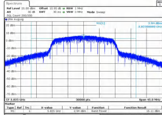
Conducted AVG output power IEEE 802.11ac_20_Channel 165_Antenna 1
