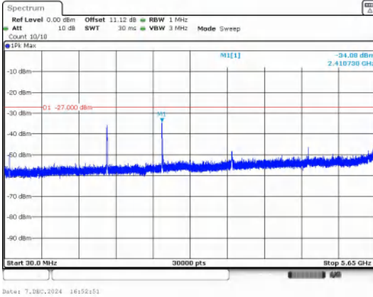
Spurious Emission:30.0~5650 MHz IEEE 802.11ac_Channel 157_20MHz_Antenna 1
