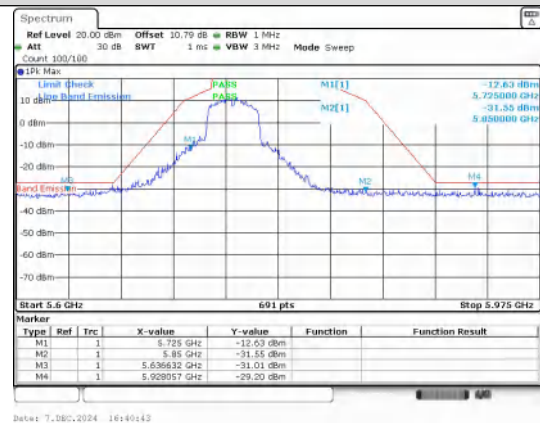
Out Of Band Emission IEEE 802.11n_Channel 151_40MHz_Antenna 1
