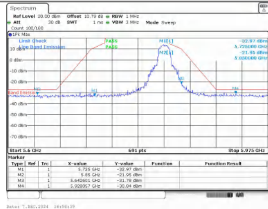
Out Of Band Emission IEEE 802.11ac_Channel 165_20MHz_Antenna 1
