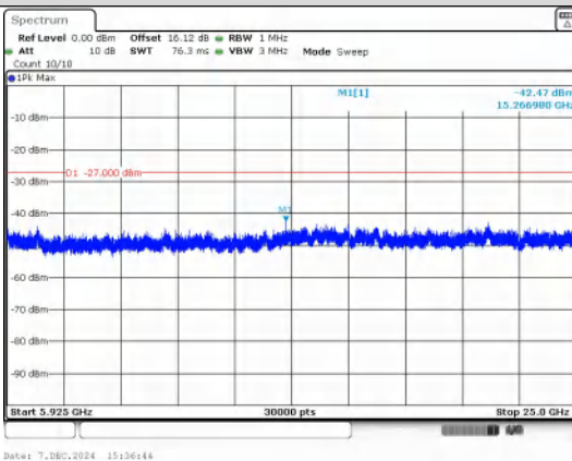
Spurious Emission:5925~25000.0 MHz IEEE 802.11ac_Channel 157_20MHz_Antenna 0
