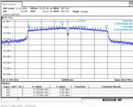
IEEE 802.11n_Channel 159_40MHz_Antenna 0
