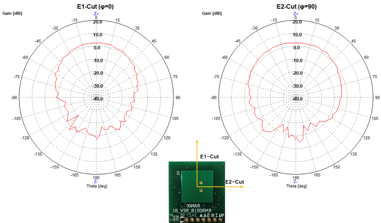
Figure 2. Radiation Pattern
