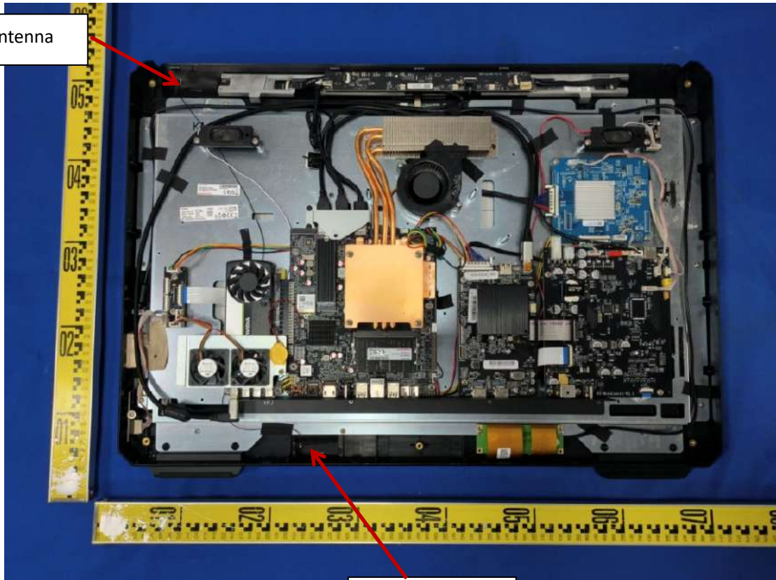
WiFi Antenna
