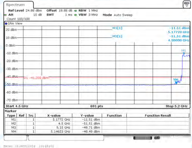
11AX40SISO-Ant1-5190-PASS
