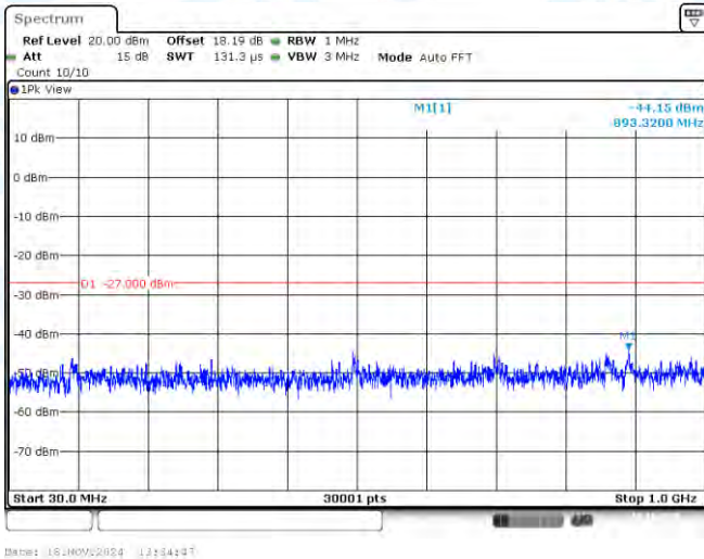
11AC40SISO-Ant1-5795-30~1000-PASS
