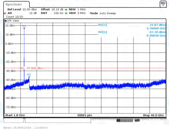
11AC20SISO-Ant1-5785-1000~40000-PASS
