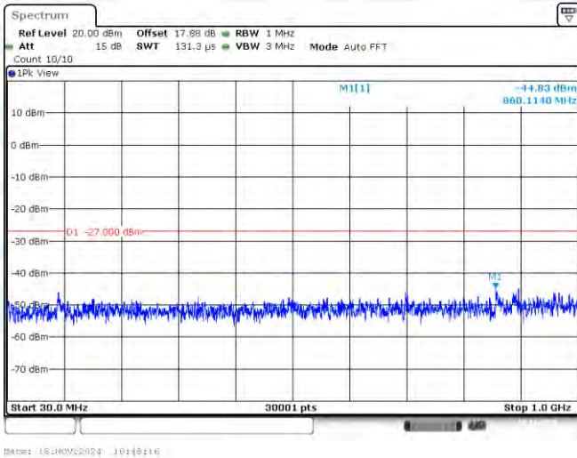
11AX40SISO-Ant1-5190-30~1000-PASS
