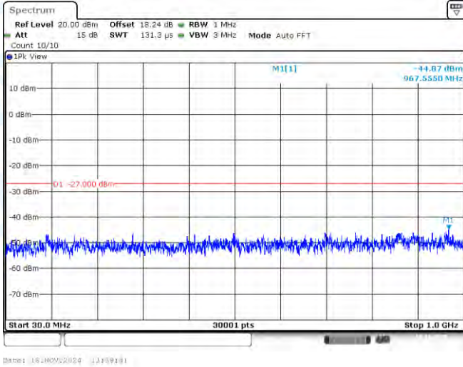
11AX20SISO-Ant1-5825-30~1000-PASS
