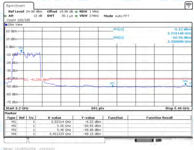
11AX40SISO-Ant1-5230-PASS
