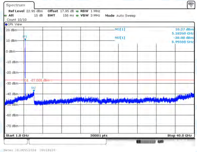
11AC20SISO-Ant1-5180-1000~40000-PASS
