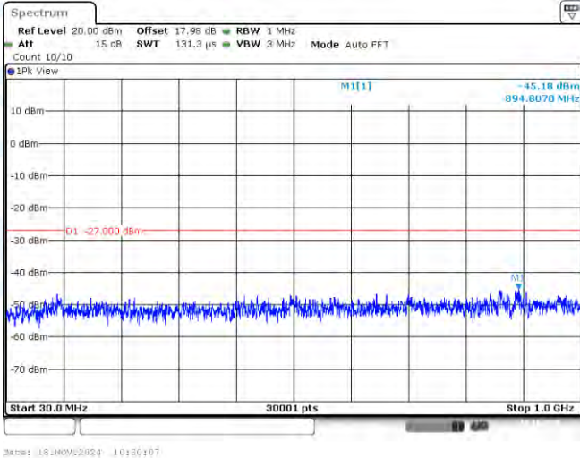
11AX20SISO-Ant1-5240-30~1000-PASS
