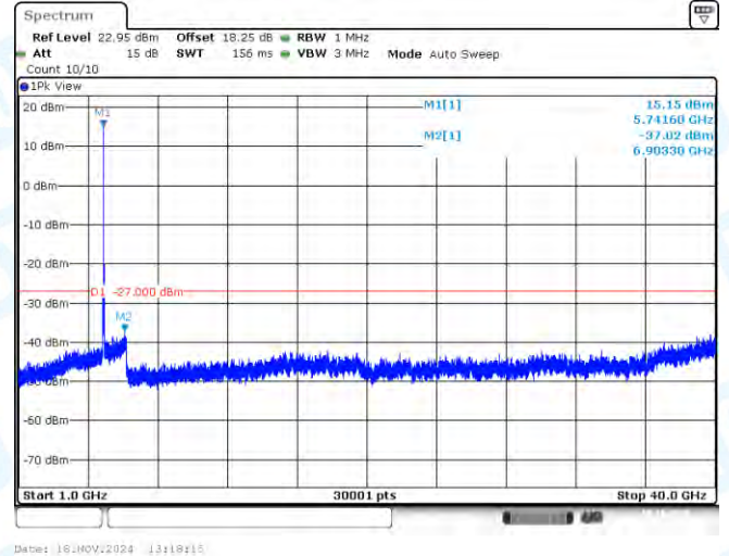
11AC20SISO-Ant1-5745-1000~40000-PASS
