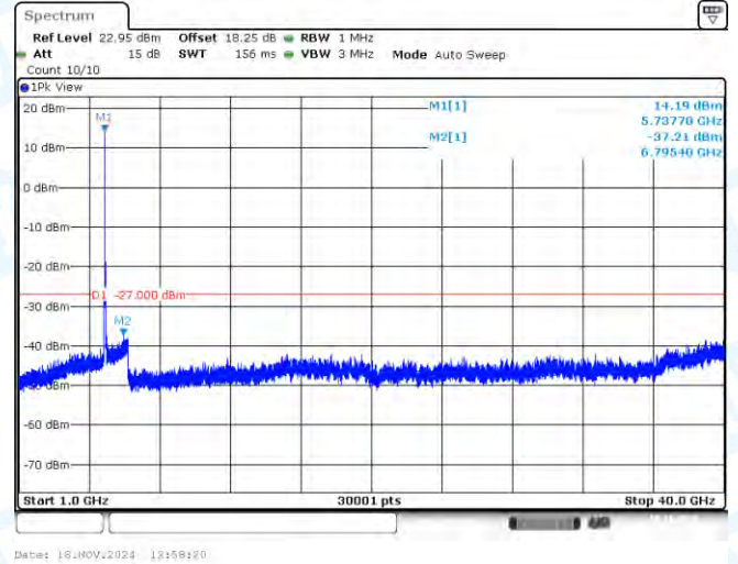
11N20SISO-Ant1-5745-1000~40000-PASS
