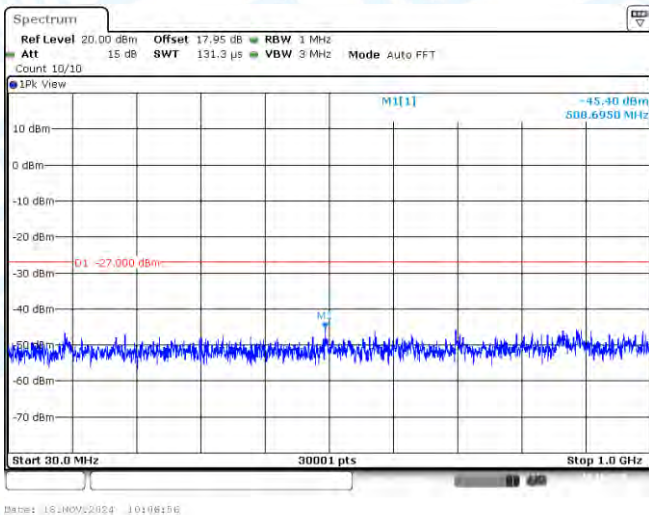
11AX20SISO-Ant1-5180-30~1000-PASS
