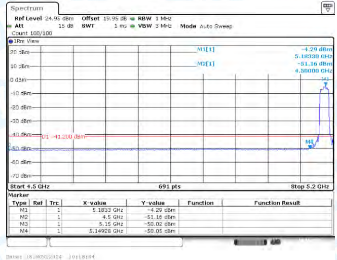
11AX20SISO-Ant1-5180-PASS
