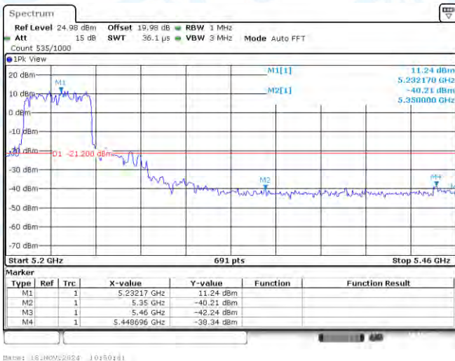
11AX40SISO-Ant1-5230-PASS
