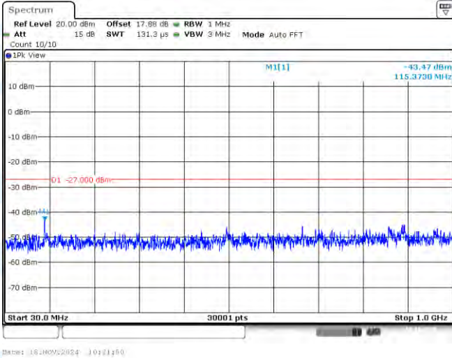
11AX20SISO-Ant1-5200-30~1000-PASS
