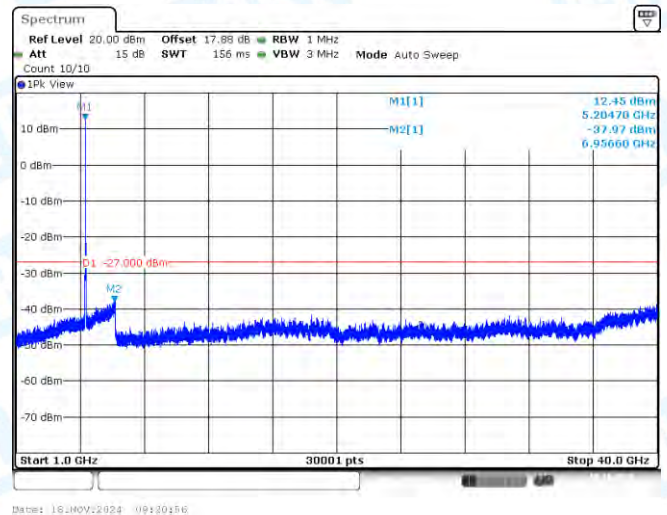
11AC20SISO-Ant1-5200-1000~40000-PASS
