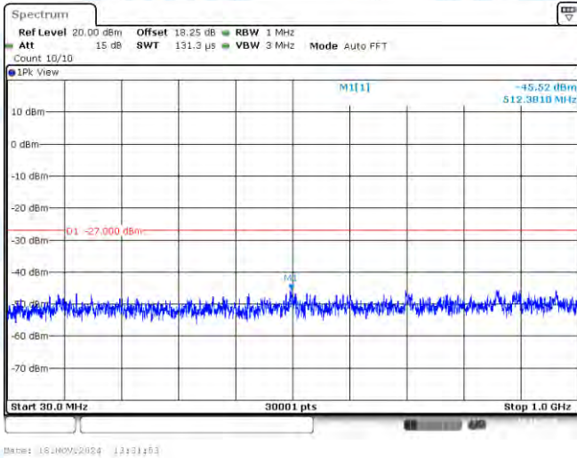
11AC40SISO-Ant1-5755-30~1000-PASS
