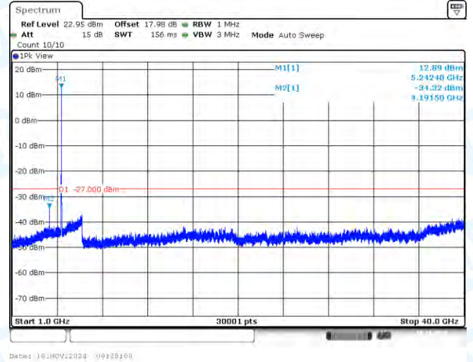
11AC20SISO-Ant1-5240-1000~40000-PASS
