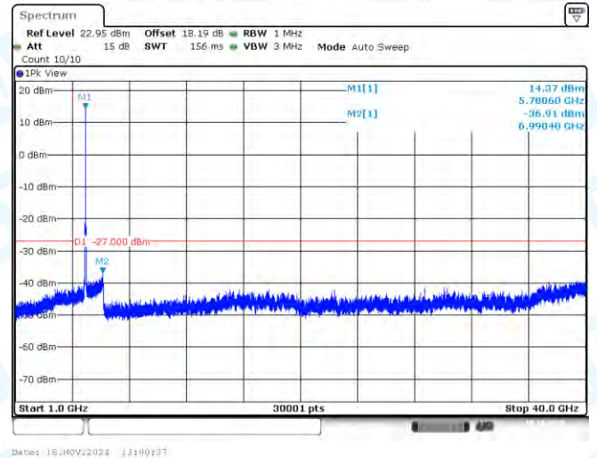
11N20SISO-Ant1-5785-1000~40000-PASS
