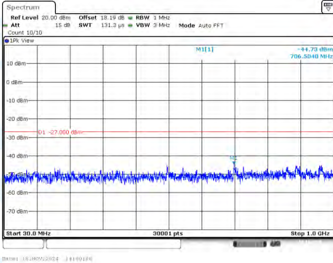
11AX20SISO-Ant1-5785-30~1000-PASS
