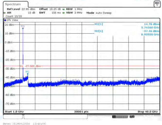
11AX20SISO-Ant1-5745-1000~40000-PASS
