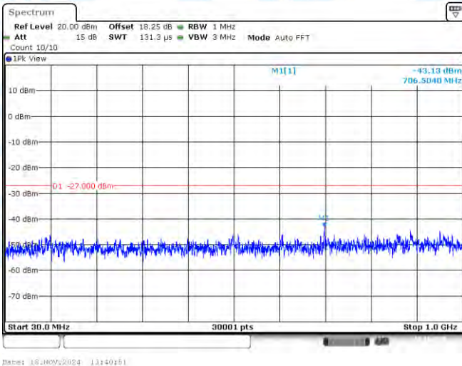
11AX20SISO-Ant1-5745-30~1000-PASS
