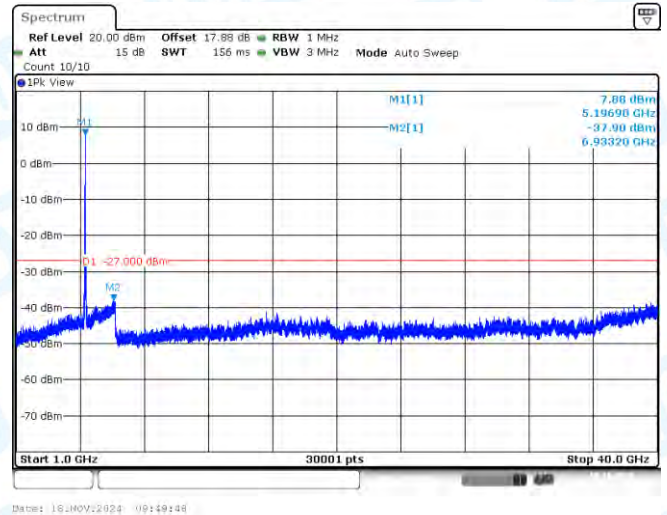
11AC40SISO-Ant1-5190-1000~40000-PASS
