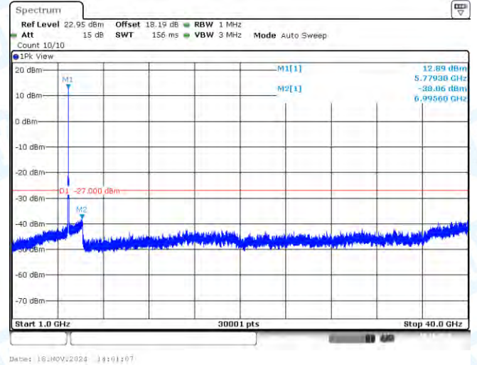
11AX20SISO-Ant1-5785-1000~40000-PASS
