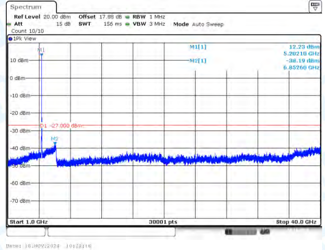
11AX20SISO-Ant1-5200-1000~40000-PASS
