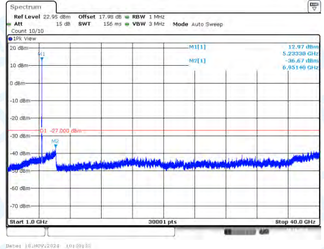
11AX20SISO-Ant1-5240-1000~40000-PASS
