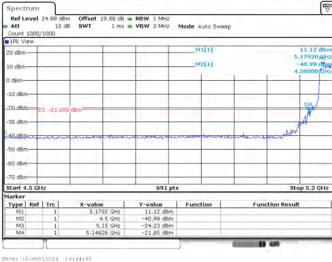
11AX40SISO-Ant1-5190-PASS
