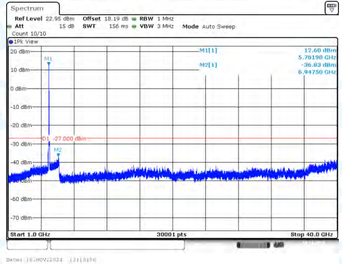
11N40SISO-Ant1-5795-1000~40000-PASS
