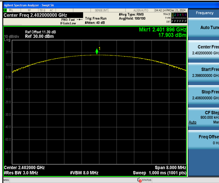
3DH5-Ant4-2402-PASS
