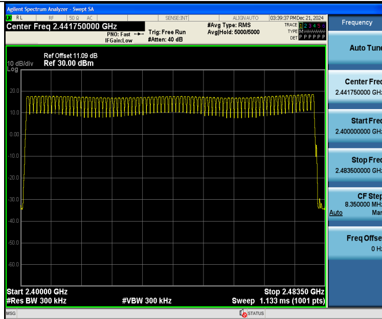
DH5-Ant3-Hop-PASS
