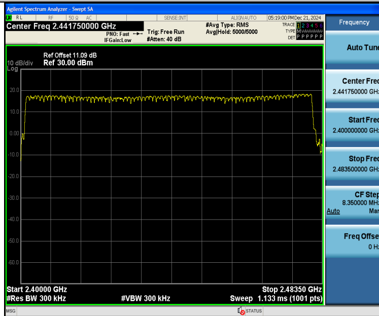
3DH5-Ant4-Hop-PASS
