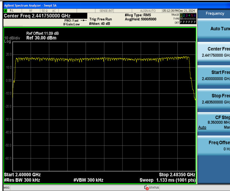
2DH5-Ant4-Hop-PASS
