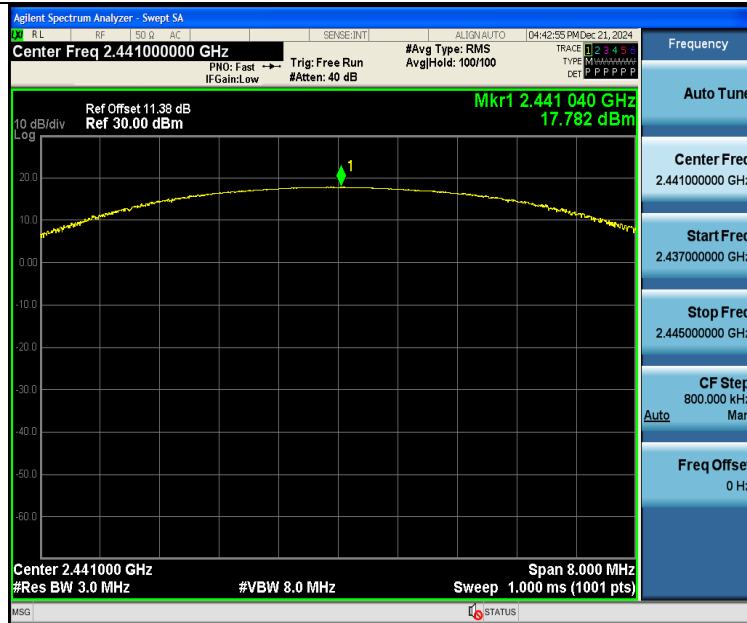
3DH5-Ant4-2441-PASS
