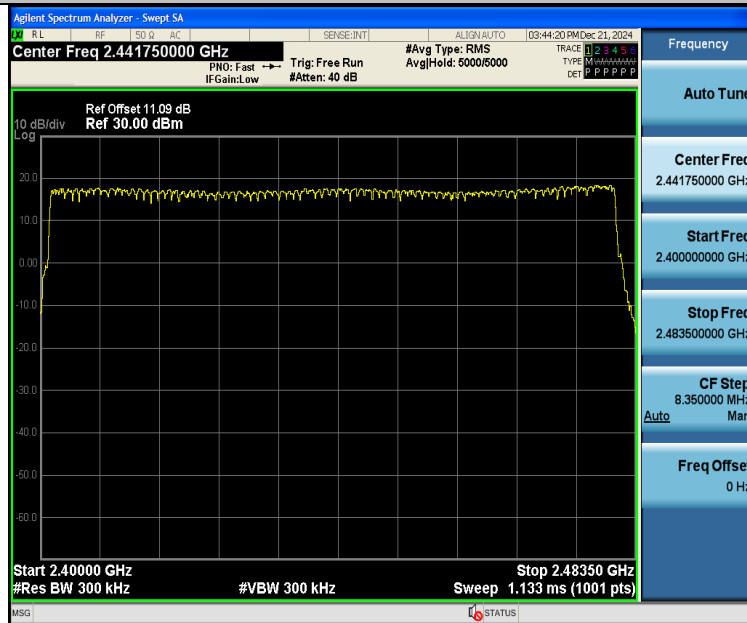
2DH5-Ant3-Hop-PASS
