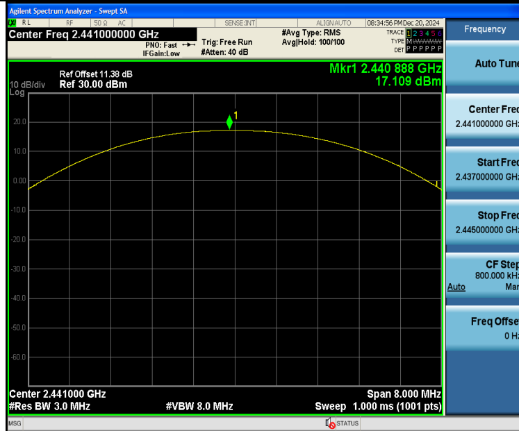
DH5-Ant2-2441-PASS
