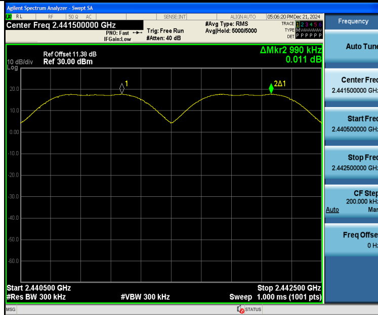
DH5-Ant4-Hop-PASS
