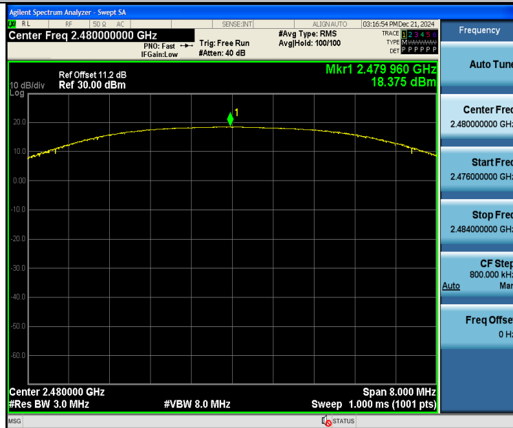
2DH5-Ant3-2480-PASS
