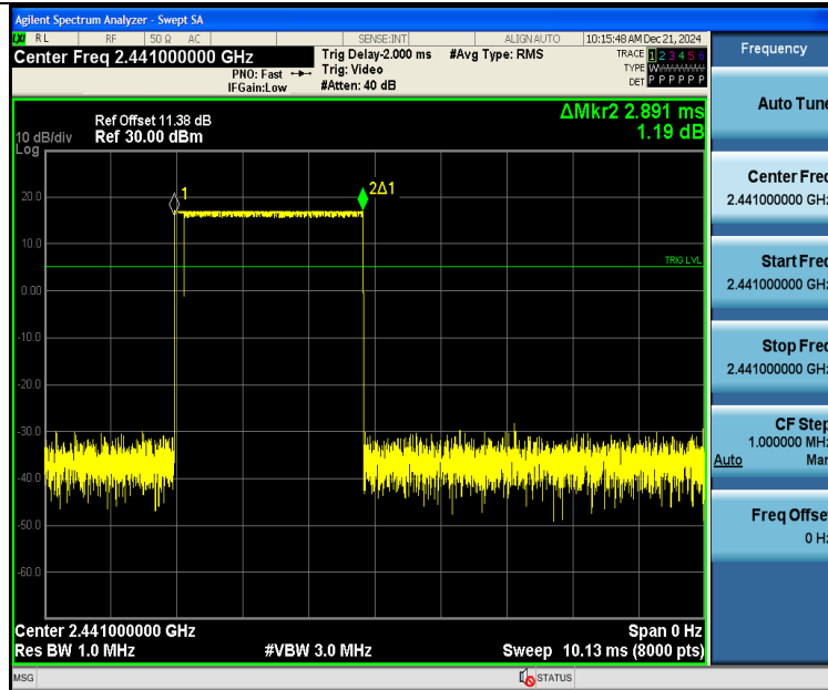
2DH5-Ant2-Hop-PASS
