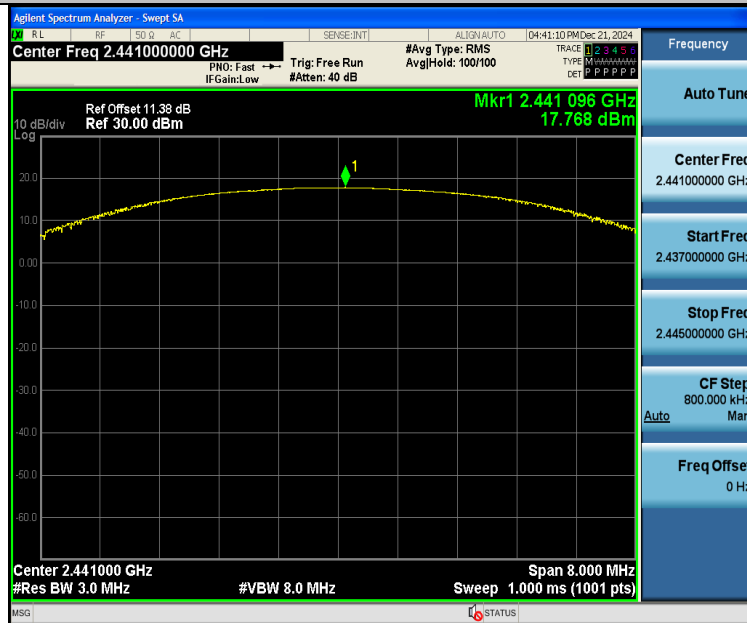
2DH5-Ant4-2441-PASS
