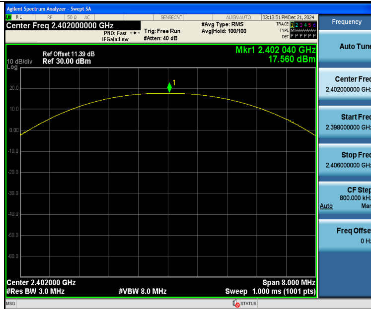
DH5-Ant3-2402-PASS
