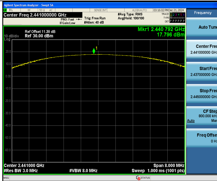
2DH5-Ant3-2441-PASS
