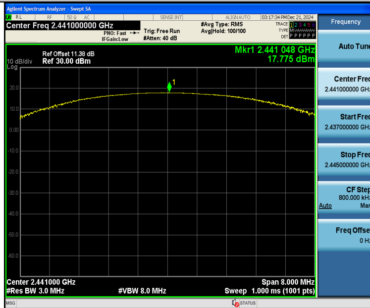
3DH5-Ant3-2441-PASS
