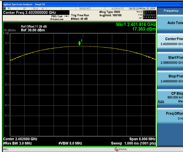
2DH5-Ant2-2402-PASS
