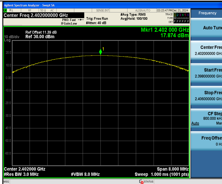
2DH5-Ant3-2402-PASS
