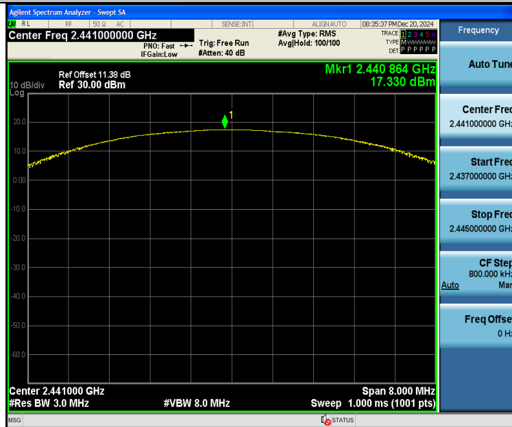
2DH5-Ant2-2441-PASS
