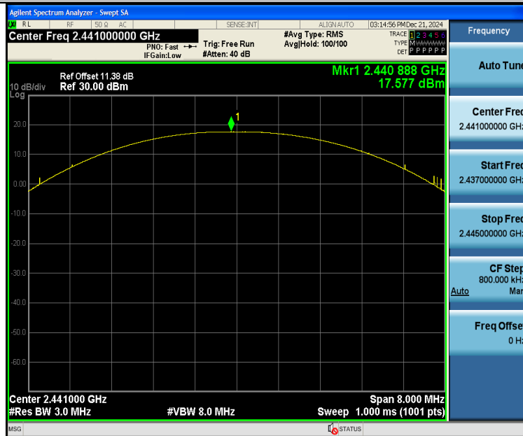
DH5-Ant3-2441-PASS
