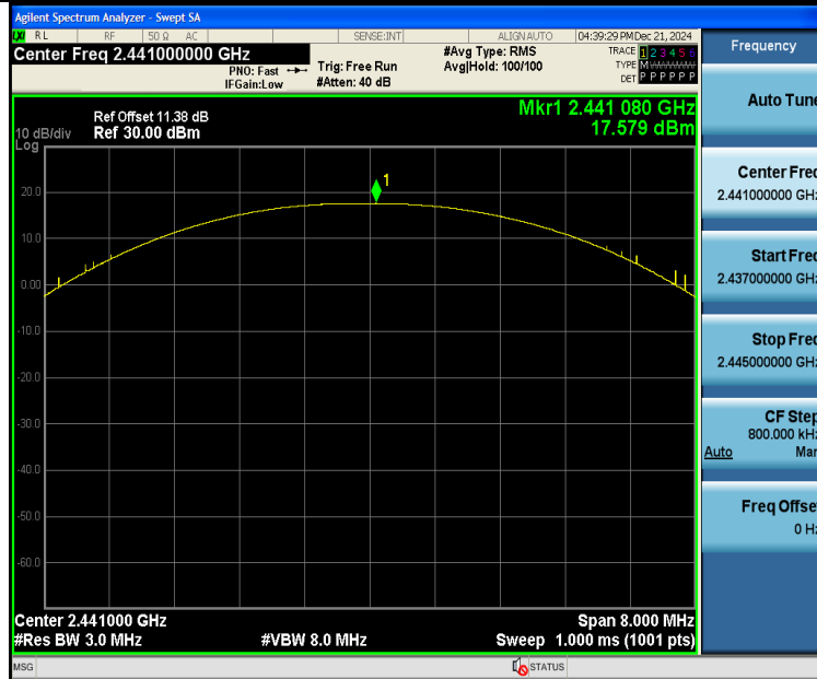
DH5-Ant4-2441-PASS
