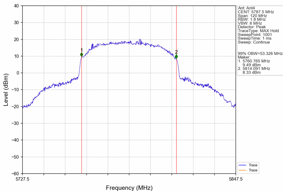
60M_MCH_5787.5MHz_Ant4_NTNV
