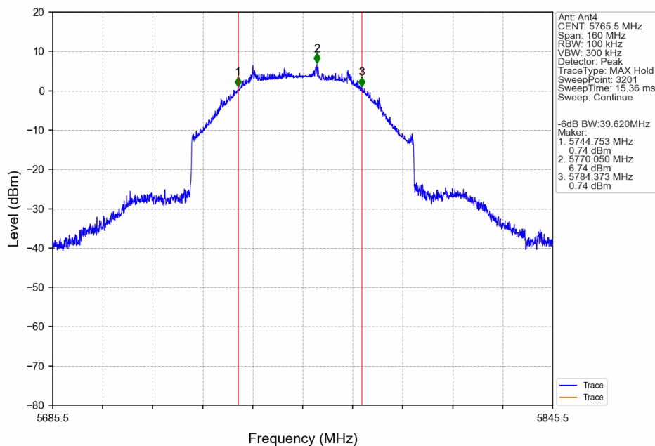
80M_LCH_5765.5MHz_Ant4_NTNV
