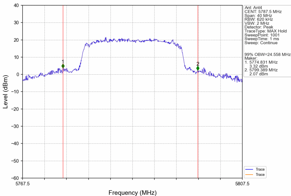
20M_MCH_5787.5MHz_Ant4_NTNV
