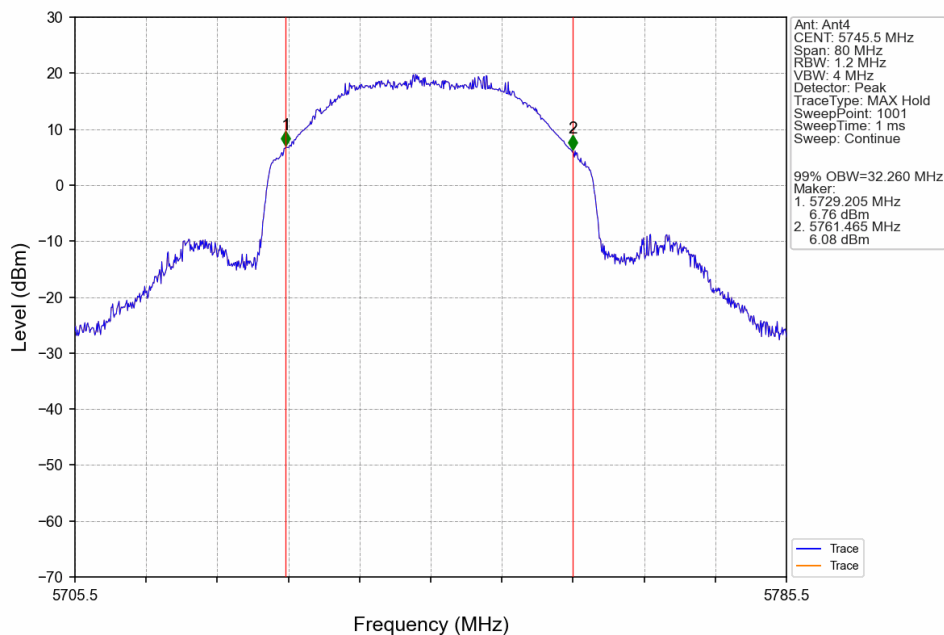
40M_LCH_5745.5MHz_Ant4_NTNV
