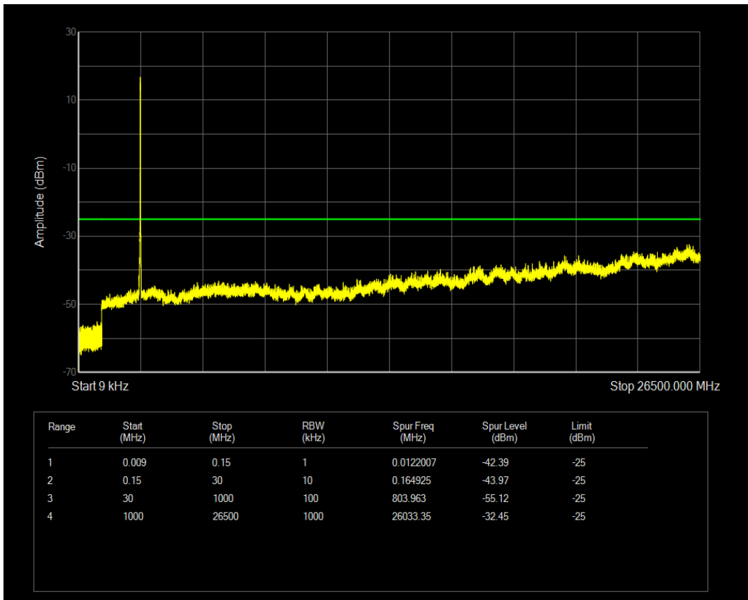
Band41 16QAM BW=20MHz Channel=41140 RB Size=1 Position=#0
