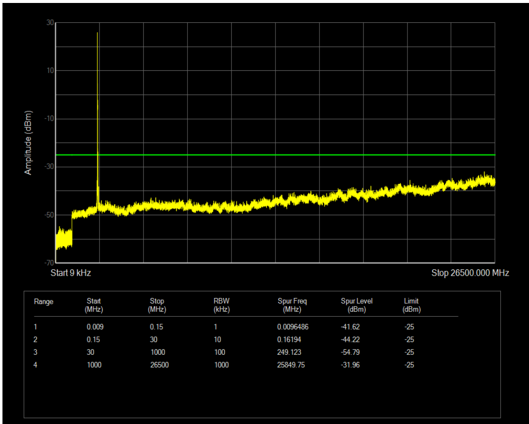
Band41 16QAM BW=20MHz Channel=40140 RB Size=1 Position=#0
