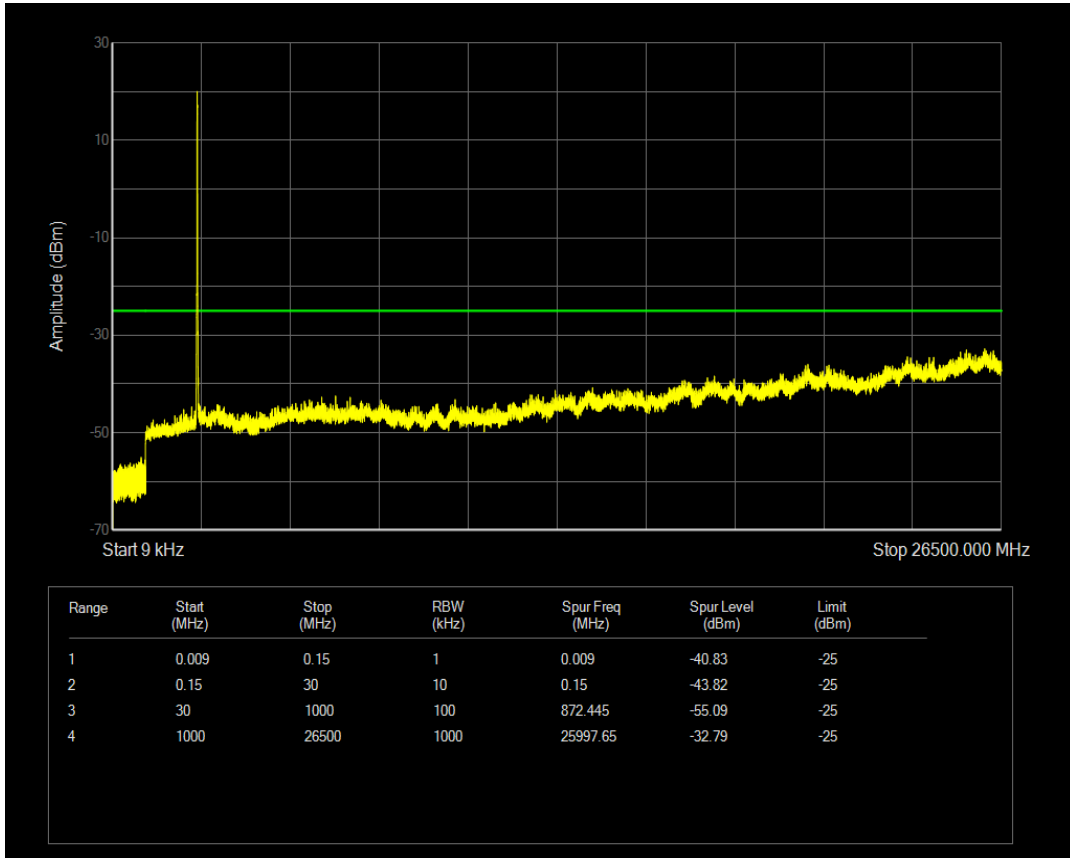
Band41 16QAM BW=15MHz Channel=40115 RB Size=1 Position=#0
