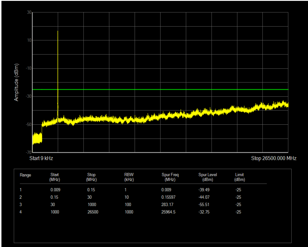
Band41 16QAM BW=15MHz Channel=41165 RB Size=1 Position=#0
