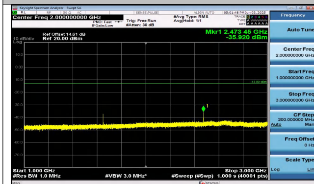
Band26(824-849)-10MHz-16QAM-26840-1RB#0-1000~3000-PASS
