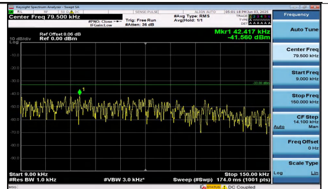
Band26(824-849)-10MHz-16QAM-26840-1RB#0-0.009~0.15-PASS
