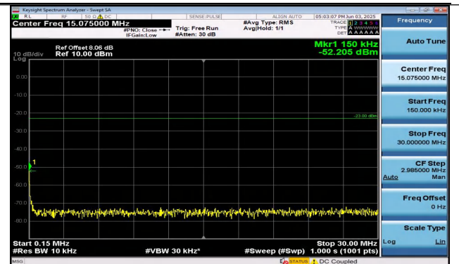
Band26(824-849)-10MHz-16QAM-26840-1RB#49-0.15~30-PASS
