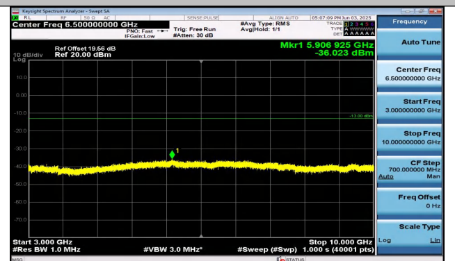
Band26(824-849)-10MHz-16QAM-26915-1RB#49-3000~10000-PASS
