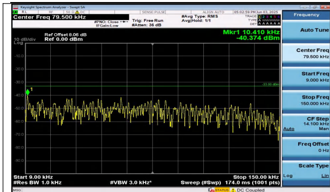
Band26(824-849)-10MHz-16QAM-26840-1RB#49-0.009~0.15-PASS
