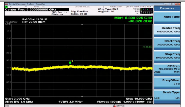
Band26(824-849)-10MHz-QPSK-26915-1RB#0-3000~100 00-PASS
