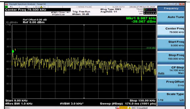
Band26(824-849)-10MHz-16QAM-26915-1RB#49-0.009~0.15-PASS
