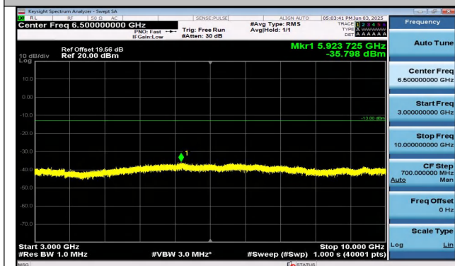
Band26(824-849)-10MHz-16QAM-26840-1RB#49-3000~10000-0000-PASS
