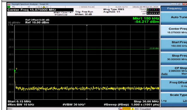
Band26(824-849)-10MHz-16QAM-26840-1RB#0-0.15~30-PASS
