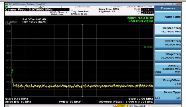
Band26(824-849)-10MHz-16QAM-26915-1RB#0-0.15~30- PASS
