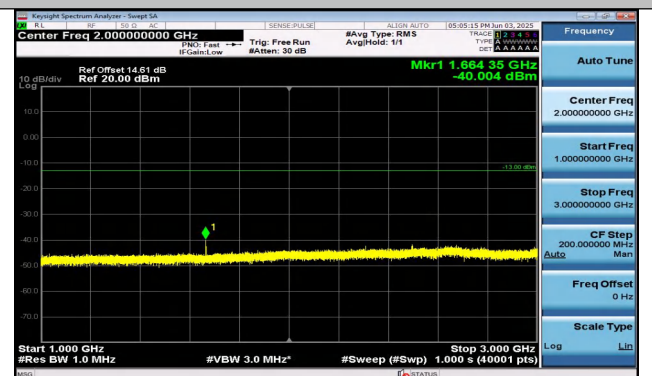
Band26(824-849)-10MHz-16QAM-26915-1RB#0-1000~30 00-PASS
