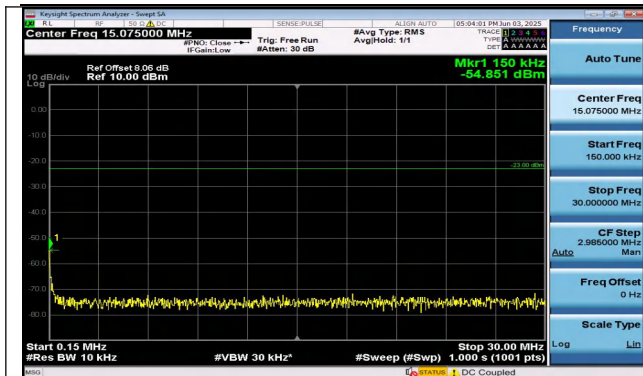
Band26(824-849)-10MHz-QPSK-26915-1RB#0-0.15~30-P ASS
