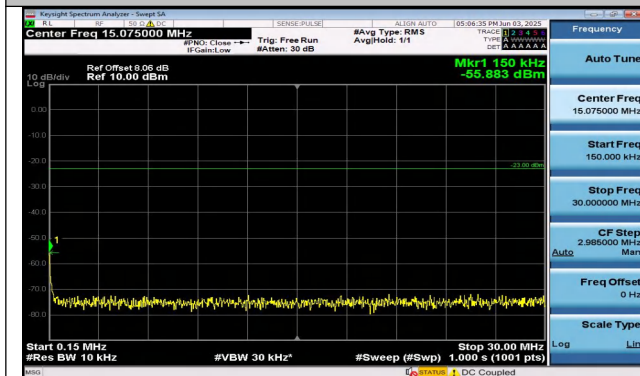
Band26(824-849)-10MHz-16QAM-26915-1RB#49-0.15~30-PASS
