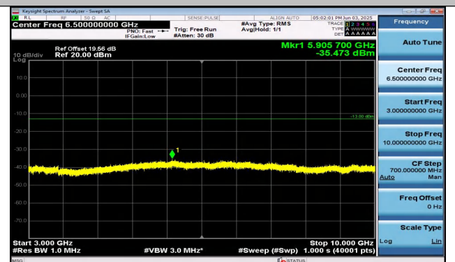
Band26(824-849)-10MHz-16QAM-26840-1RB#0-3000~10000-PASS
