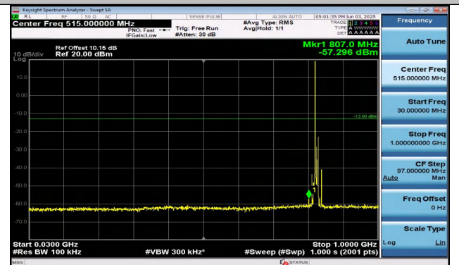
Band26(824-849)-10MHz-16QAM-26840-1RB#0-30~1000-PASS
