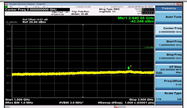
Band26(824-849)-10MHz-16QAM-26840-1RB#49-1000~3000-000-PASS
