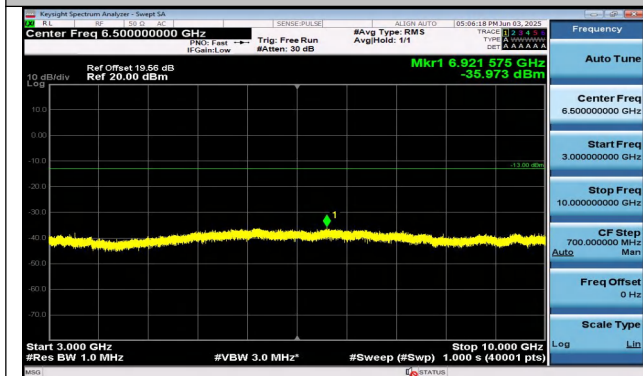
Band26(824-849)-10MHz-QPSK-26915-1RB#49-3000~10000- 000-PASS
