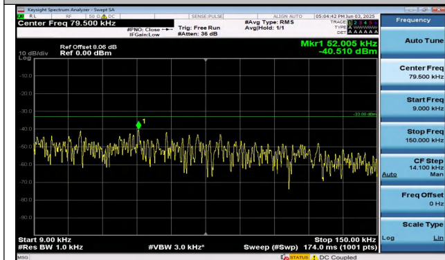
Band26(824-849)-10MHz-16QAM-26915-1RB#0-0.009~0. 15-PASS
