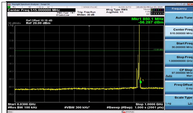
Band26(824-849)-10MHz-QPSK-26915-1RB#49-30~1000- PASS
