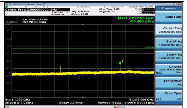
Band26(824-849)-10MHz-QPSK-26915-1RB#49-1000~3000- 00-PASS
