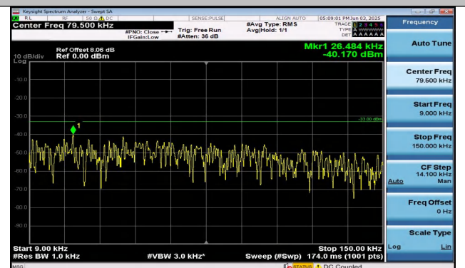
Band26(824-849)-10MHz-QPSK-26990-1RB#49-0.009~0. 15-PASS
