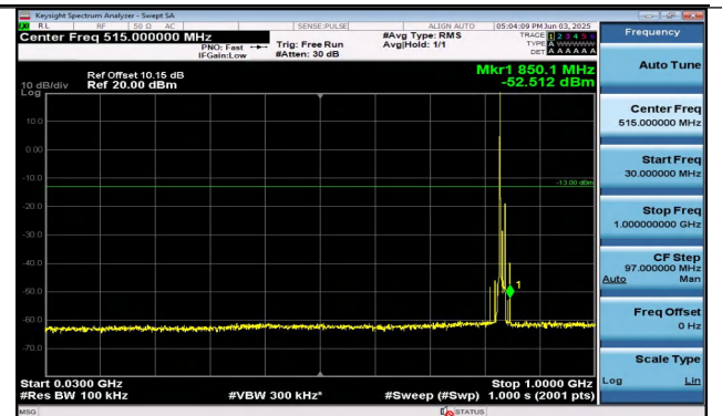
Band26(824-849)-10MHz-QPSK-26915-1RB#0-30~1000-P ASS
