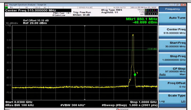
Band26(824-849)-10MHz-QPSK-26915-50RB#0-30~1000- PASS
