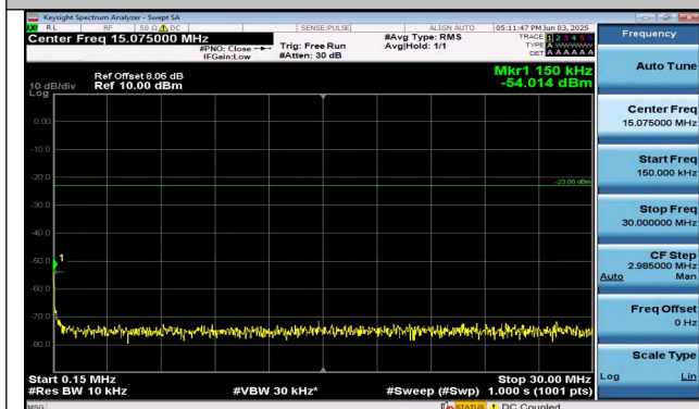
Band26(824-849)-10MHz-QPSK-26915-50RB#0-0.15~30- PASS
