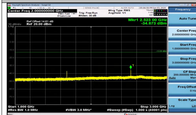
Band26(824-849)-10MHz-16QAM-26915-1RB#49-1000~3000-PASS
