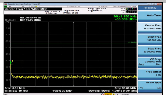
Band26(824-849)-10MHz-QPSK-26915-1RB#49-0.15~30- PASS
