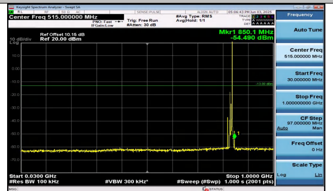
Band26(824-849)-10MHz-16QAM-26915-1RB#49-30~1000-PASS
