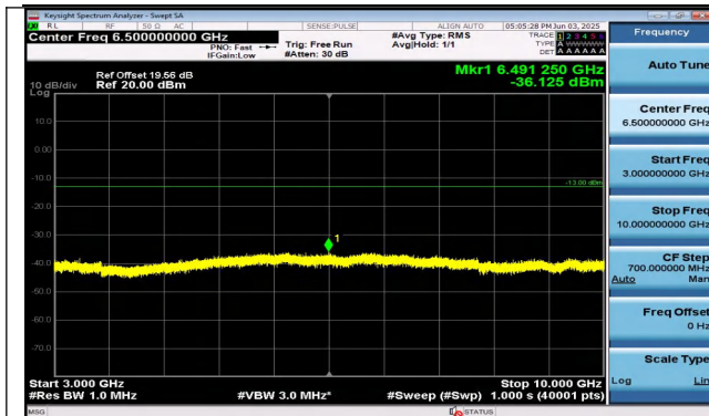
Band26(824-849)-10MHz-16QAM-26915-1RB#0-3000~10000-PASS
