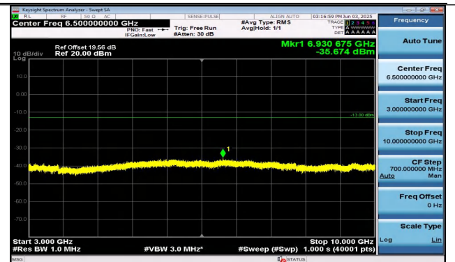
Band26(824-849)-3MHz-QPSK-26805-1RB#14-3000~100 00-PASS
