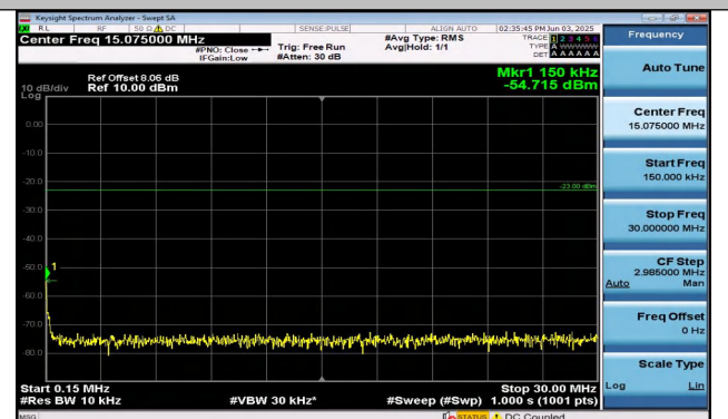
Band26(824-849)-1.4MHz-QPSK-27033-1RB#0-0.15~30-P ASS
