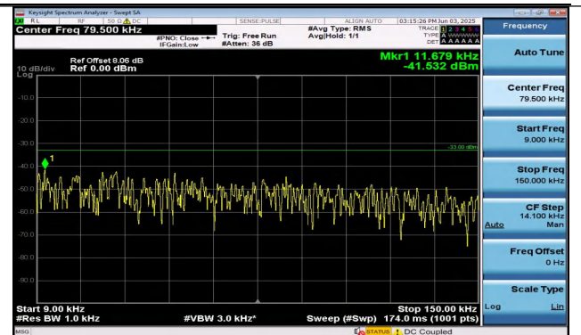
Band26(824-849)-3MHz-16QAM-26805-1RB#0-0.009~0.1 5-PASS
