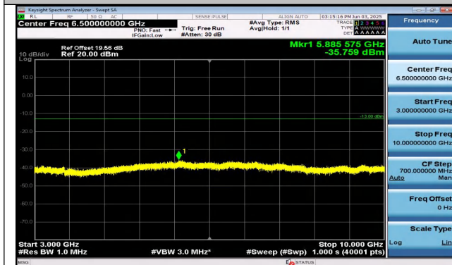
Band26(824-849)-3MHz-QPSK-26805-1RB#0-3000~1000
