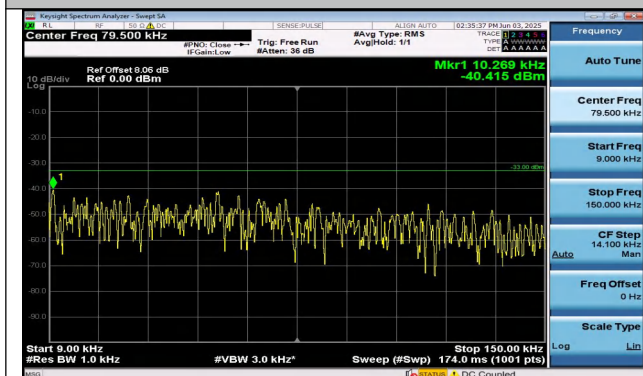
Band26(824-849)-1.4MHz-QPSK-27033-1RB#0-0.009~0.1 5-PASS
