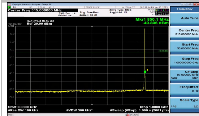
Band26(824-849)-1.4MHz-QPSK-27033-6RB#0-30~1000- PASS
