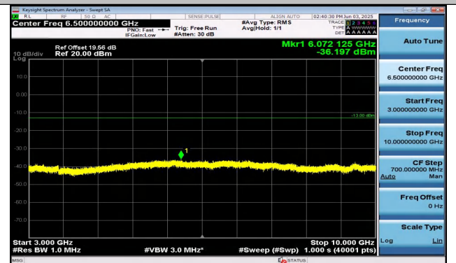
Band26(824-849)-1.4MHz-16QAM-27033-6RB#0-3000~10 000-PASS
