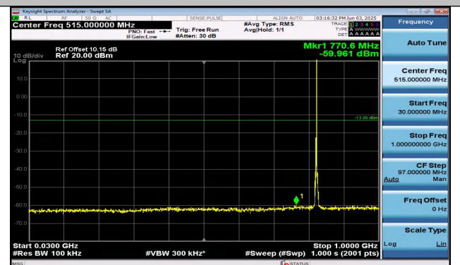
Band26(824-849)-3MHz-QPSK-26805-1RB#14-30~1000-P
