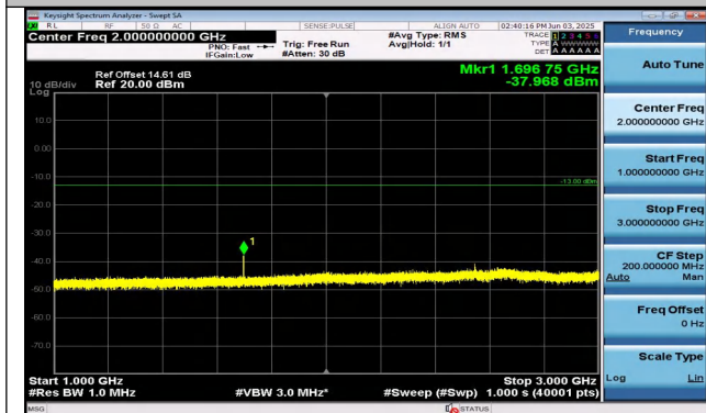
Band26(824-849)-1.4MHz-16QAM-27033-6RB#0-1000~30 00-PASS
