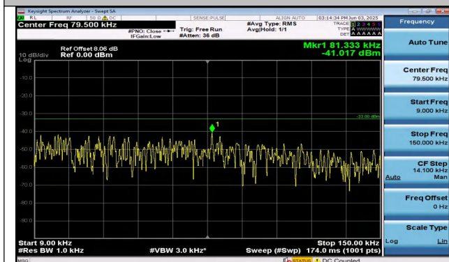
Band26(824-849)-3MHz-QPSK-26805-1RB#0-0.009~0.15- PASS
