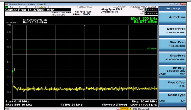
Band26(824-849)-1.4MHz-QPSK-27033-6RB#0-0.15~30-P ASS
