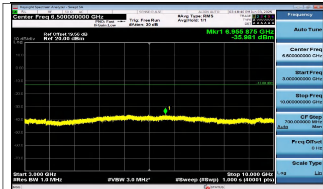
Band26(824-849)-3MHz-QPSK-26805-15RB#0-3000~100 00-PASS
