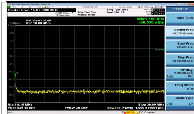
Band26(824-849)-1.4MHz-16QAM-26915-6RB#0-0.15~30- PASS
