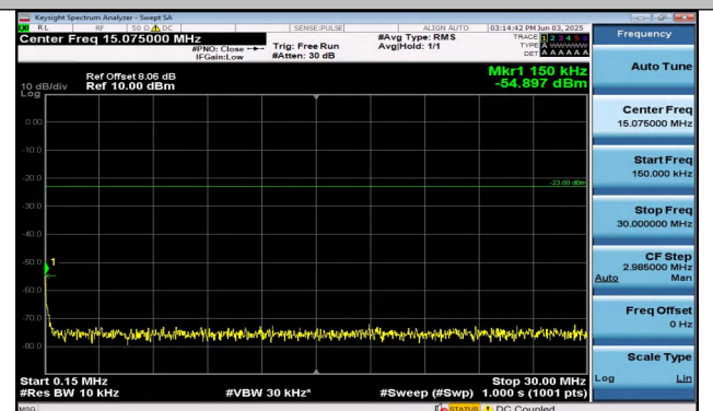
Band26(824-849)-3MHz-QPSK-26805-1RB#0-0.15~30-PA SS
