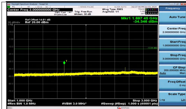
Band26(824-849)-1.4MHz-QPSK-27033-1RB#5-1000~300 0-PASS
