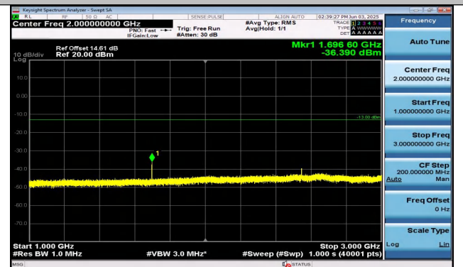
Band26(824-849)-1.4MHz-QPSK-27033-6RB#0-1000~300 0-PASS
