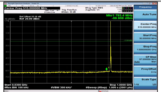
Band26(824-849)-3MHz-16QAM-26805-1RB#0-30~1000-P ASS
