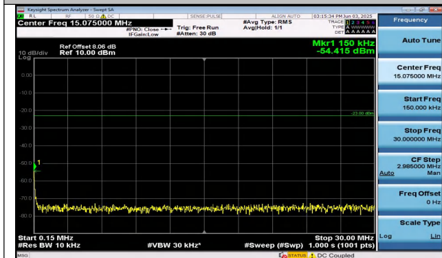
Band26(824-849)-3MHz-16QAM-26805-1RB#0-0.15~30-P ASS
