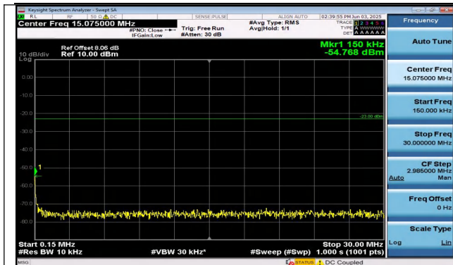
Band26(824-849)-1.4MHz-16QAM-27033-6RB#0-0.15~30- PASS
