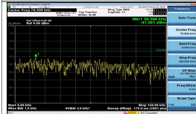
Band26(824-849)-1.4MHz-QPSK-27033-6RB#0-0.009~0.1 5-PASS
