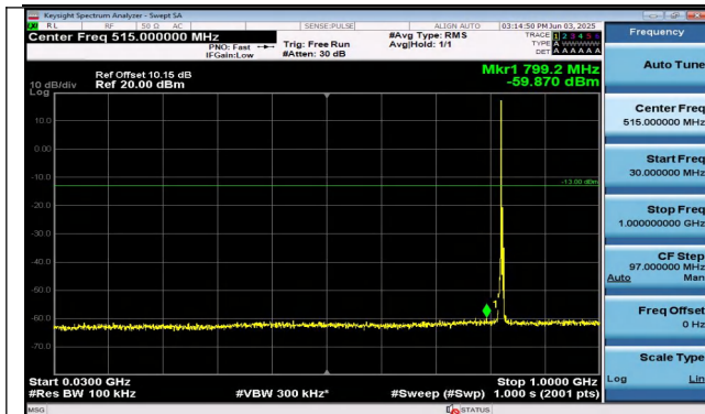
Band26(824-849)-3MHz-QPSK-26805-1RB#0-30~1000-P
