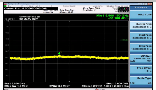
Band26(824-849)-3MHz-16QAM-26805-1RB#0-3000~100 00-PASS
