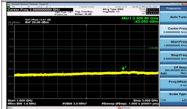
Band26(824-849)-1.4MHz-16QAM-26915-6RB#0-1000~30 00-PASS
