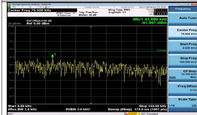
Band26(824-849)-3MHz-QPSK-26805-15RB#0-0.009~0.1 5-PASS
