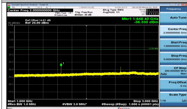
Band26(824-849)-3MHz-16QAM-26805-1RB#0-1000~300 0-PASS
