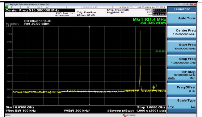
Band26(824-849)-1.4MHz-16QAM-26915-6RB#0-30~1000 -PASS
