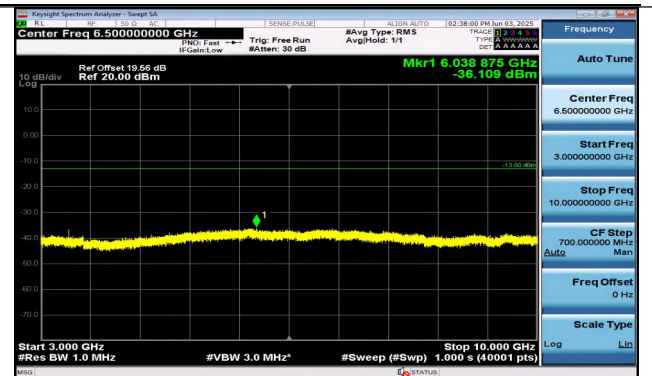
Band26(824-849)-1.4MHz-QPSK-27033-1RB#5-3000~100 00-PASS
