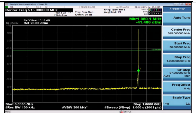
Band26(824-849)-1.4MHz-16QAM-27033-6RB#0-30~1000 -PASS
