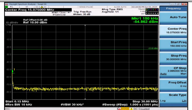
Band26(824-849)-3MHz-QPSK-26805-15RB#0-0.15~30-P ASS
