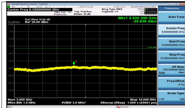
Band26(824-849)-1.4MHz-QPSK-26797-6RB#0-3000~100 00-PASS
