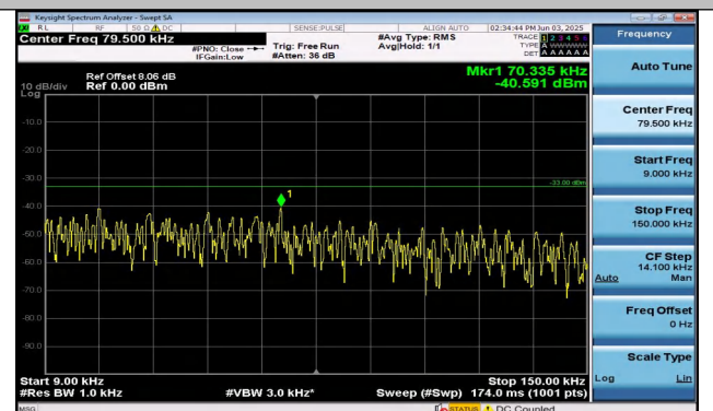
Band26(824-849)-1.4MHz-16QAM-26915-6RB#0-0.009~0. 15-PASS
