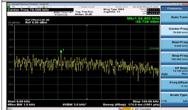
Band26(824-849)-1.4MHz-QPSK-26915-6RB#0-0.009~0.1 5-PASS
