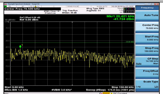
Band26(824-849)-1.4MHz-16QAM-26797-6RB#0-0.009~0. 15-PASS
