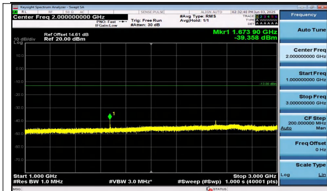
Band26(824-849)-1.4MHz-QPSK-26915-1RB#5-1000~300 0-PASS
