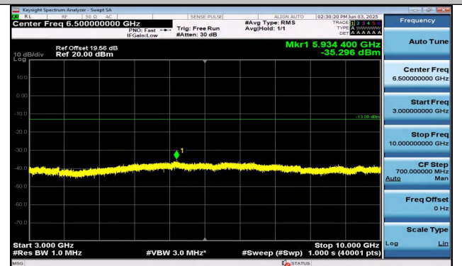
Band26(824-849)-1.4MHz-16QAM-26797-6RB#0-3000~10 000-PASS
