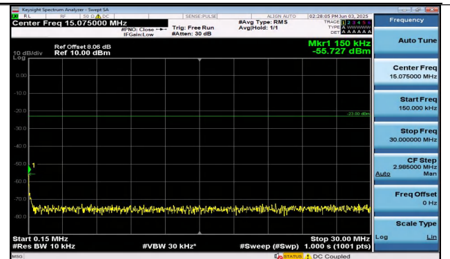
Band26(824-849)-1.4MHz-16QAM-26797-1RB#5-0.15~30- PASS
