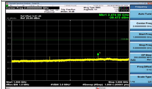
Band26(824-849)-1.4MHz-16QAM-26797-6RB#0-1000~30 00-PASS
