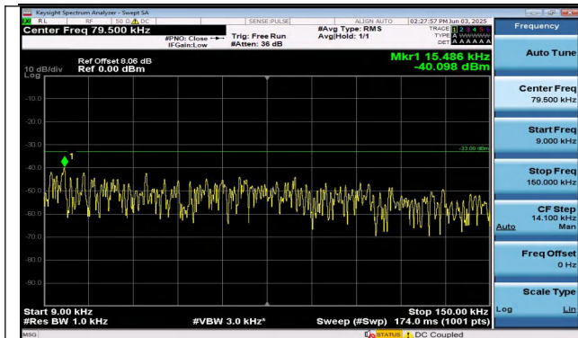
Band26(824-849)-1.4MHz-16QAM-26797-1RB#5-0.009~0. 15-PASS
