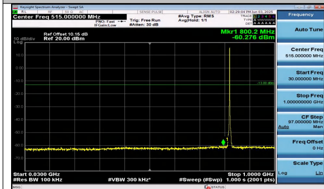
Band26(824-849)-1.4MHz-QPSK-26797-6RB#0-30~1000- PASS
