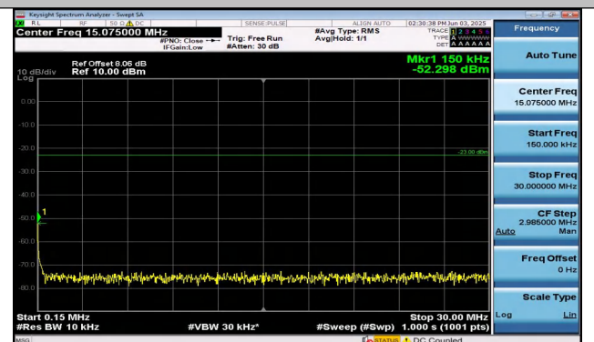
Band26(824-849)-1.4MHz-QPSK-26915-1RB#0-0.15~30-P ASS
