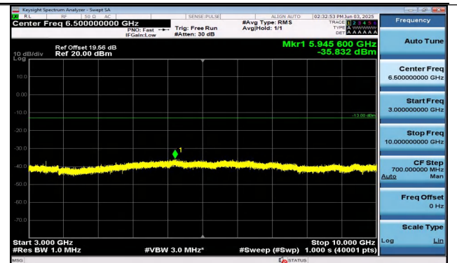
Band26(824-849)-1.4MHz-QPSK-26915-1RB#5-3000~100 00-PASS
