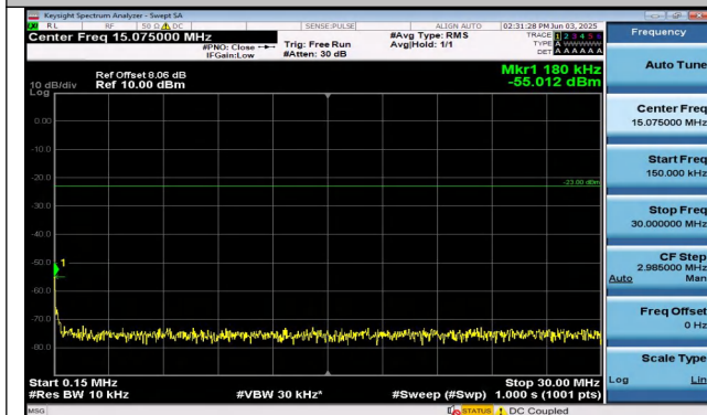
Band26(824-849)-1.4MHz-16QAM-26915-1RB#0-0.15~30- PASS
