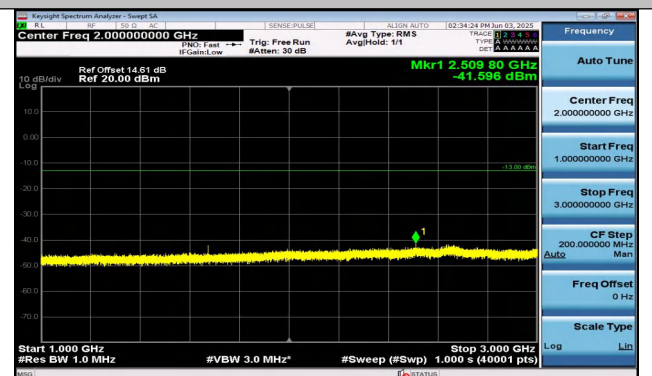
Band26(824-849)-1.4MHz-QPSK-26915-6RB#0-1000~300 0-PASS
