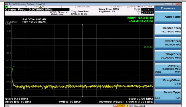
Band26(824-849)-1.4MHz-QPSK-26915-6RB#0-0.15~30-P ASS
