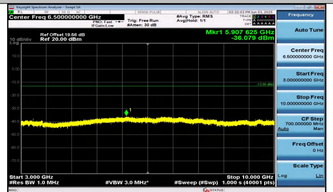
Band26(824-849)-1.4MHz-16QAM-26915-1RB#0-3000~10 000-PASS
