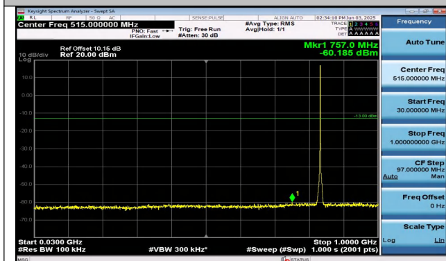
Band26(824-849)-1.4MHz-QPSK-26915-6RB#0-30~1000- PASS
