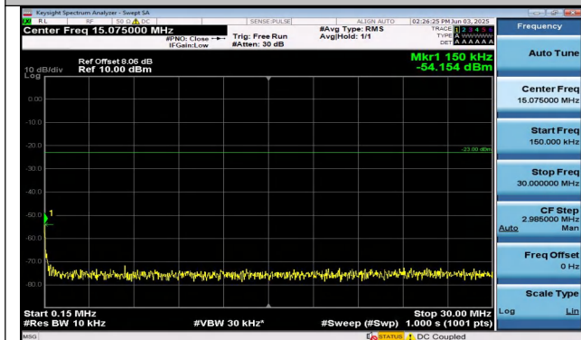
Band26(824-849)-1.4MHz-16QAM-26797-1RB#0-0.15~30- PASS
