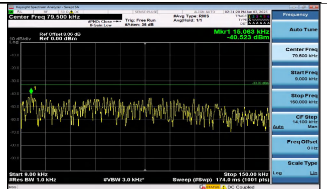
Band26(824-849)-1.4MHz-16QAM-26915-1RB#0-0.009~0. 15-PASS
