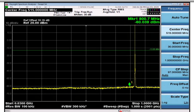
Band26(824-849)-1.4MHz-16QAM-26915-1RB#0-30~1000 -PASS
