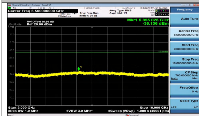
Band26(824-849)-1.4MHz-16QAM-26797-1RB#5-3000~10000- 000-PASS
