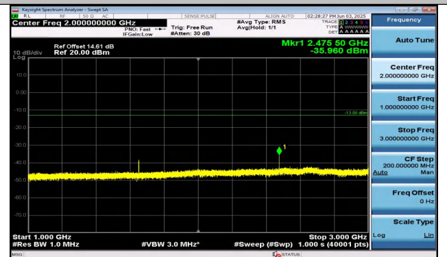
Band26(824-849)-1.4MHz-16QAM-26797-1RB#5-1000~3000- 00-PASS
