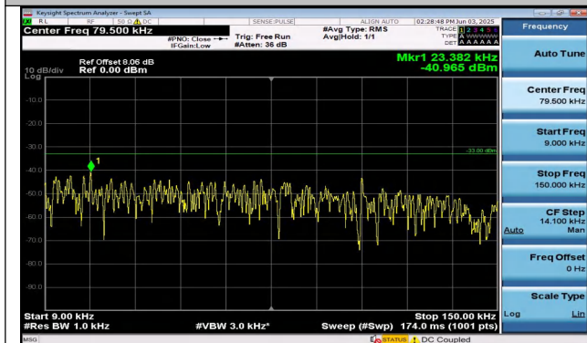
Band26(824-849)-1.4MHz-QPSK-26797-6RB#0-0.009~0.1 5-PASS
