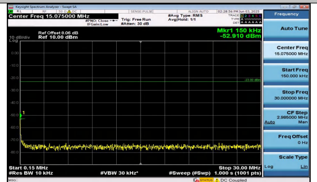
Band26(824-849)-1.4MHz-QPSK-26797-6RB#0-0.15~30-P ASS
