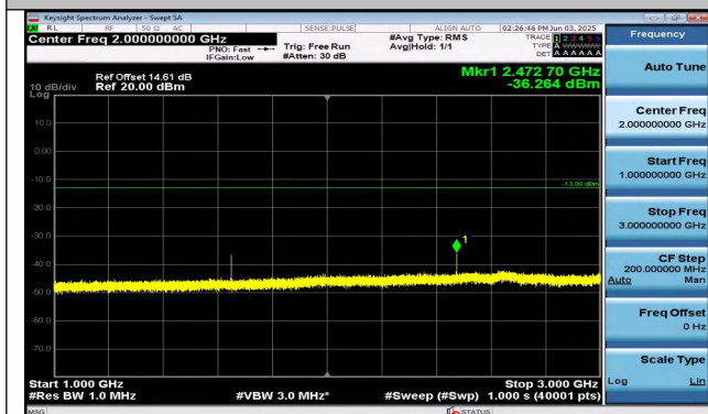
Band26(824-849)-1.4MHz-16QAM-26797-1RB#0-1000~30 00-PASS
