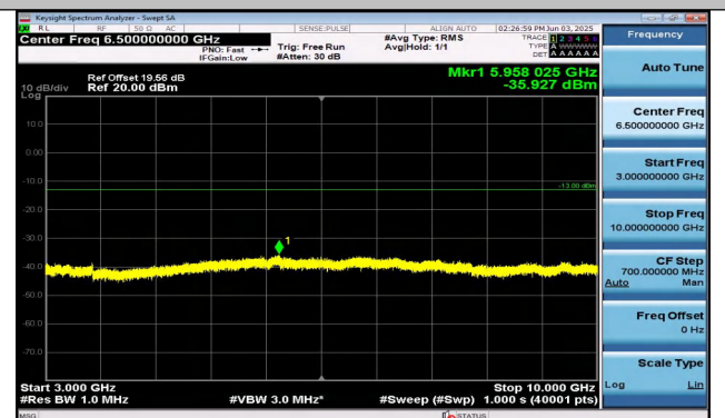
Band26(824-849)-1.4MHz-16QAM-26797-1RB#0-3000~10 000-PASS
