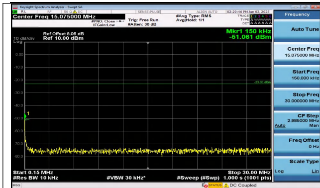
Band26(824-849)-1.4MHz-16QAM-26797-6RB#0-0.15~30- PASS
