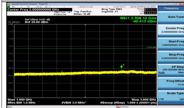
Band26(824-849)-1.4MHz-16QAM-26915-1RB#0-1000~30 00-PASS
