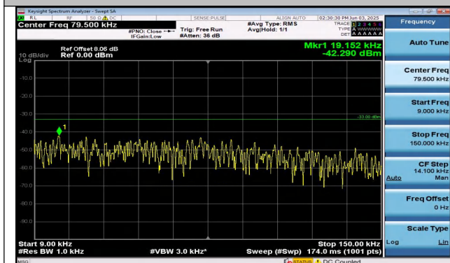
Band26(824-849)-1.4MHz-QPSK-26915-1RB#0-0.009~0.1 5-PASS
