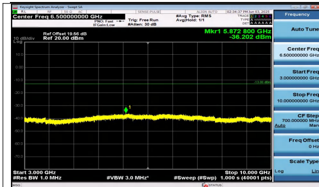
Band26(824-849)-1.4MHz-QPSK-26915-6RB#0-3000~100 00-PASS
