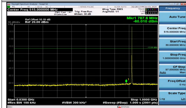
Band26(824-849)-1.4MHz-16QAM-26797-1RB#5-30~1000- -PASS
