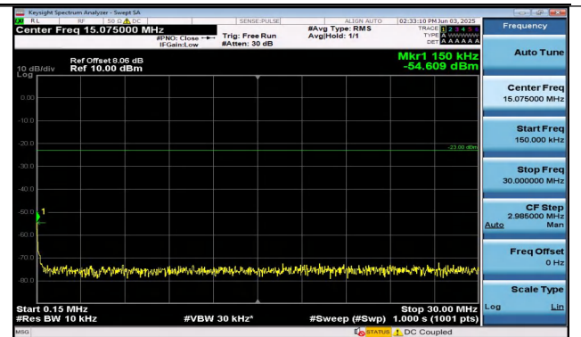
Band26(824-849)-1.4MHz-16QAM-26915-1RB#5-0.15~30-. PASS
