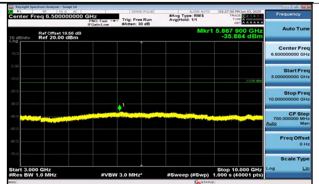
Band26(824-849)-1.4MHz-QPSK-26797-1RB#5-3000~100 00-PASS
