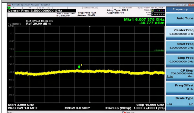
Band26(824-849)-1.4MHz-16QAM-26915-1RB#5-3000~10000-. 000-PASS
