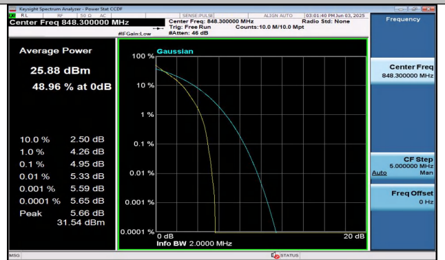
Band26(824-849)-1.4MHz-QPSK-27033-6RB#0-PASS
