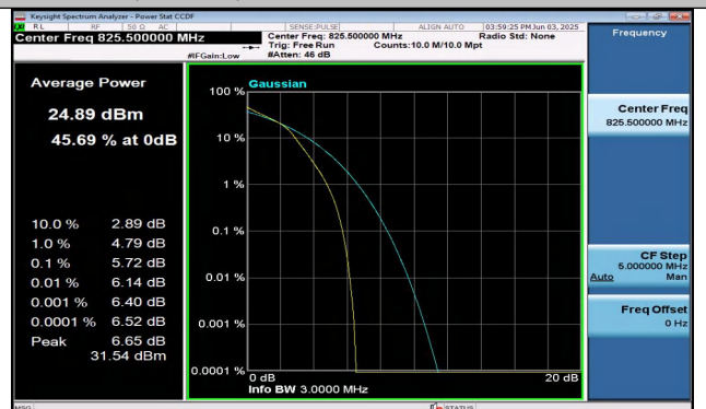
Band26(824-849)-3MHz-16QAM-26805-15RB#0-PASS
