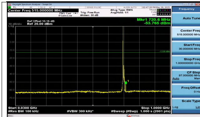
Band12-10MHz-16QAM-23095-1RB#0-30~1000-PASS
