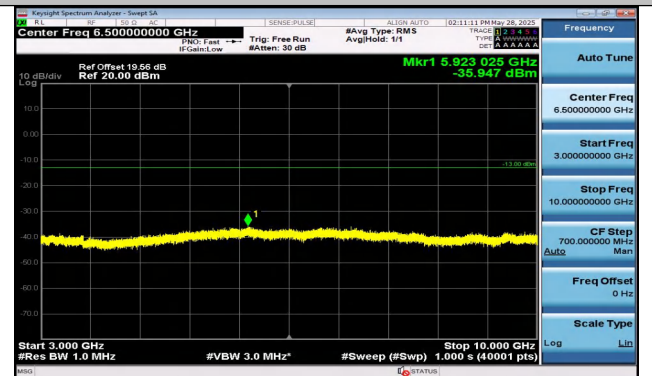
Band12-5MHz-16QAM-23155-25RB#0-3000~10000-PASS
