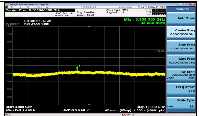
Band12-10MHz-16QAM-23060-1RB#0-3000~10000-PASS
