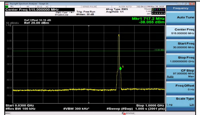
Band12-10MHz-QPSK-23095-50RB#0-30~1000-PASS
