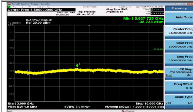
Band12-10MHz-16QAM-23060-1RB#49-3000~10000-PAS
