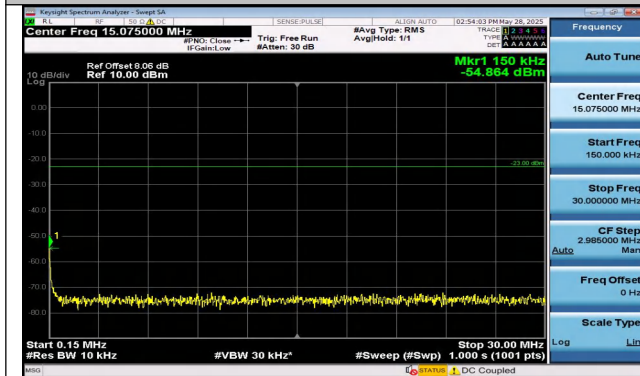
Band12-10MHz-QPSK-23095-50RB#0-0.15~30-PASS
