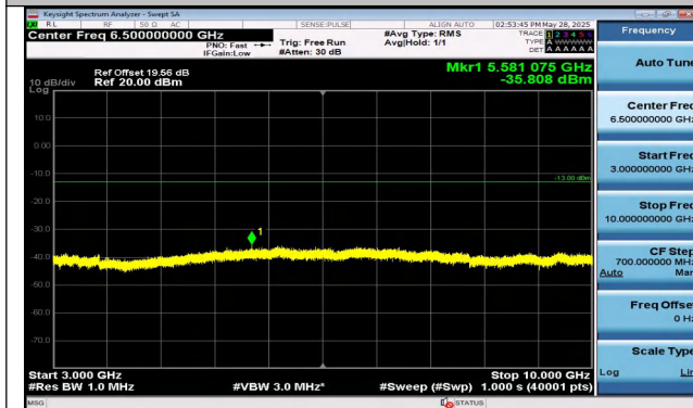
Band12-10MHz-QPSK-23060-50RB#0-3000~10000-PASS
