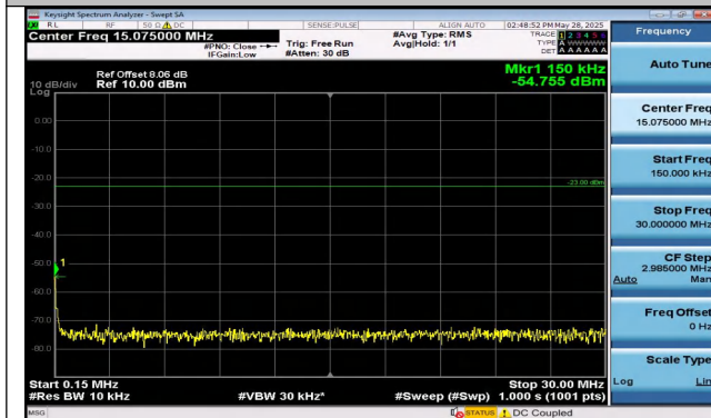
Band12-10MHz-16QAM-23095-1RB#49-0.15~30-PASS
