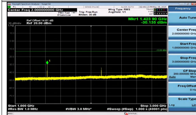
Band12-10MHz-16QAM-23095-1RB#49-1000~3000-PASS
