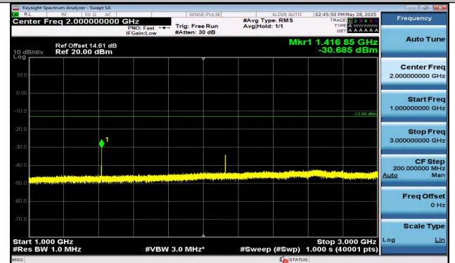
Band12-10MHz-16QAM-23060-1RB#49-1000~3000-PASS
