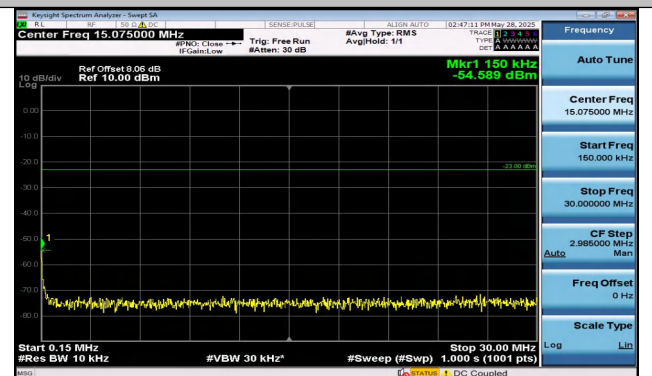
Band12-10MHz-16QAM-23095-1RB#0-0.15~30-PASS
