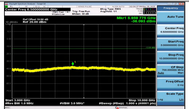
Band12-10MHz-QPSK-23095-50RB#0-3000~10000-PASS
