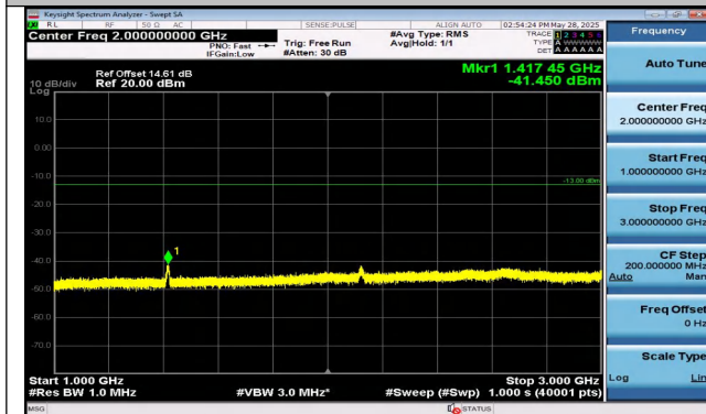
Band12-10MHz-QPSK-23095-50RB#0-1000~3000-PASS
