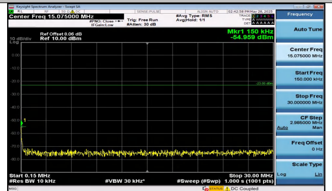
Band12-10MHz-QPSK-23060-1RB#0-0.15~30-PASS
