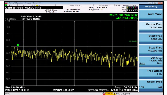
Band12-10MHz-QPSK-23130-1RB#49-0.009~0.15-PASS
