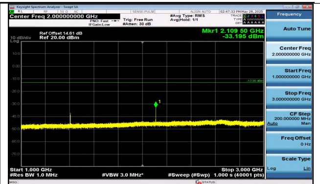
Band12-10MHz-16QAM-23095-1RB#0-1000~3000-PASS
