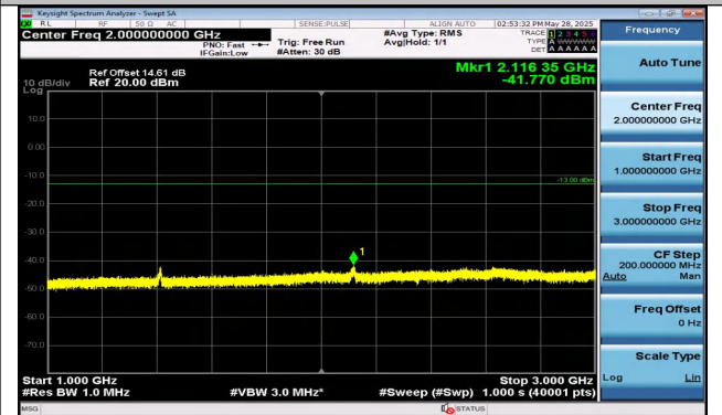
Band12-10MHz-QPSK-23060-50RB#0-1000~3000-PASS
