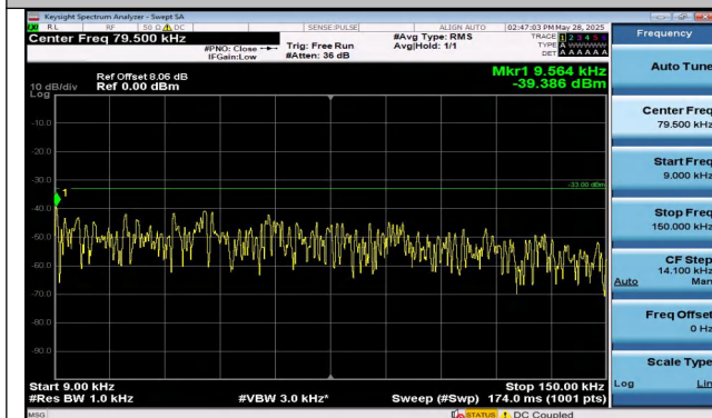
Band12-10MHz-16QAM-23095-1RB#0-0.009~0.15-PASS
