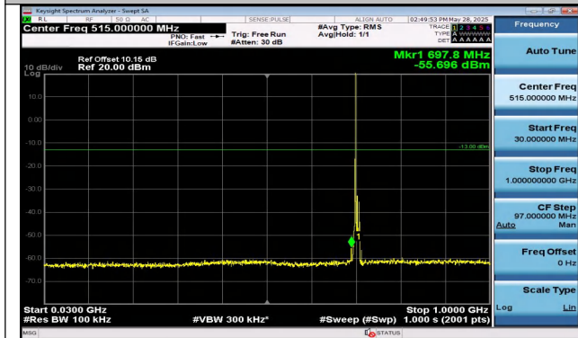
Band12-10MHz-QPSK-23130-1RB#0-30~1000-PASS
