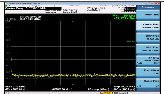
Band12-10MHz-QPSK-23130-1RB#0-0.15~30-PASS
