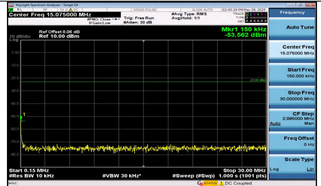
Band12-10MHz-16QAM-23060-1RB#49-0.15~30-PASS
