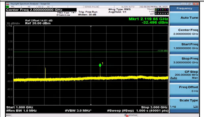
Band12-10MHz-QPSK-23130-1RB#0-1000~3000-PASS
