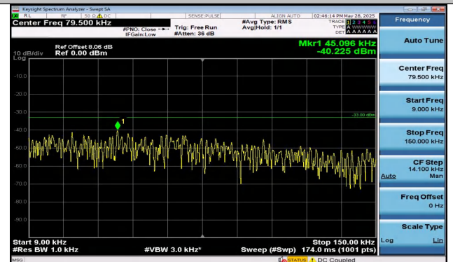
Band12-10MHz-QPSK-23095-1RB#0-0.009~0.15-PASS
