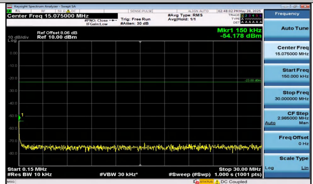
Band12-10MHz-QPSK-23095-1RB#49-0.15~30-PASS
