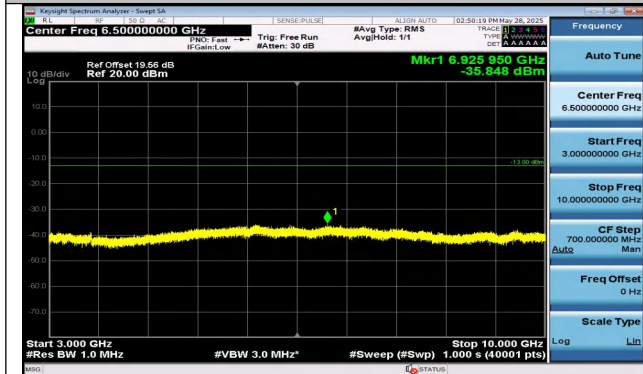
Band12-10MHz-QPSK-23130-1RB#0-3000~10000-PASS
