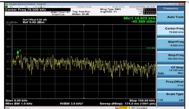
Band12-10MHz-QPSK-23095-50RB#0-0.009~0.15-PASS
