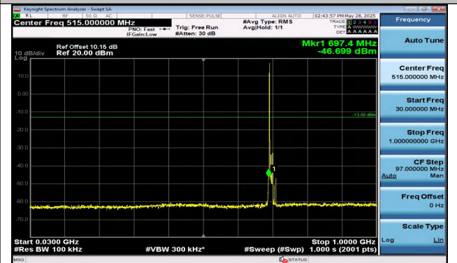
Band12-10MHz-16QAM-23060-1RB#0-30~1000-PASS
