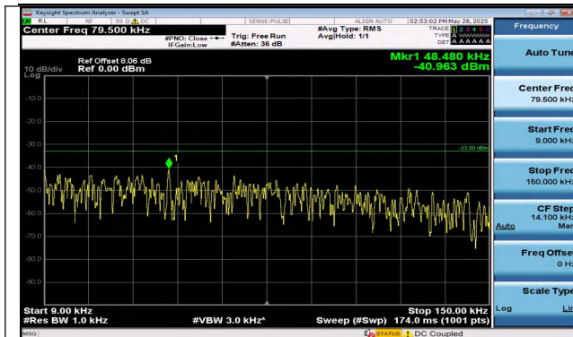
Band12-10MHz-QPSK-23060-50RB#0-0.009~0.15-PASS
