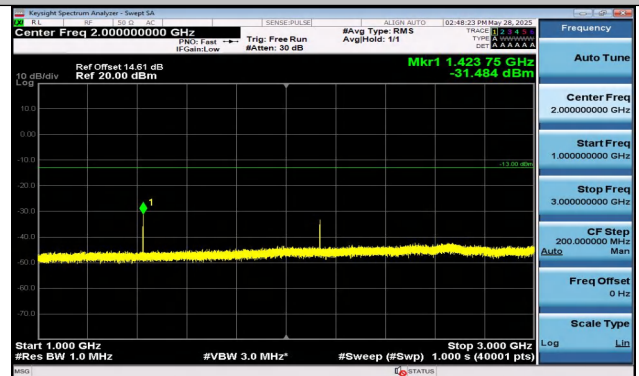
Band12-10MHz-QPSK-23095-1RB#49-1000~3000-PASS
