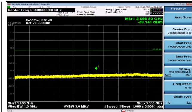
Band12-10MHz-16QAM-23060-1RB#0-1000~3000-PASS
