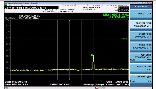
Band12-10MHz-QPSK-23130-1RB#49-30~1000-PASS
