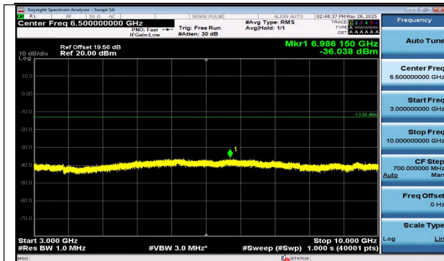
Band12-10MHz-QPSK-23095-1RB#49-3000~10000-PASS
