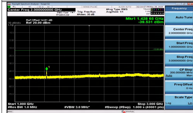
Band12-5MHz-16QAM-23155-25RB#0-1000~3000-PASS
