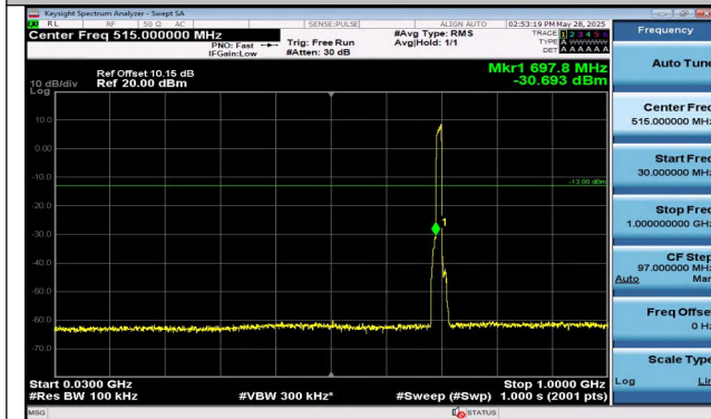
Band12-10MHz-QPSK-23060-50RB#0-0.30~1000-PASS
