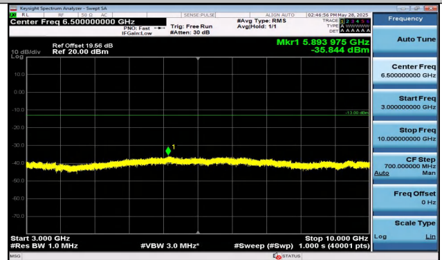
Band12-10MHz-QPSK-23095-1RB#0-3000~10000-PASS
