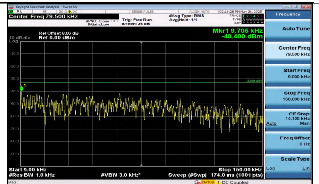
Band12-5MHz-16QAM-23155-25RB#0-0.009~0.15-PASS
