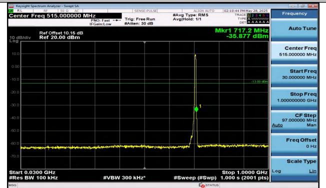
Band12-5MHz-16QAM-23155-25RB#0-30~1000-PASS
