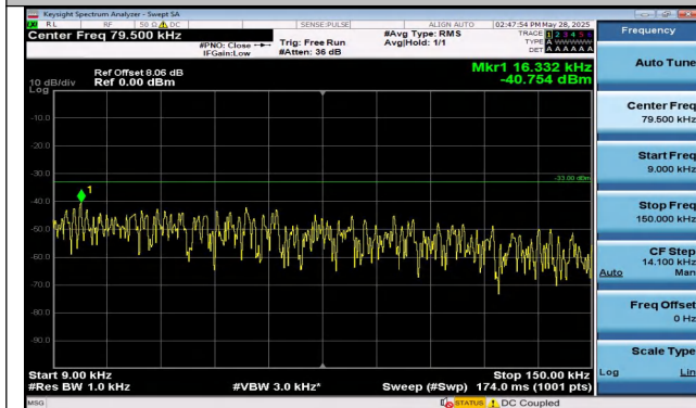
Band12-10MHz-QPSK-23095-1RB#49-0.009~0.15-PASS
