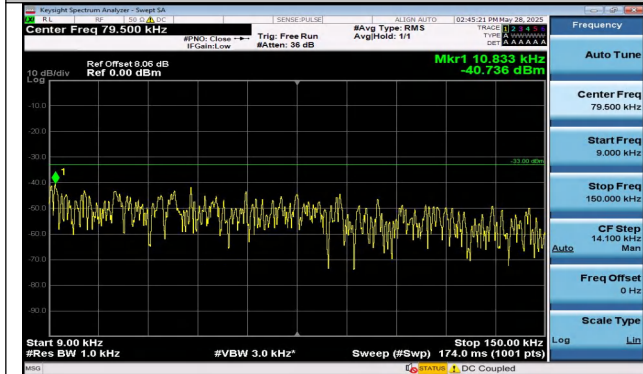
Band12-10MHz-16QAM-23060-1RB#49-0.009~0.15-PASS
