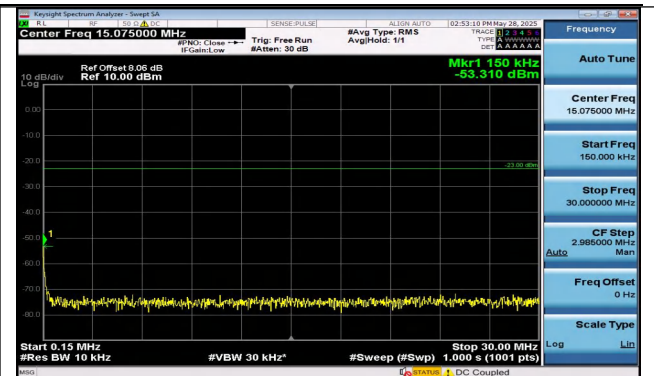
Band12-10MHz-QPSK-23060-50RB#0-0.15~30-PASS
