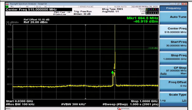
Band12-10MHz-16QAM-23095-1RB#49-30~1000-PASS
