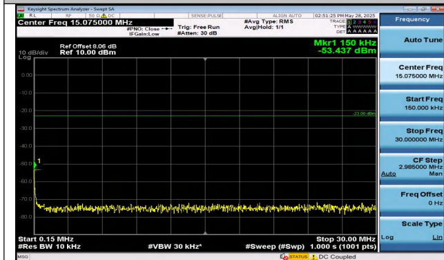
Band12-10MHz-QPSK-23130-1RB#49-0.15~30-PASS
