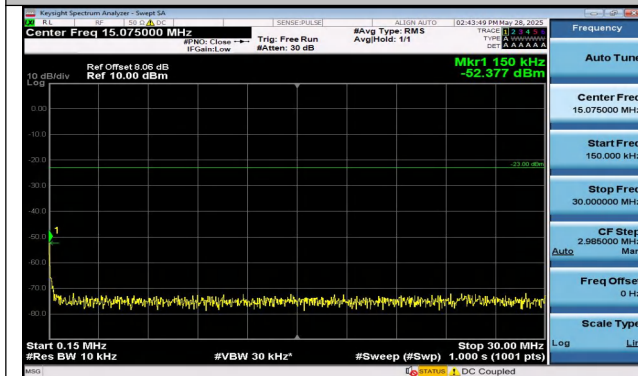
Band12-10MHz-16QAM-23060-1RB#0-0.15~30-PASS
