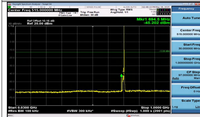
Band12-10MHz-QPSK-23095-1RB#49-30~1000-PASS
