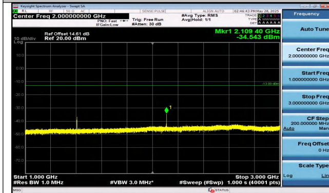
Band12-10MHz-QPSK-23095-1RB#0-1000~3000-PASS
