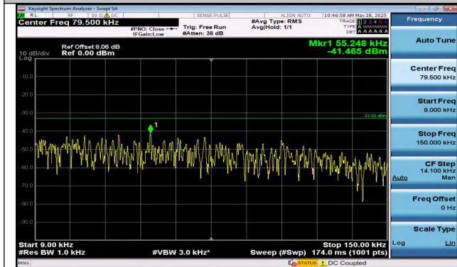
Band5-5MHz-QPSK-20525-1RB#0-0.009~0.15-PASS
