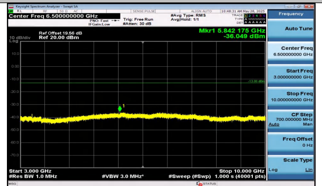
Band5-5MHz-16QAM-20525-1RB#0-3000~10000-PASS
