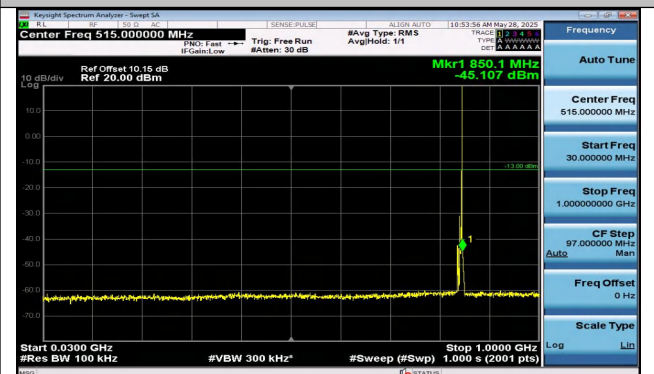
Band5-5MHz-QPSK-20625-1RB#24-30~1000-PASS
