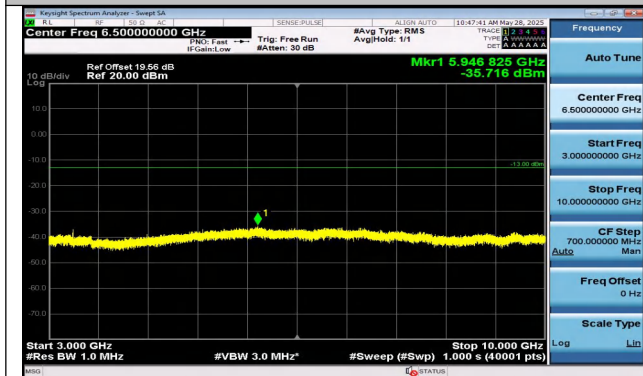
Band5-5MHz-QPSK-20525-1RB#0-3000~10000-PASS
