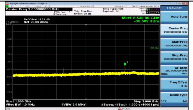
Band5-5MHz-QPSK-20625-1RB#0-1000~3000-PASS
