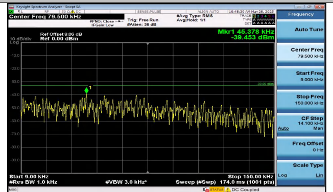
Band5-5MHz-QPSK-20525-1RB#24-0.009~0.15-PASS
