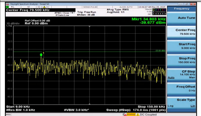
Band5-5MHz-16QAM-20425-25RB#0-0.009~0.15-PASS
