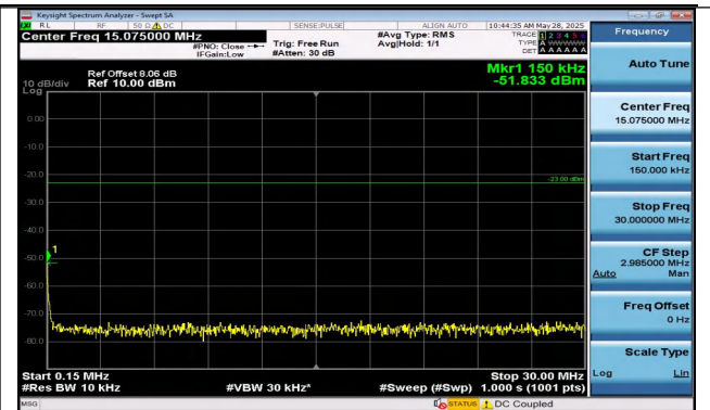
Band5-5MHz-16QAM-20425-1RB#24-0.15~30-PASS
