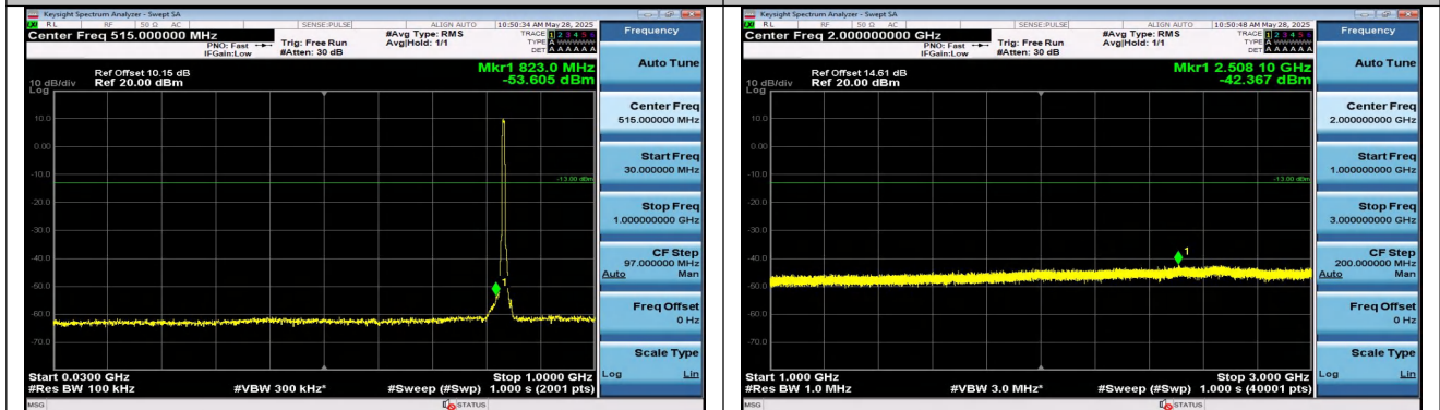
Band5-5MHz-QPSK-20525-25RB#0-30~1000-PASS
