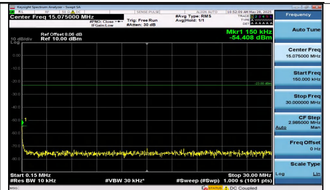
Band5-5MHz-QPSK-20625-1RB#0-0.15~30-PASS
