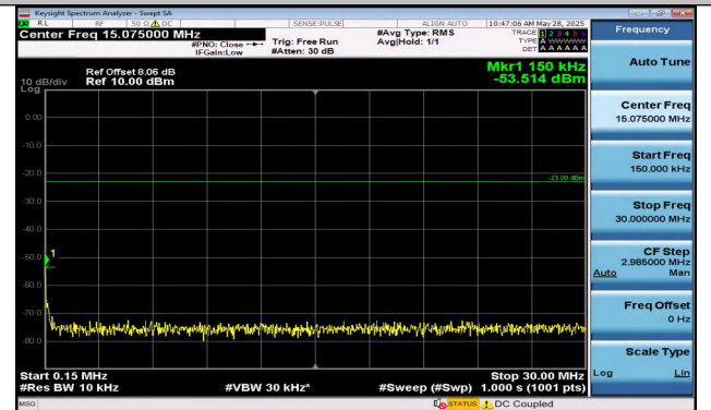
Band5-5MHz-QPSK-20525-1RB#0-0.15~30-PASS
