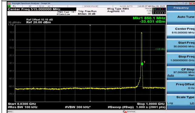
Band5-5MHz-QPSK-20625-25RB#0-30~1000-PASS
