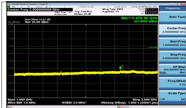
Band5-5MHz-16QAM-20425-25RB#0-1000~3000-PASS
