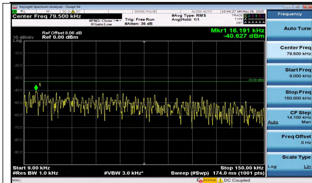
Band5-5MHz-16QAM-20425-1RB#24-0.009~0.15-PASS
