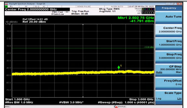
Band5-5MHz-QPSK-20525-1RB#0-1000~3000-PASS
