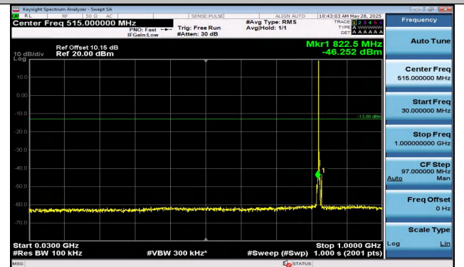
Band5-5MHz-16QAM-20425-1RB#0-0.009~0.15-PASS
