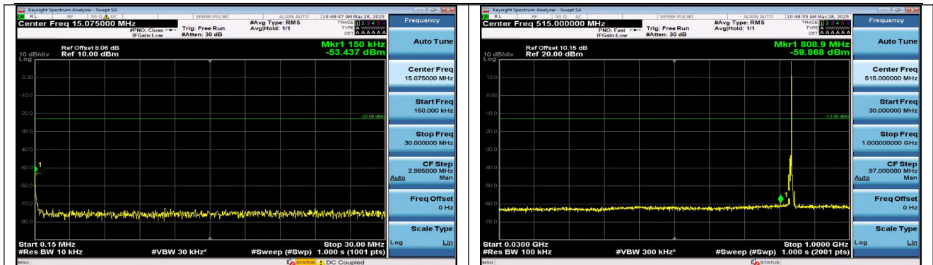
Band5-5MHz-QPSK-20525-1RB#24-0.15~30-PASS
