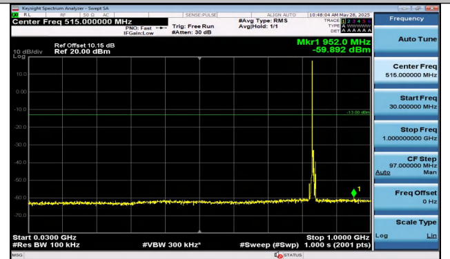
Band5-5MHz-16QAM-20525-1RB#0-30~1000-PASS
