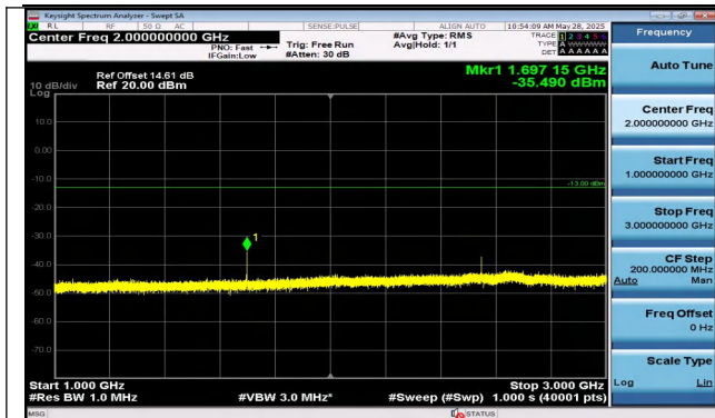
Band5-5MHz-QPSK-20625-1RB#24-1000~3000-PASS
