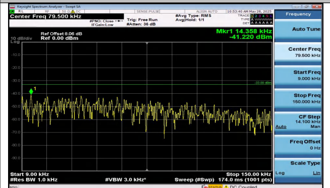
Band5-5MHz-QPSK-20625-1RB#24-0.009~0.15-PASS
