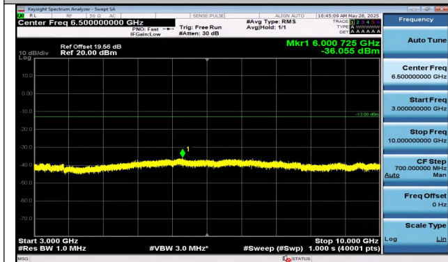
Band5-5MHz-16QAM-20425-1RB#24-3000~10000-PASS
