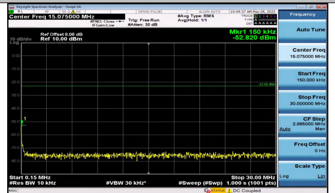
Band5-5MHz-16QAM-20525-1RB#24-0.15~30-PASS
