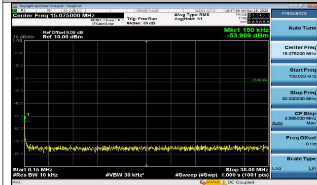
Band5-5MHz-16QAM-20525-1RB#0-0.15~30-PASS
