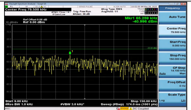
Band5-5MHz-16QAM-20625-1RB#0-0.009~0.15-PASS
