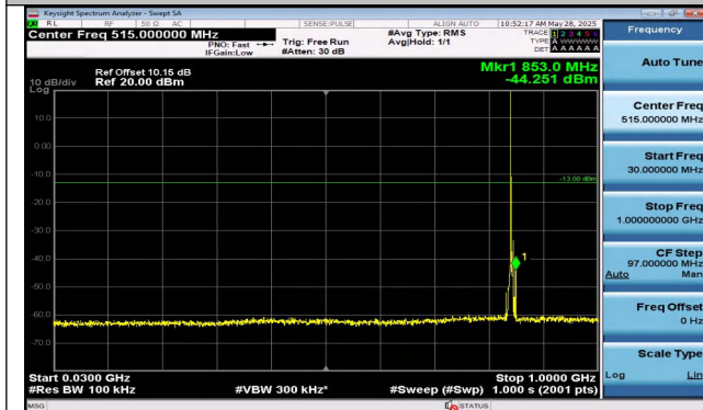
Band5-5MHz-QPSK-20625-1RB#0-30~1000-PASS
