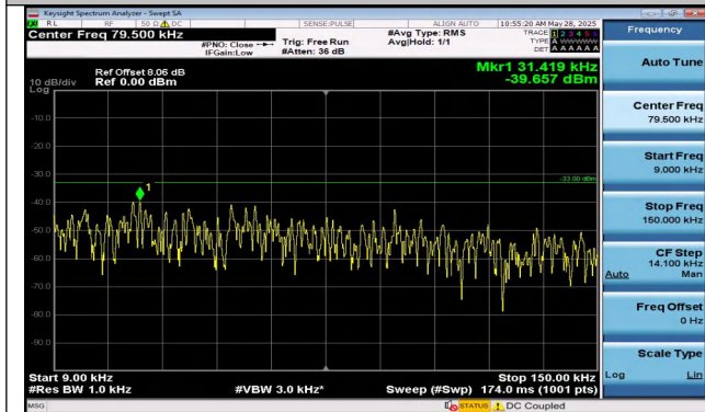
Band5-5MHz-QPSK-20625-25RB#0-0.009~0.15-PASS
