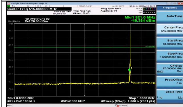
Band5-5MHz-16QAM-20425-1RB#24-30~1000-PASS
