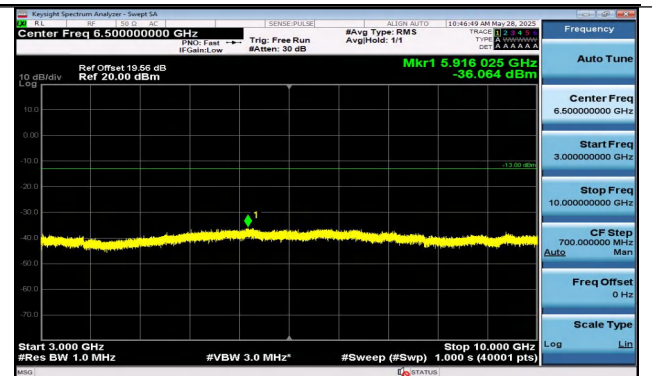
Band5-5MHz-16QAM-20425-25RB#0-3000~10000-PASS
