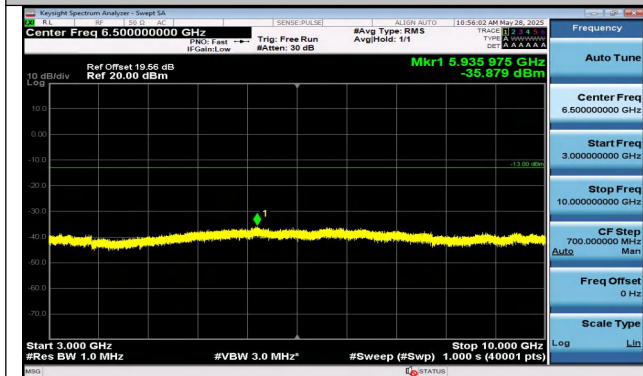
Band5-5MHz-QPSK-20625-25RB#0-3000~10000-PASS
