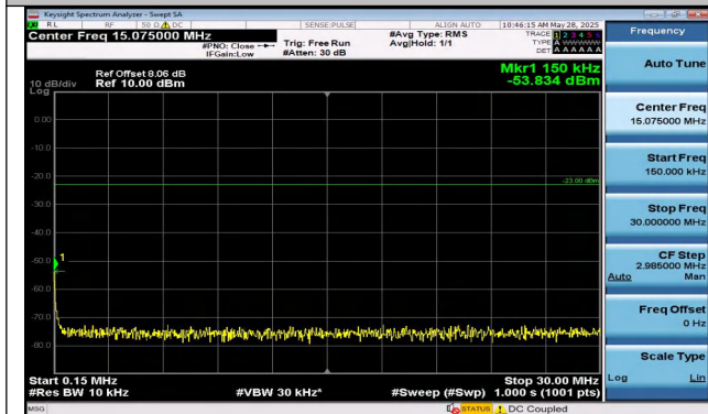
Band5-5MHz-16QAM-20425-25RB#0-0.15~30-PASS
