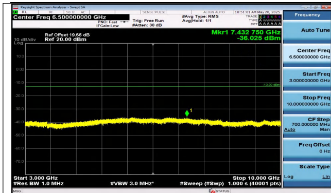
Band5-5MHz-QPSK-20525-25RB#0-3000~10000-PASS
