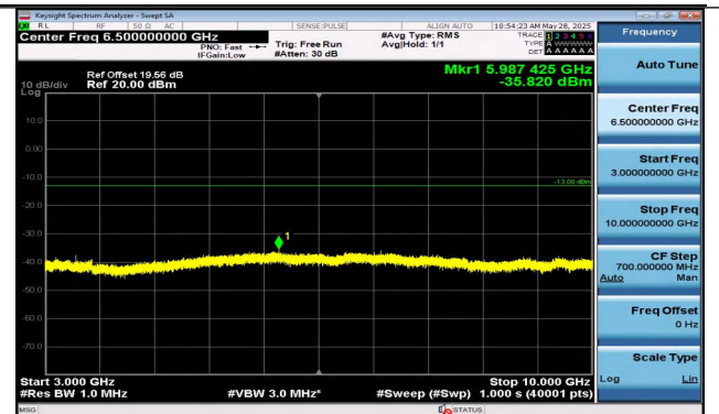
Band5-5MHz-QPSK-20625-1RB#24-3000~10000-PASS
