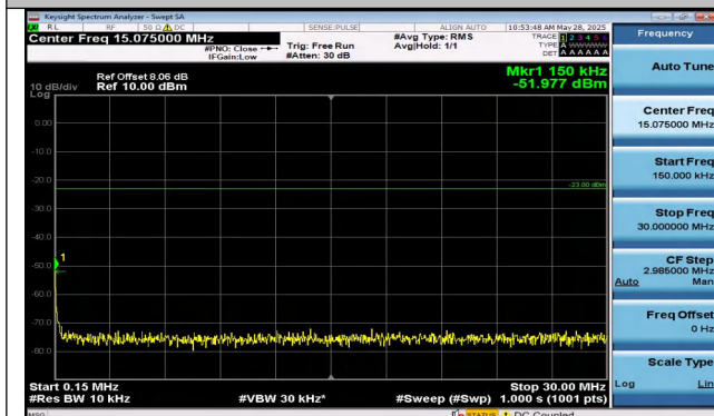
Band5-5MHz-QPSK-20625-1RB#24-0.15~30-PASS
