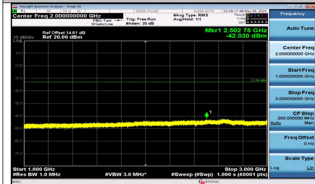
Band5-5MHz-16QAM-20525-1RB#0-1000~3000-PASS
