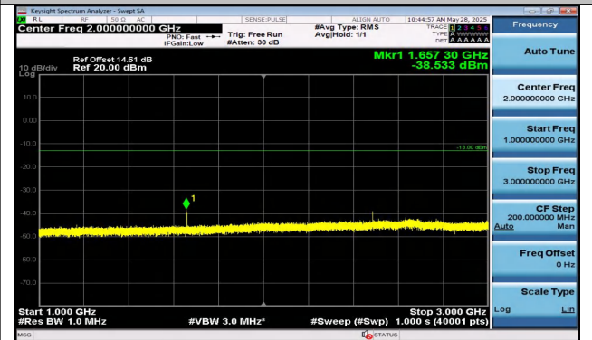
Band5-5MHz-16QAM-20425-1RB#24-1000~3000-PASS
