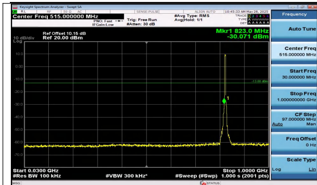
Band5-5MHz-QPSK-20425-25RB#0-30~1000-PASS
