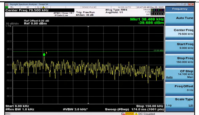
Band5-5MHz-16QAM-20525-1RB#0-0.009~0.15-PASS
