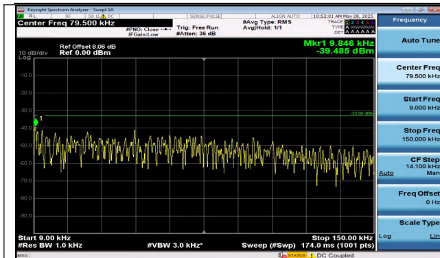
Band5-5MHz-QPSK-20625-1RB#0-0.009~0.15-PASS
