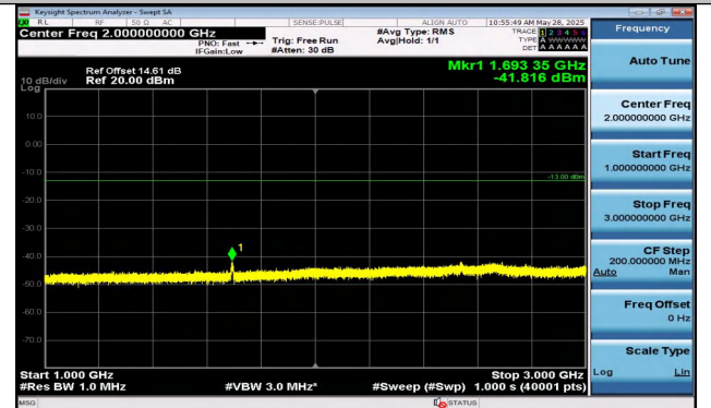
Band5-5MHz-QPSK-20625-25RB#0-1000~3000-PASS
