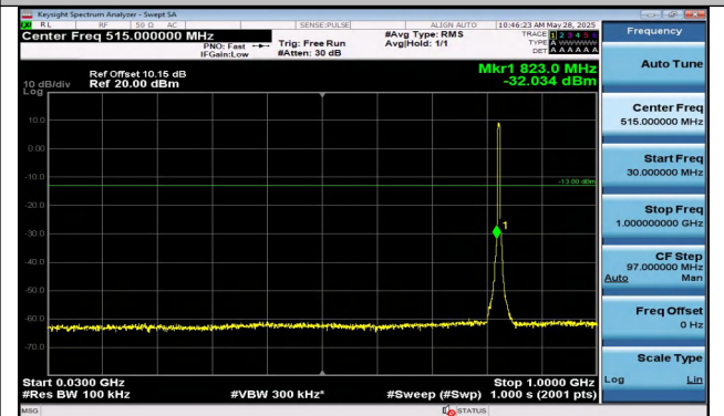
Band5-5MHz-16QAM-20425-25RB#0-30~1000-PASS
