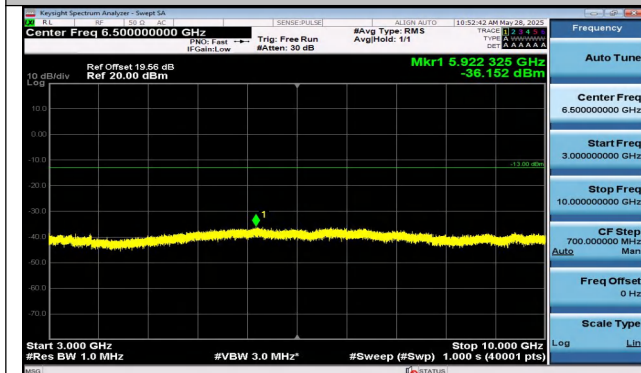
Band5-5MHz-QPSK-20625-1RB#0-3000~10000-PASS
