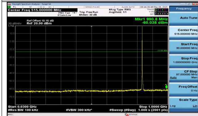
Band5-1.4MHz-16QAM-20525-1RB#5-30~1000-PASS
