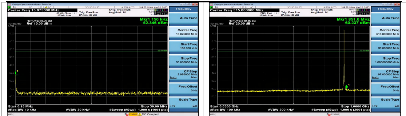
Band5-1.4MHz-16QAM-20525-6RB#0-0.15~30-PASS
