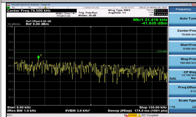
Band5-1.4MHz-QPSK-20407-6RB#0-0.009~0.15-PASS
