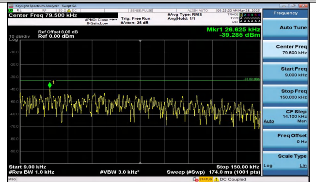
Band5-1.4MHz-QPSK-20525-1RB#5-0.009~0.15-PASS
