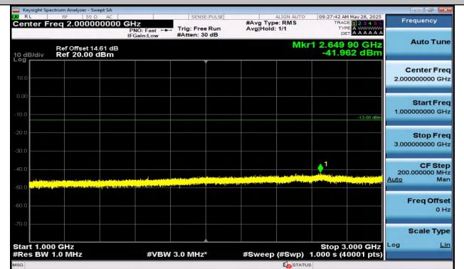
Band5-1.4MHz-QPSK-20525-6RB#0-1000~3000-PASS
