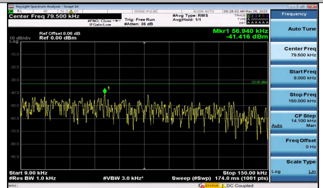
Band5-1.4MHz-16QAM-20525-6RB#0-0.009~0.15-PASS
