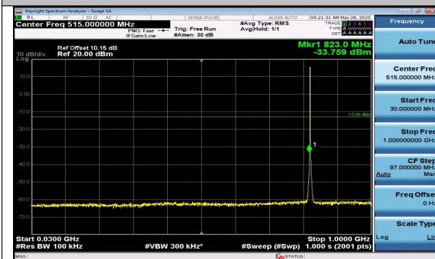
Band5-1.4MHz-QPSK-20407-6RB#0-30~1000-PASS
