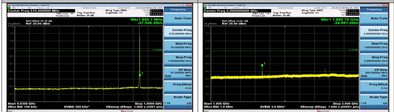
Band5-1.4MHz-QPSK-20643-1RB#0-30~1000-PASS
