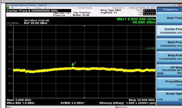
Band5-1.4MHz-QPSK-20407-6RB#0-3000~10000-PASS
