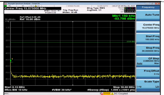
Band5-1.4MHz-QPSK-20525-6RB#0-0.15~30-PASS
