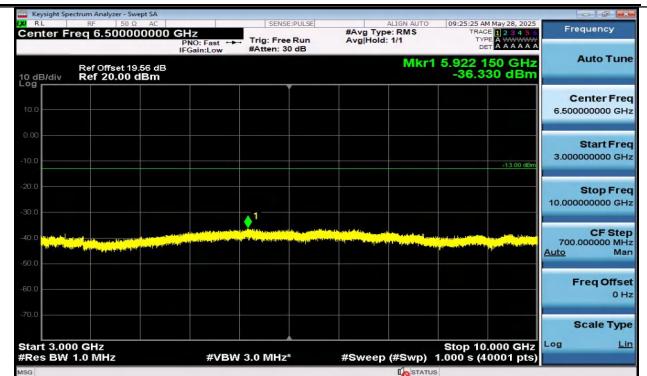
Band5-1.4MHz-16QAM-20525-1RB#0-3000~10000-PASS
