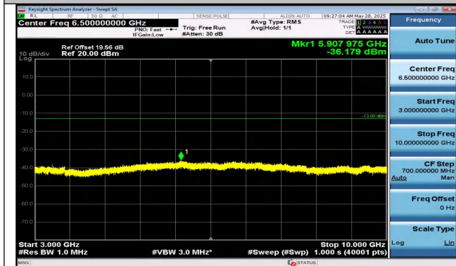
Band5-1.4MHz-16QAM-20525-1RB#5-3000~10000-PASS
