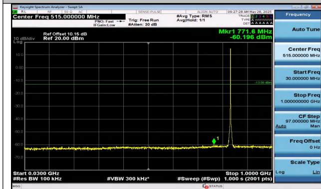
Band5-1.4MHz-QPSK-20525-6RB#0-30~1000-PASS
