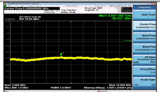
Band5-1.4MHz-QPSK-20525-1RB#5-3000~10000-PASS
