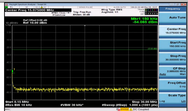
Band5-1.4MHz-QPSK-20407-6RB#0-0.15~30-PASS
