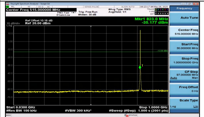
Band5-1.4MHz-16QAM-20407-6RB#0-30~1000-PASS
