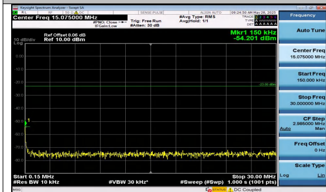
Band5-1.4MHz-16QAM-20525-1RB#0-0.15~30-PASS
