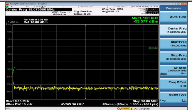
Band5-1.4MHz-QPSK-20525-1RB#0-0.15~30-PASS
