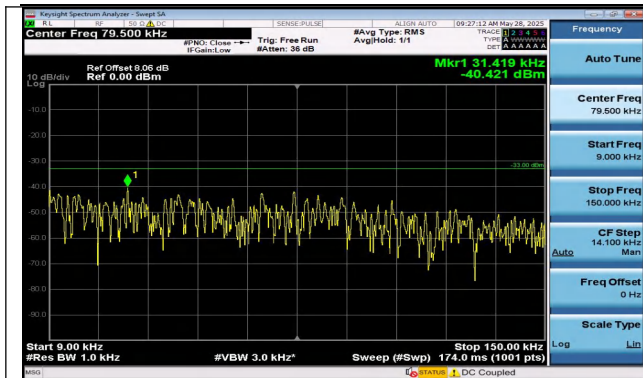
Band5-1.4MHz-QPSK-20525-6RB#0-0.009~0.15-PASS
