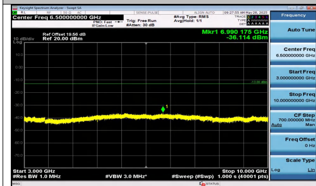
Band5-1.4MHz-QPSK-20525-6RB#0-3000~10000-PASS
