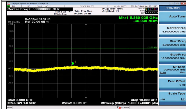
Band5-1.4MHz-QPSK-20525-1RB#0-3000~10000-PASS
