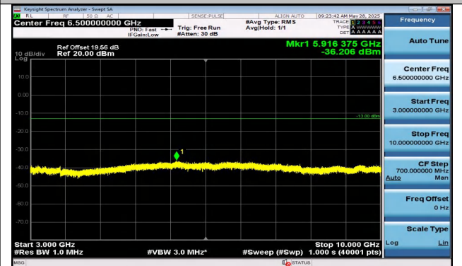
Band5-1.4MHz-16QAM-20407-6RB#0-3000~10000-PASS
