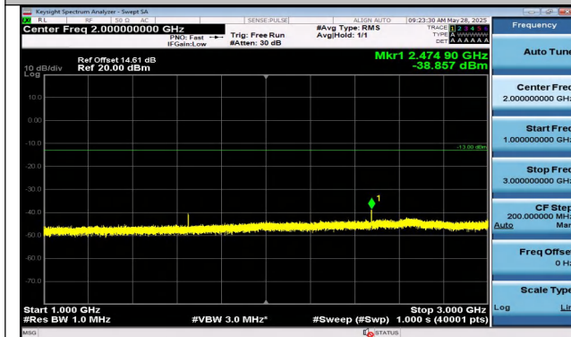
Band5-1.4MHz-16QAM-20407-6RB#0-1000~3000-PASS
