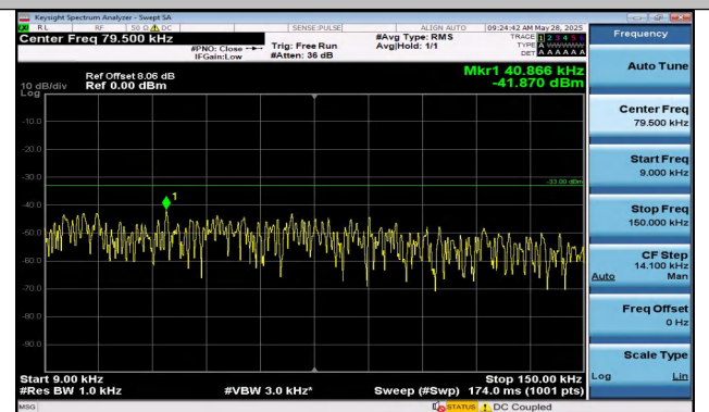
Band5-1.4MHz-16QAM-20525-1RB#0-0.009~0.15-PASS
