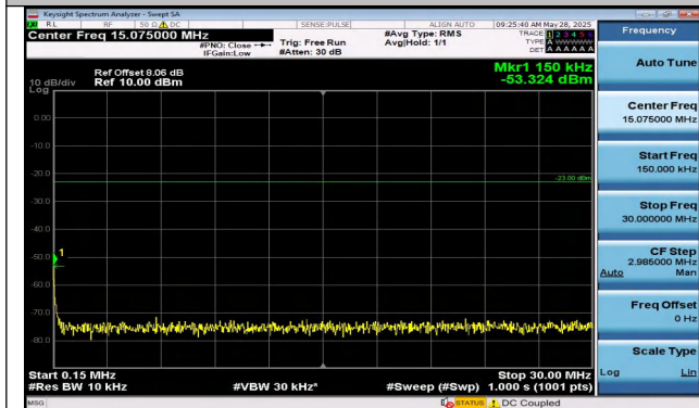
Band5-1.4MHz-QPSK-20525-1RB#5-0.15~30-PASS
