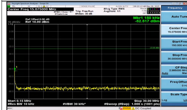
Band5-1.4MHz-16QAM-20407-6RB#0-0.15~30-PASS
