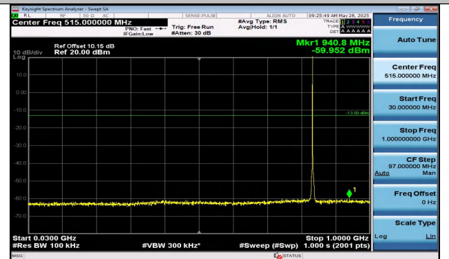
Band5-1.4MHz-QPSK-20525-1RB#5-30~1000-PASS
