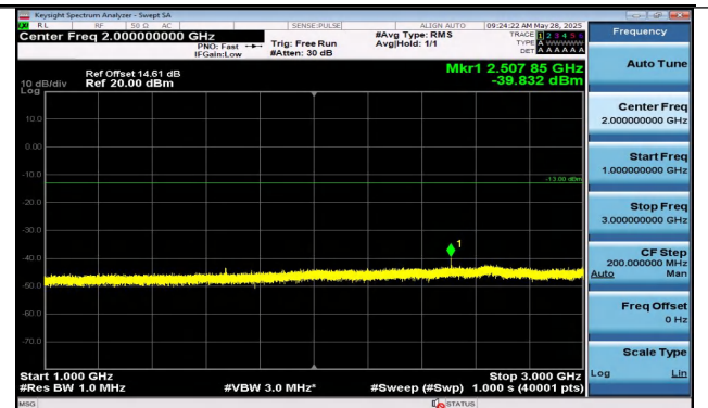
Band5-1.4MHz-QPSK-20525-1RB#0-1000~3000-PASS
