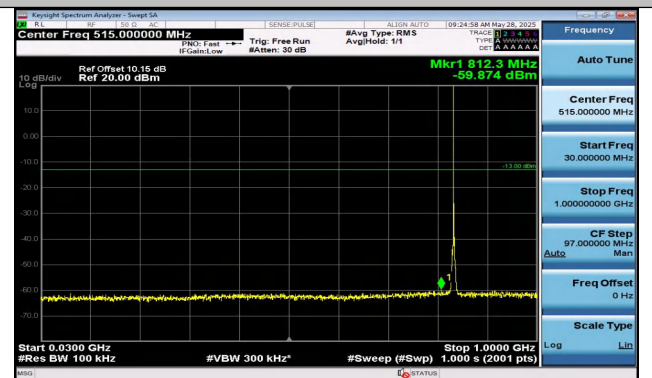
Band5-1.4MHz-16QAM-20525-1RB#0-30~1000-PASS
