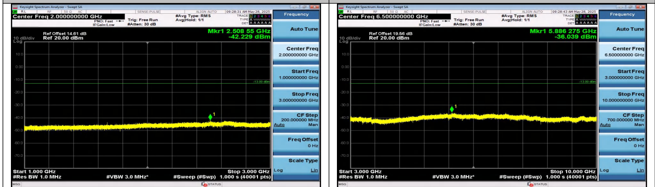
Band5-1.4MHz-16QAM-20525-6RB#0-1000~3000-PASS
