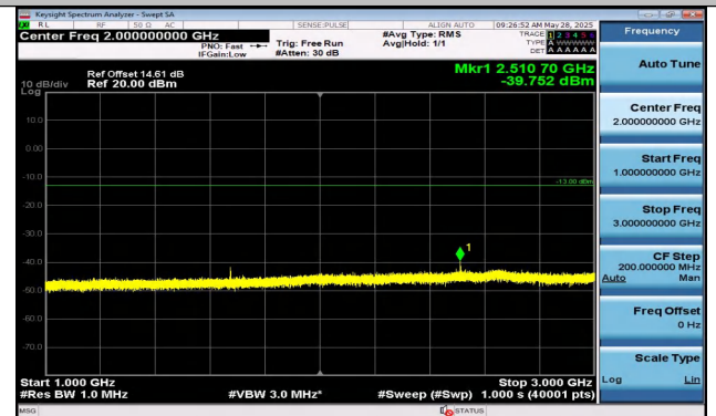
Band5-1.4MHz-16QAM-20525-1RB#5-1000~3000-PASS
