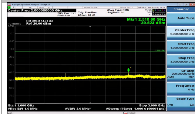
Band5-1.4MHz-QPSK-20525-1RB#5-1000~3000-PASS
