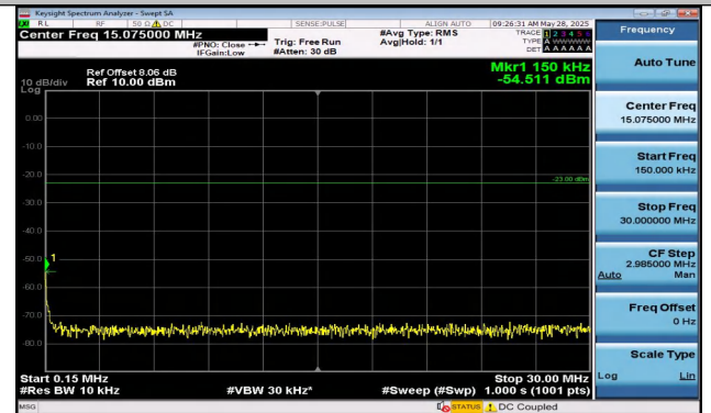
Band5-1.4MHz-16QAM-20525-1RB#5-0.15~30-PASS
