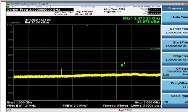
Band5-1.4MHz-QPSK-20407-1RB#5-1000~3000-PASS
