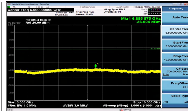
Band5-1.4MHz-16QAM-20407-1RB#5-3000~10000-PASS
