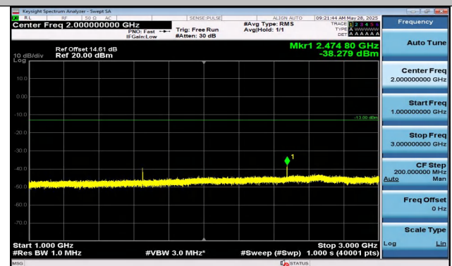
Band5-1.4MHz-QPSK-20407-6RB#0-1000~3000-PASS
