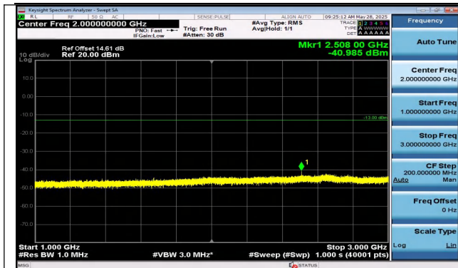
Band5-1.4MHz-16QAM-20525-1RB#0-1000~3000-PASS
