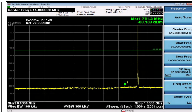
Band5-1.4MHz-QPSK-20525-1RB#0-30~1000-PASS
