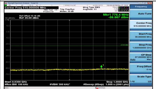
Band4-1.4MHz-QPSK-19957-1RB#5-30~1000-PASS
