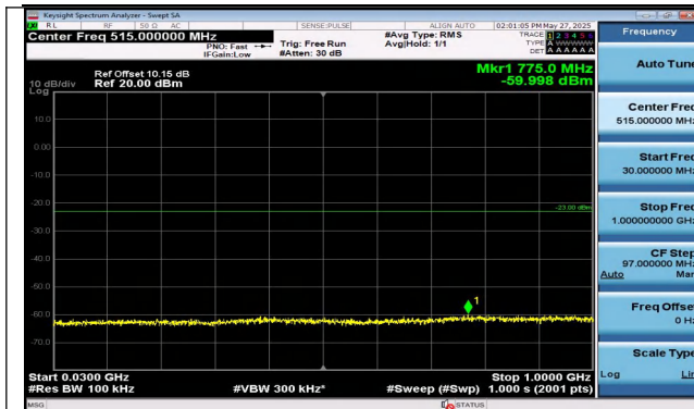
Band4-1.4MHz-QPSK-19957-1RB#0-30~1000-PASS
