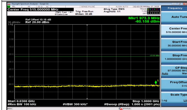
Band4-1.4MHz-16QAM-19957-1RB#5-30~1000-PASS
