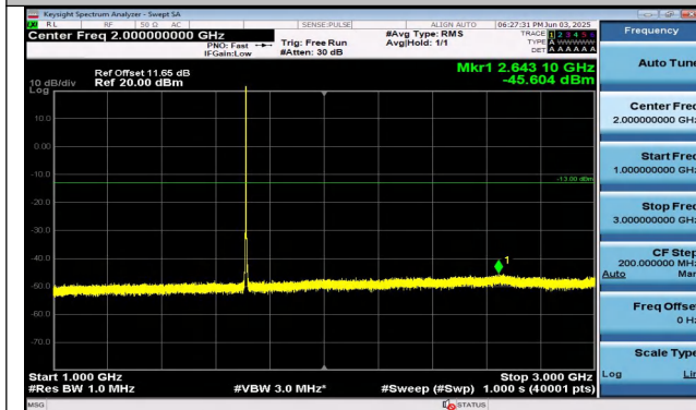
Band4-1.4MHz-QPSK-19957-1RB#5-1000~3000-PASS
