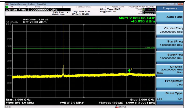
Band4-1.4MHz-QPSK-19957-1RB#0-1000~3000-PASS
