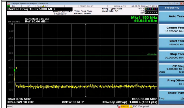
Band4-1.4MHz-QPSK-20175-1RB#5-0.15~30-PASS
