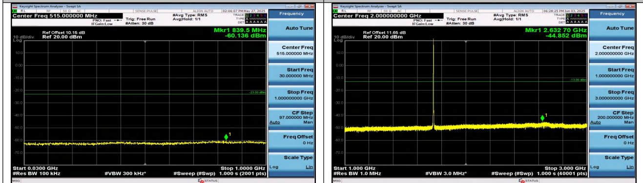
Band4-1.4MHz-QPSK-20175-1RB#0-30~1000-PASS
