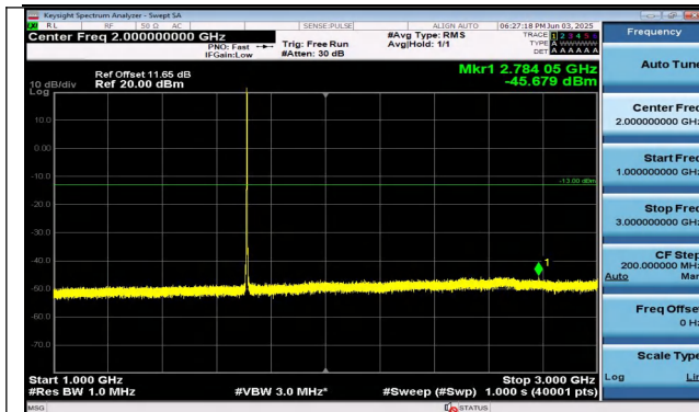
Band4-1.4MHz-16QAM-19957-1RB#0-1000~3000-PASS
