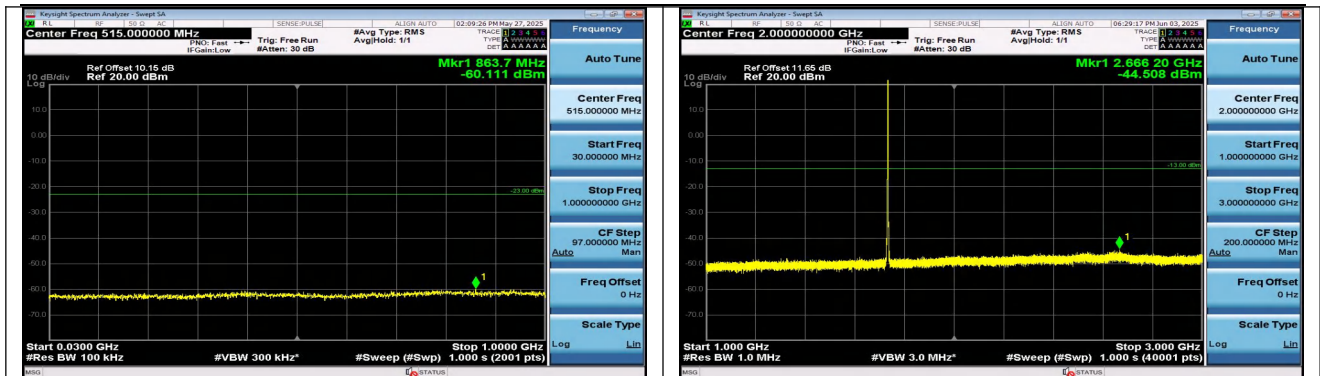
Band4-1.4MHz-QPSK-20175-6RB#0-30~1000-PASS
