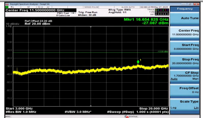
Band4-1.4MHz-QPSK-20175-1RB#5-3000~20000-PASS
