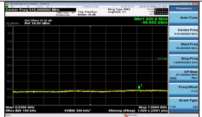
Band4-1.4MHz-QPSK-20175-1RB#5-30~1000-PASS
