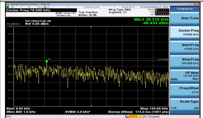
Band4-1.4MHz-16QAM-19957-6RB#0-0.009~0.15-PASS
