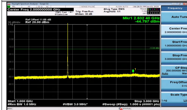
Band4-1.4MHz-QPSK-20175-1RB#5-1000~3000-PASS
