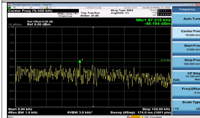
Band4-1.4MHz-QPSK-20175-6RB#0-0.009~0.15-PASS
