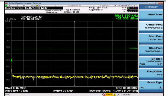
Band4-1.4MHz-16QAM-19957-1RB#5-0.15~30-PASS
