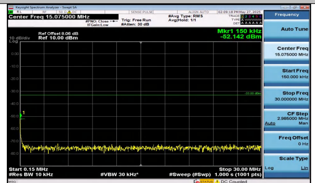
Band4-1.4MHz-QPSK-20175-6RB#0-0.15~30-PASS
