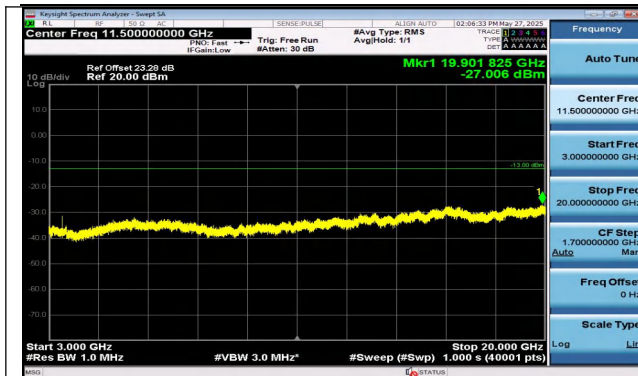
Band4-1.4MHz-QPSK-20175-1RB#0-3000~20000-PASS
