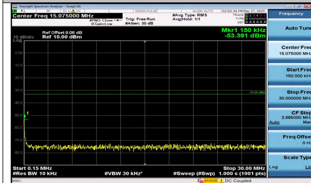
Band4-1.4MHz-QPSK-19957-1RB#5-0.15~30-PASS
