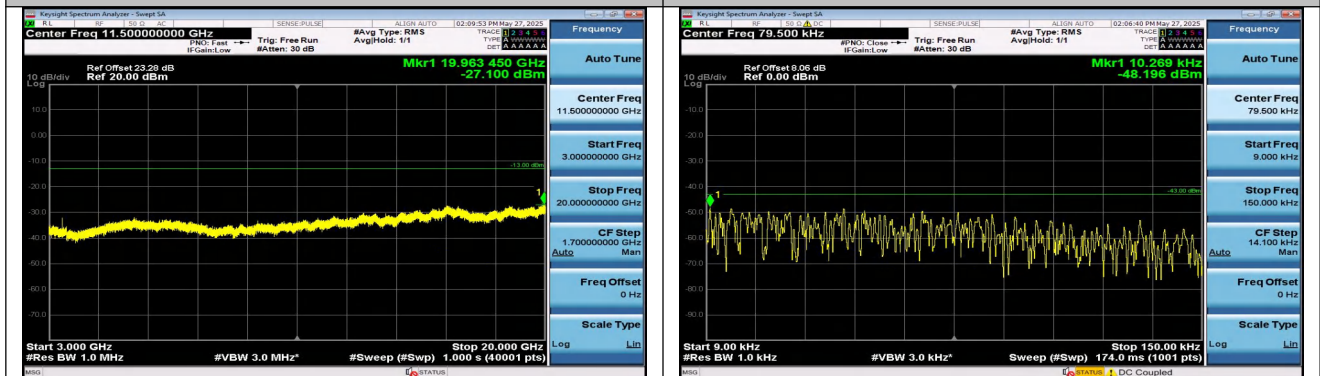
Band4-1.4MHz-QPSK-20175-6RB#0-3000~20000-PASS
