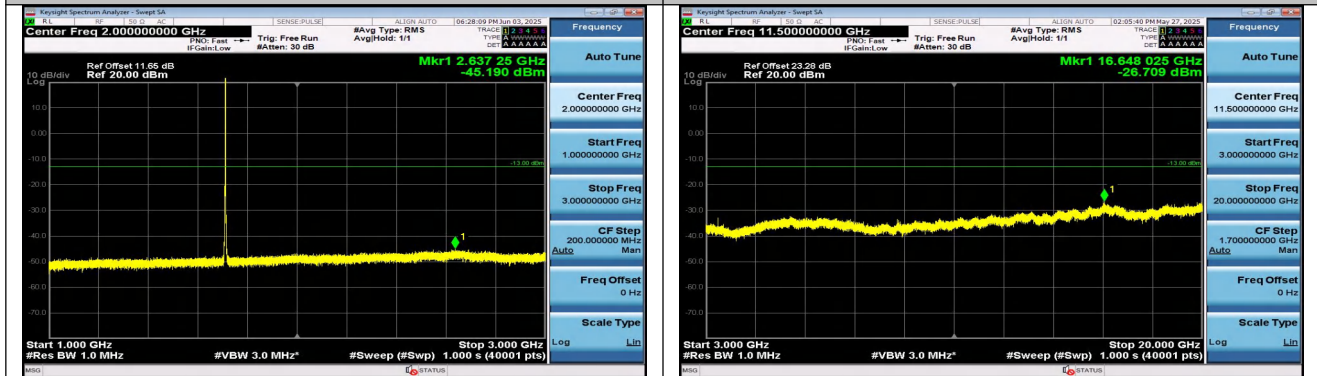
Band4-1.4MHz-16QAM-19957-6RB#0-1000~3000-PASS
