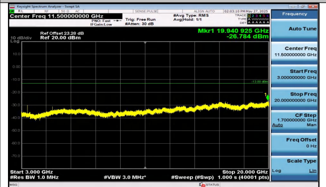
Band4-1.4MHz-QPSK-19957-1RB#5-3000~20000-PASS
