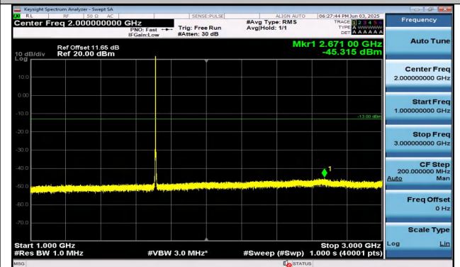
Band4-1.4MHz-16QAM-19957-1RB#5-1000~3000-PASS
