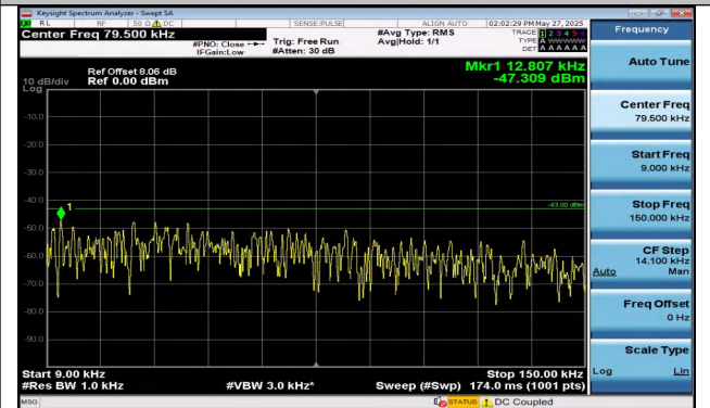
Band4-1.4MHz-QPSK-19957-1RB#5-0.009~0.15-PASS
