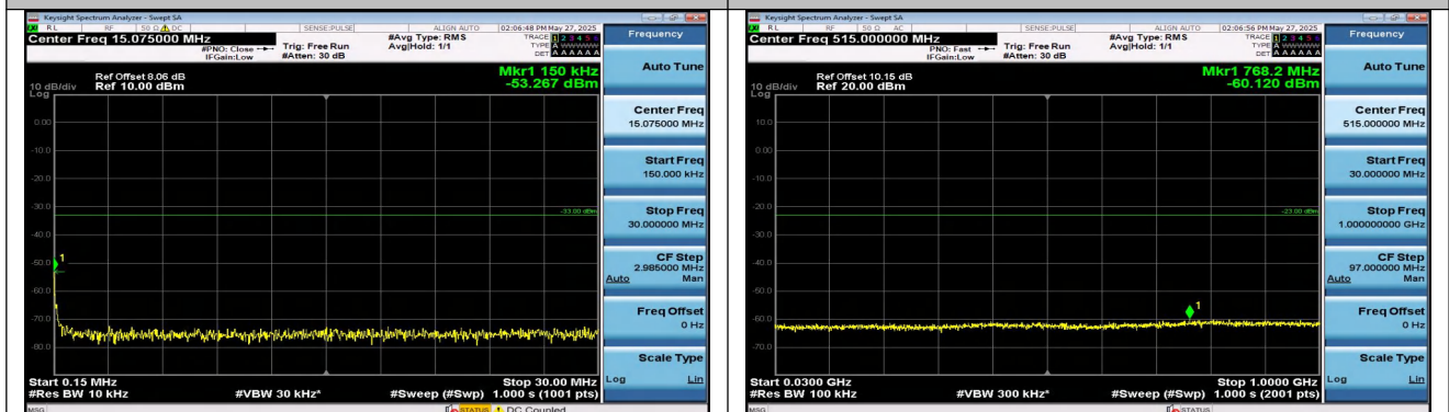
Band4-1.4MHz-16QAM-20175-1RB#0-0.15~30-PASS
