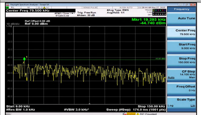
Band2-15MHz-QPSK-18675-1RB#0-0.009~0.15-PASS
