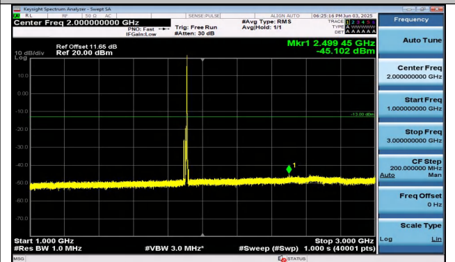
Band2-10MHz-16QAM-19150-1RB#49-1000~3000-PASS
