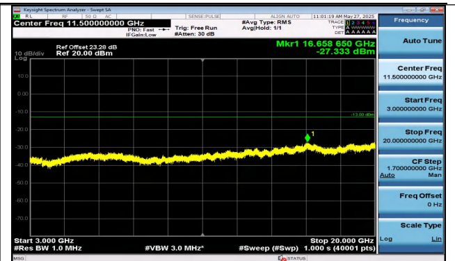
Band2-10MHz-16QAM-19150-1RB#0-3000~20000-PASS
