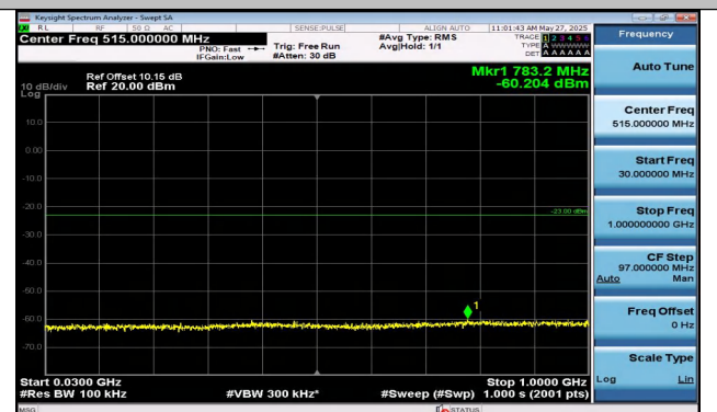
Band2-10MHz-QPSK-19150-1RB#49-30~1000-PASS
