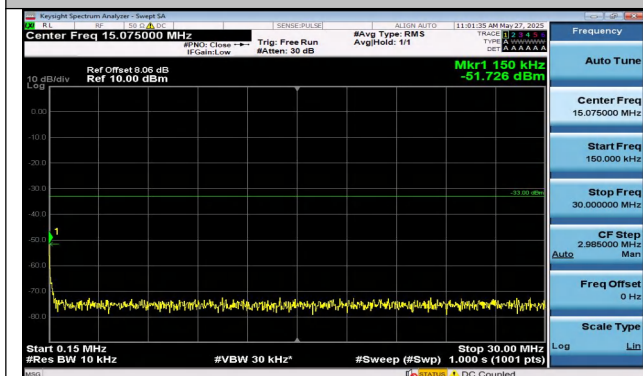
Band2-10MHz-QPSK-19150-1RB#49-0.15~30-PASS
