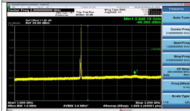
Band2-10MHz-QPSK-19150-1RB#49-1000~3000-PASS
