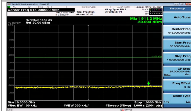
Band2-15MHz-QPSK-18900-1RB#0-30~1000-PASS
