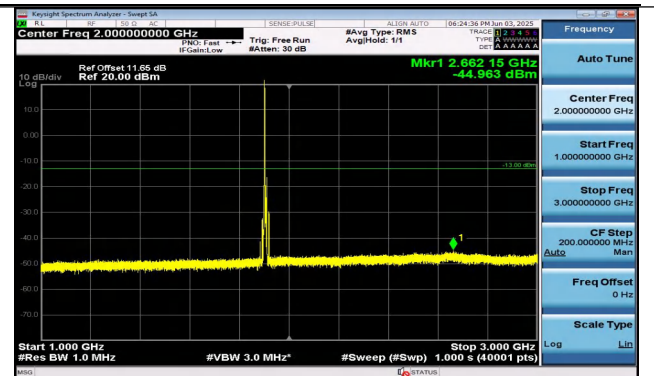
Band2-10MHz-QPSK-19150-1RB#0-1000~3000-PASS
