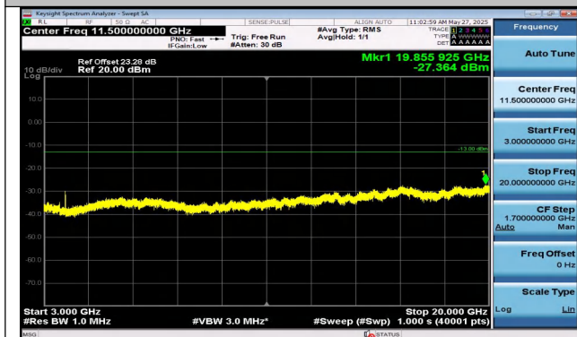
Band2-10MHz-16QAM-19150-1RB#49-3000~20000-PASS
