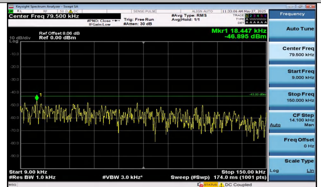
Band2-15MHz-16QAM-18900-1RB#0-0.009~0.15-PASS
