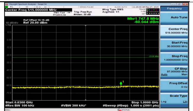
Band2-15MHz-QPSK-18675-1RB#0-30~1000-PASS
