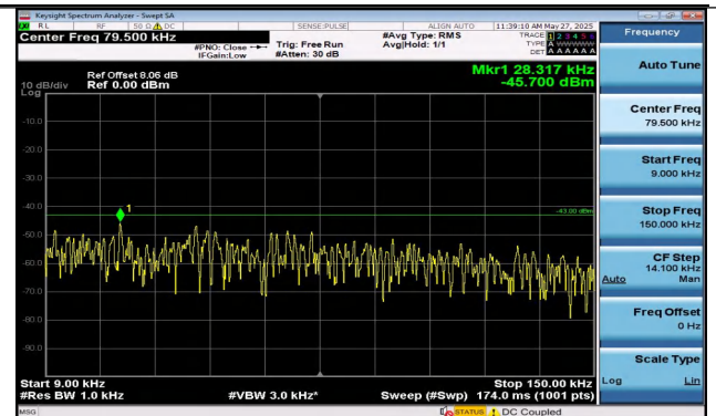
Band2-15MHz-QPSK-18675-75RB#0-0.009~0.15-PASS
