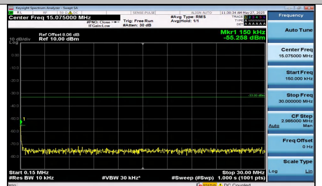
Band2-15MHz-QPSK-18675-1RB#74-0.15~30-PASS
