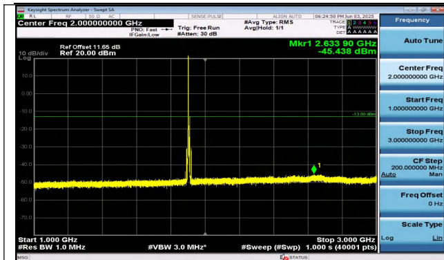
Band2-10MHz-16QAM-19150-1RB#0-1000~3000-PASS
