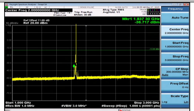
Band2-15MHz-QPSK-18675-1RB#74-1000~3000-PASS
