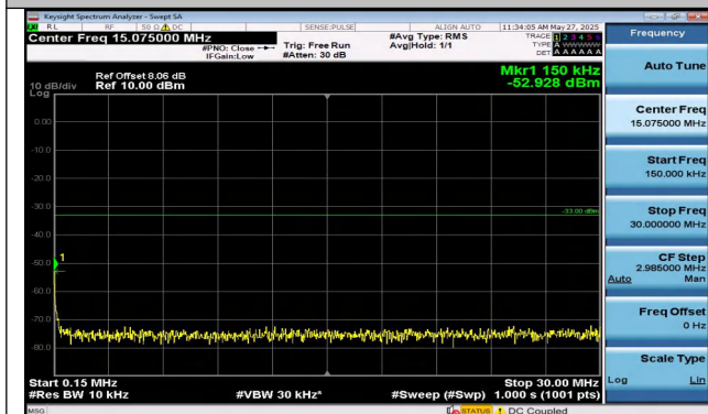
Band2-15MHz-QPSK-18900-1RB#74-0.15~30-PASS
