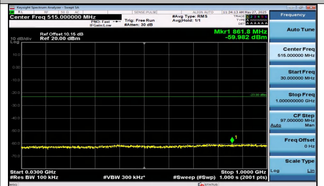
Band2-15MHz-QPSK-18900-1RB#74-30~1000-PASS
