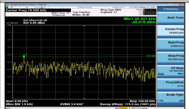
Band2-15MHz-QPSK-18900-1RB#74-0.009~0.15-PASS
