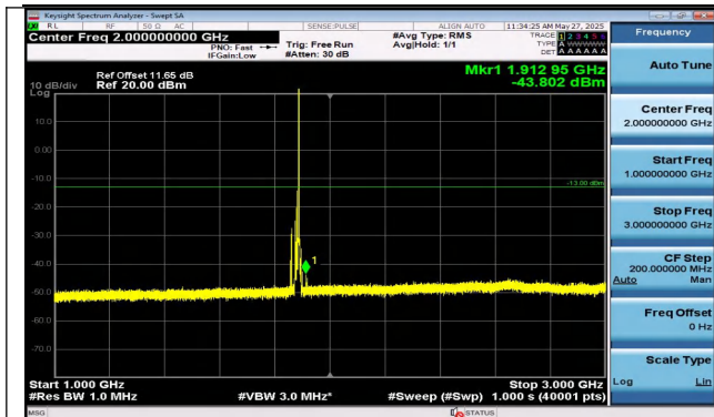
Band2-15MHz-QPSK-18900-1RB#74-1000~3000-PASS
