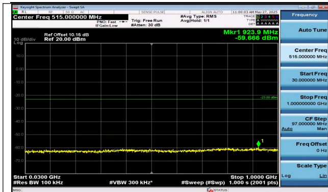
Band2-10MHz-QPSK-19150-1RB#0-30~1000-PASS
