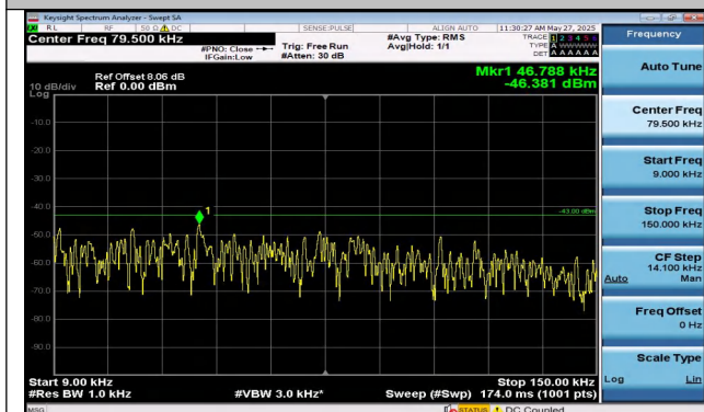
Band2-15MHz-QPSK-18675-1RB#74-0.009~0.15-PASS
