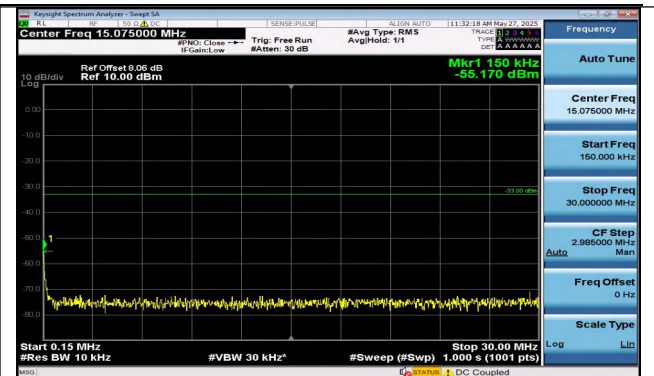
Band2-15MHz-QPSK-18900-1RB#0-0.15~30-PASS
