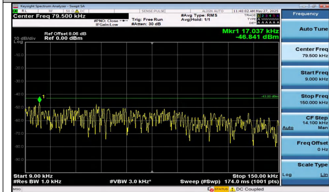
Band2-15MHz-QPSK-18900-75RB#0-0.009~0.15-PASS
