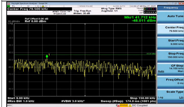
Band2-10MHz-16QAM-19150-1RB#49-0.009~0.15-PASS
