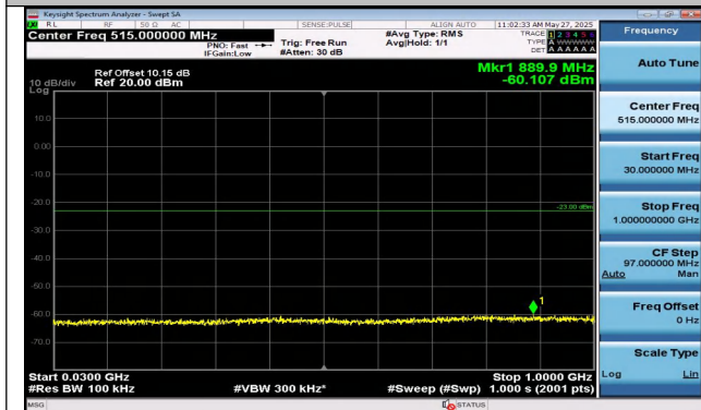
Band2-10MHz-16QAM-19150-1RB#49-30~1000-PASS
