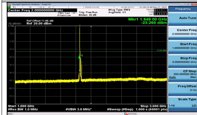
Band2-15MHz-QPSK-18675-1RB#0-1000~3000-PASS
