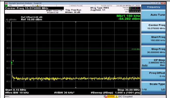
Band2-10MHz-16QAM-19150-1RB#49-0.15~30-PASS
