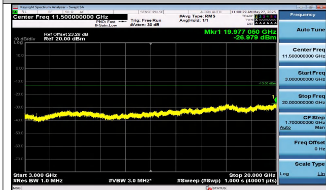
Band2-10MHz-QPSK-19150-1RB#0-3000~20000-PASS
