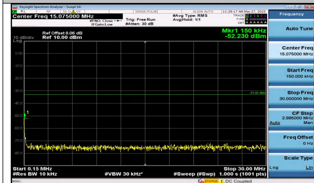
Band2-15MHz-QPSK-18675-1RB#74-3000~20000-PASS
