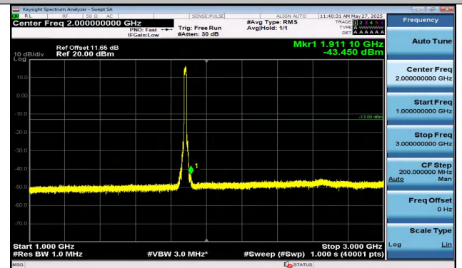
Band2-15MHz-QPSK-18900-75RB#0-1000~3000-PASS
