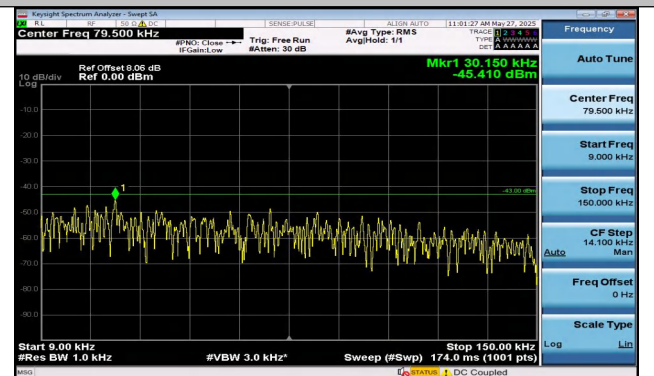
Band2-10MHz-QPSK-19150-1RB#49-0.009~0.15-PASS
