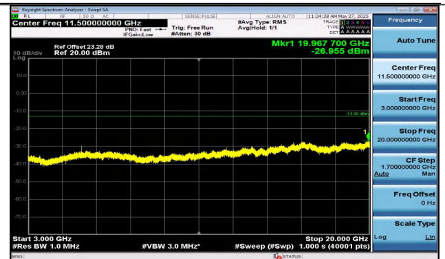
Band2-15MHz-QPSK-18900-1RB#74-3000~20000-PASS
