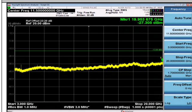
Band2-15MHz-QPSK-18900-1RB#0-3000~20000-PASS
