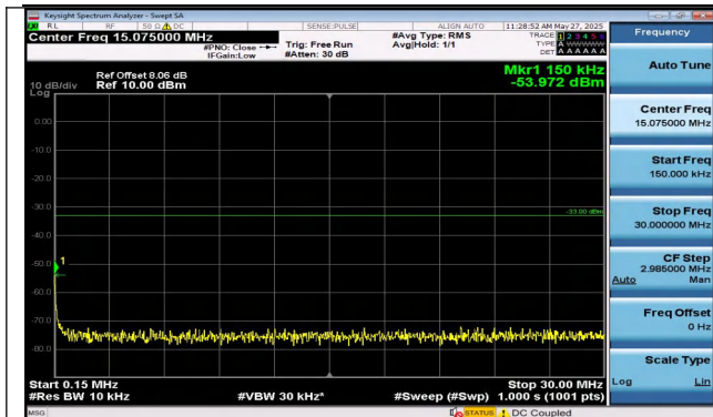
Band2-15MHz-QPSK-18675-1RB#0-0.15~30-PASS
