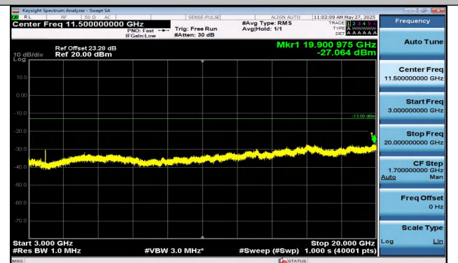
Band2-10MHz-QPSK-19150-1RB#49-3000~20000-PASS
