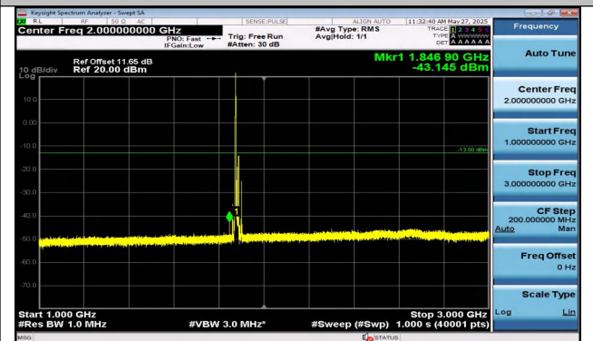
Band2-15MHz-QPSK-18900-1RB#0-1000~3000-PASS
