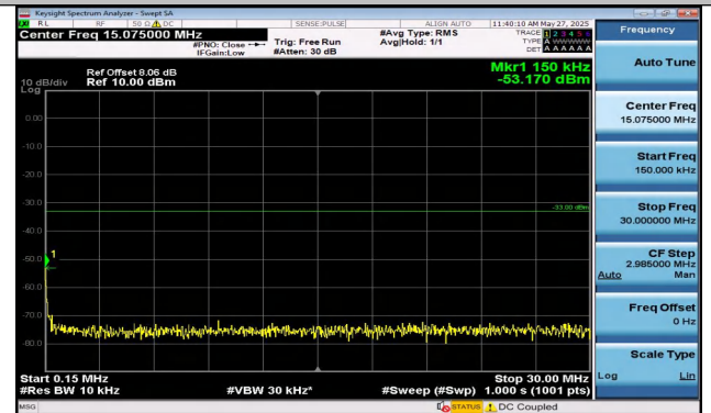
Band2-15MHz-QPSK-18900-75RB#0-0.15~30-PASS
