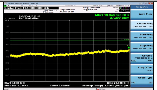
Band2-15MHz-QPSK-18675-1RB#0-3000~20000-PASS
