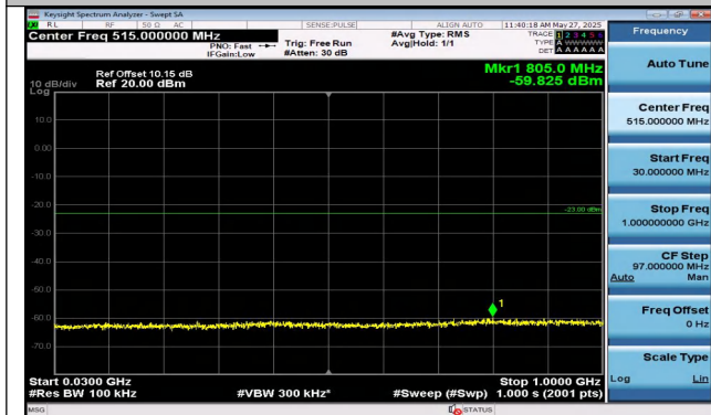
Band2-15MHz-QPSK-18900-75RB#0-30~1000-PASS
