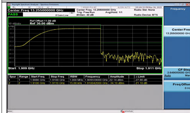
Band2-1.4MHz-16QAM-19193-1RB#5-PASS
