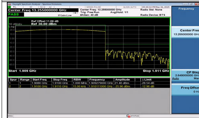
Band2-1.4MHz-QPSK-19193-6RB#0-PASS
