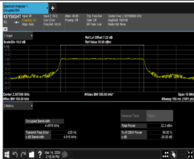
Band40-5MHz-16QAM-38750-25RB#0
