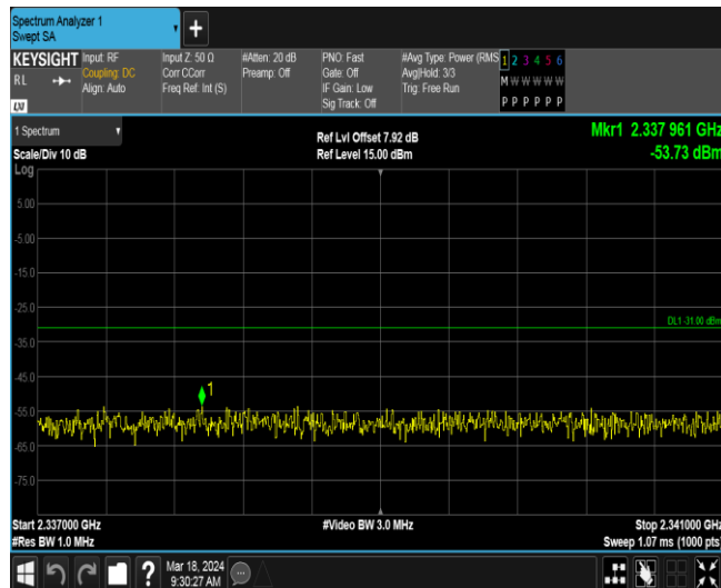
Band40-5MHz-QPSK-38725-1RB#0-Range11:2341~2345MHz
