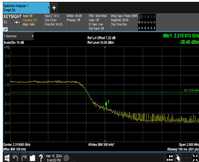
Band40-5MHz-16QAM-38725-1RB#0
