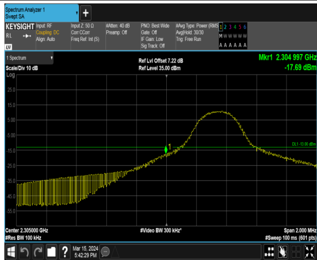
Band40-5MHz-16QAM-38725-1RB#24
