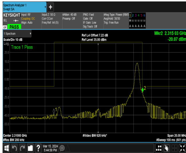
Band40-10MHz-16QAM-38750-50RB#0
