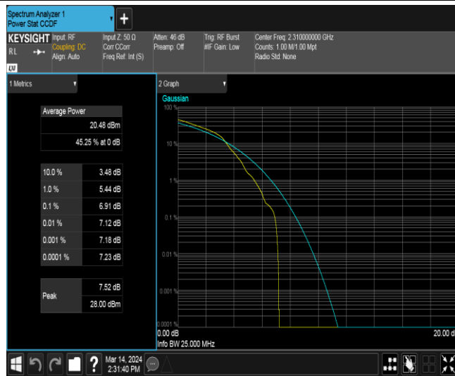
Band40-5MHz-16QAM-38750-25RB#0
