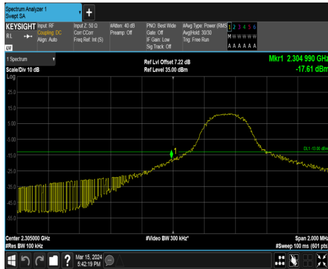
Band40-5MHz-QPSK-38725-1RB#24
