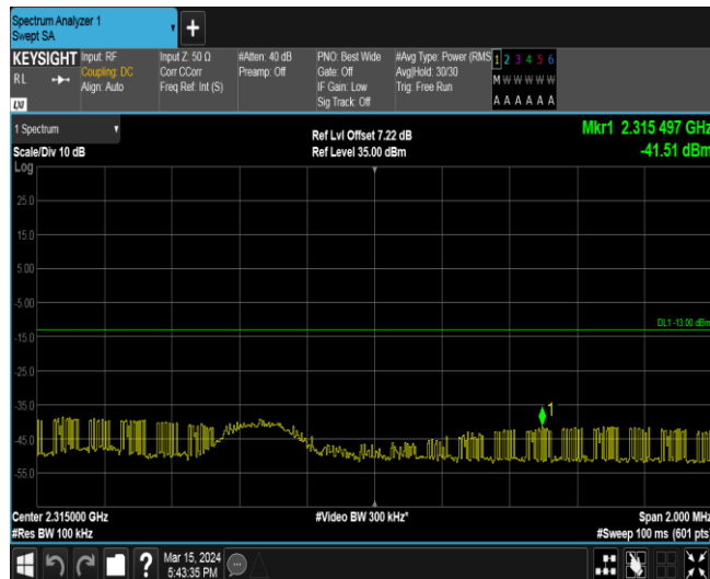
Band40-5MHz-16QAM-38775-1RB#24
