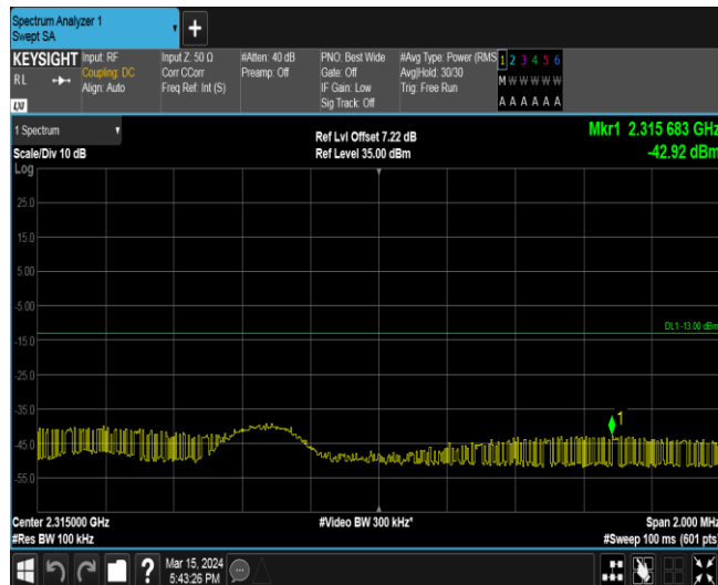
Band40-5MHz-QPSK-38775-1RB#24
