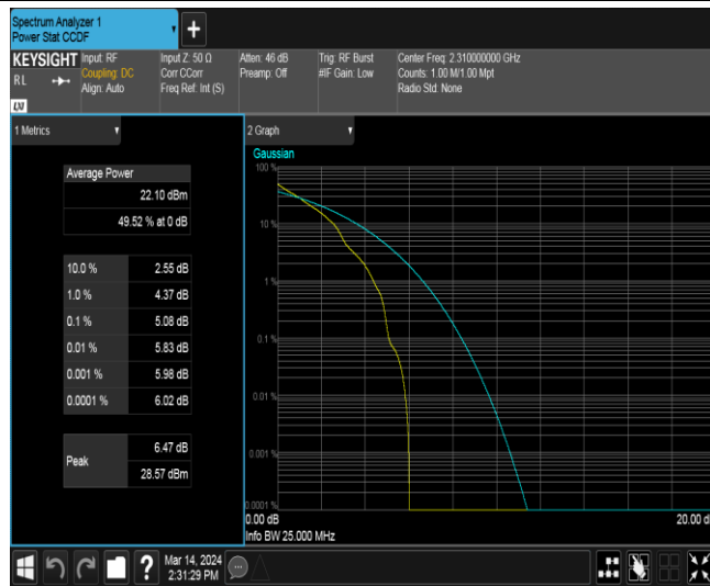
Band40-5MHz-QPSK-38750-25RB#0
