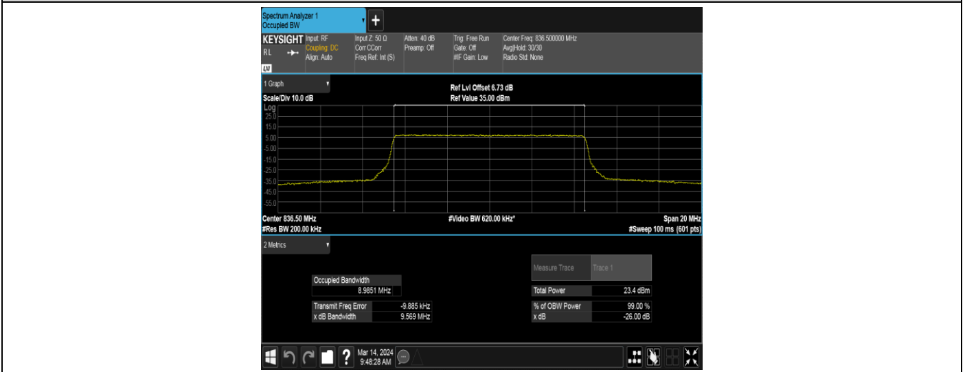
Band5-10MHz-QPSK-20600-50RB#0
