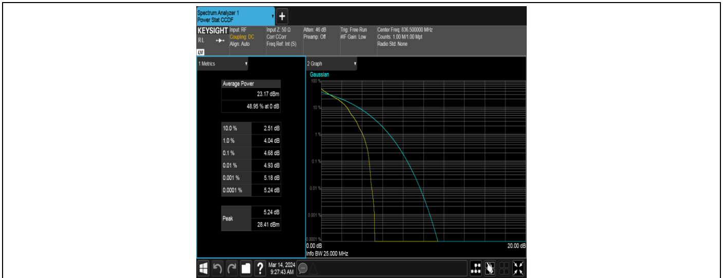
Band5-3MHz-QPSK-20525-15RB#0
