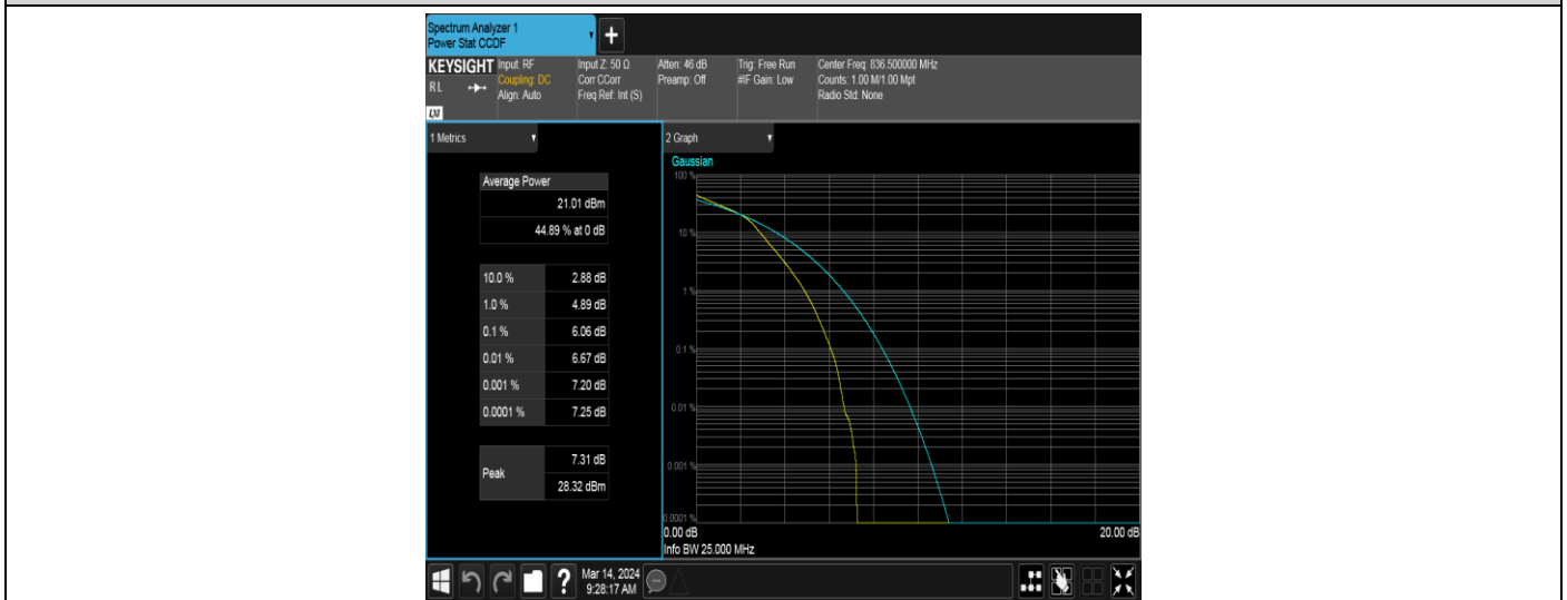
Band5-3MHz-16QAM-20635-1RB#0
