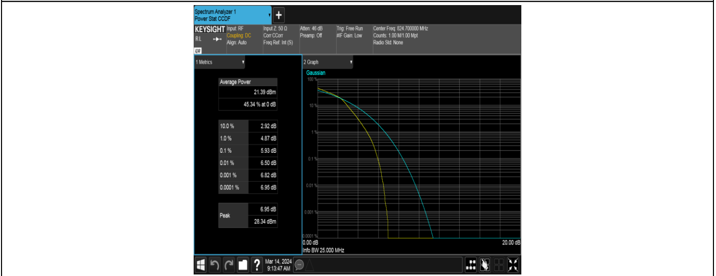
Band5-1.4MHz-16QAM-20525-1RB#0
