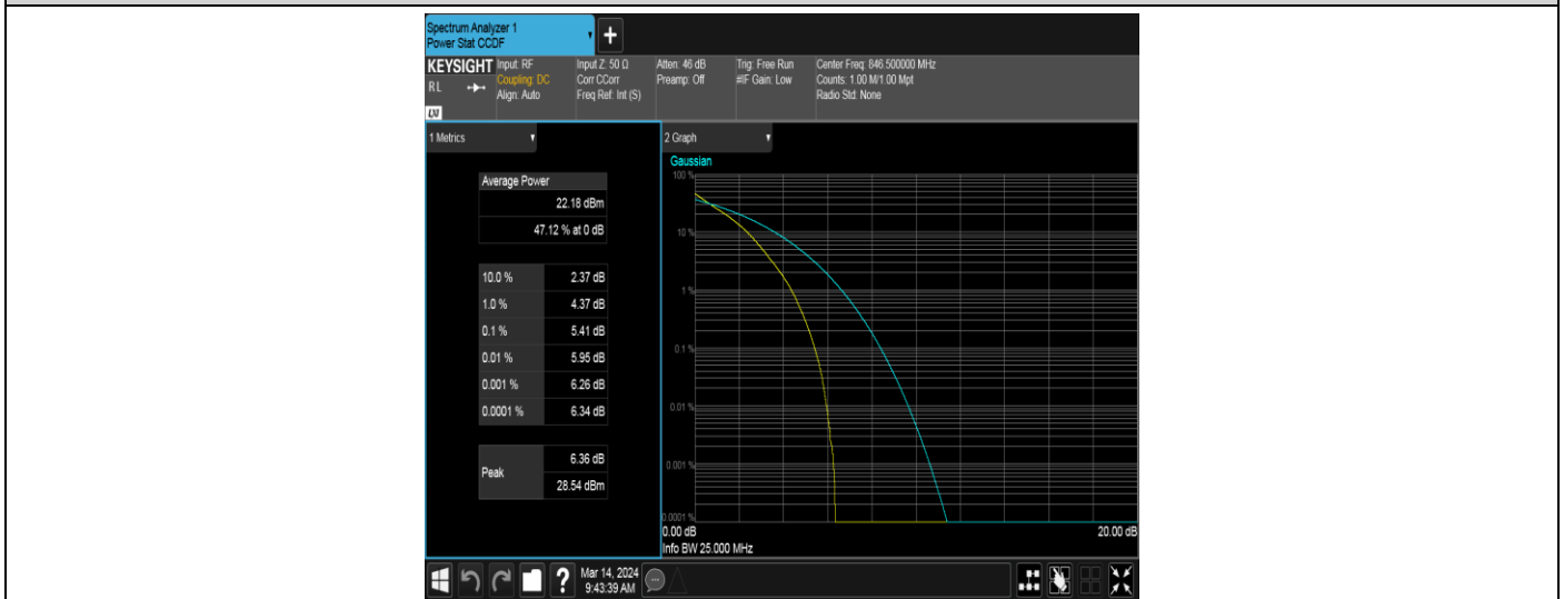
Band5-5MHz-16QAM-20425-1RB#0
