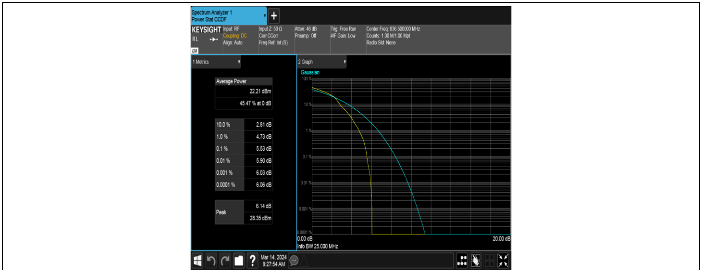
Band5-3MHz-16QAM-20525-15RB#0
