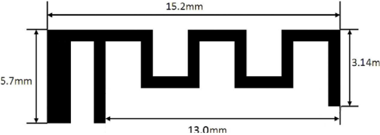
Antenna Photo & Length (mm)
