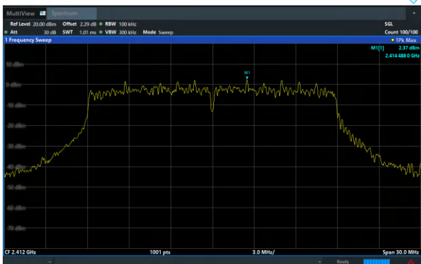
802.11n20 on Channel 01
