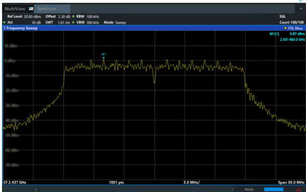
802.11n20 on Channel 06
