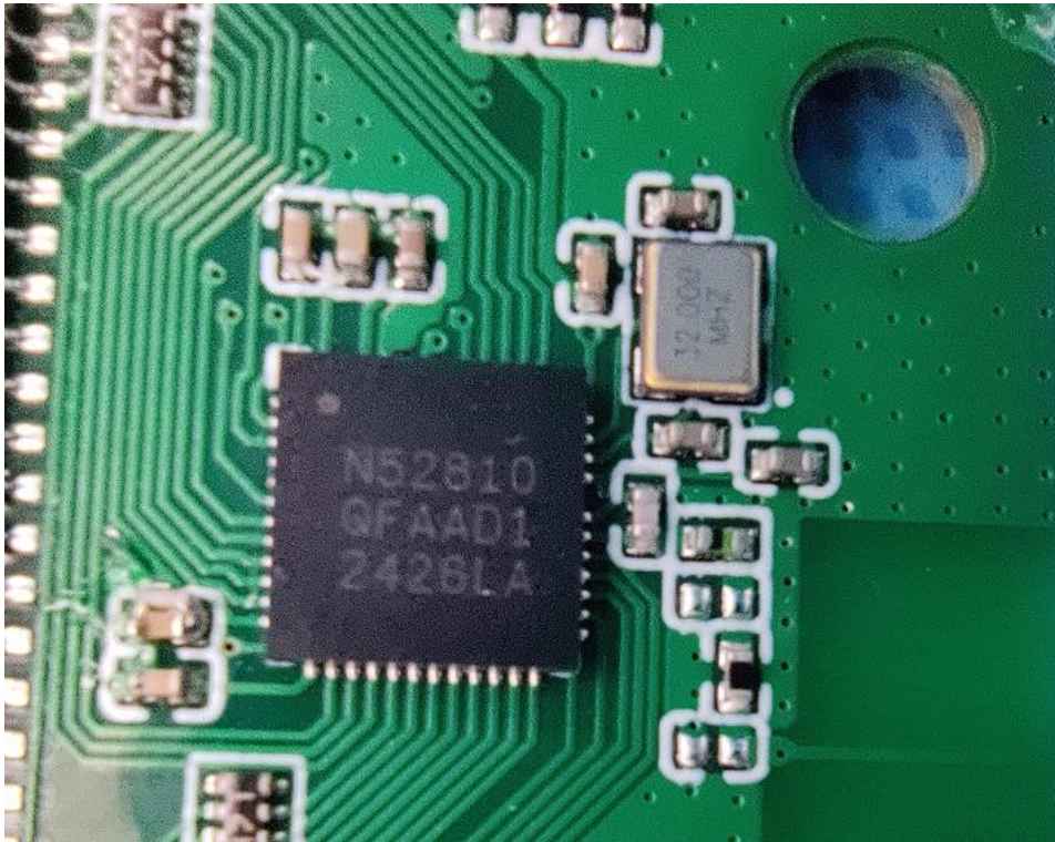
INTERNAL VIEW OF EUT (FIGURE 5)
