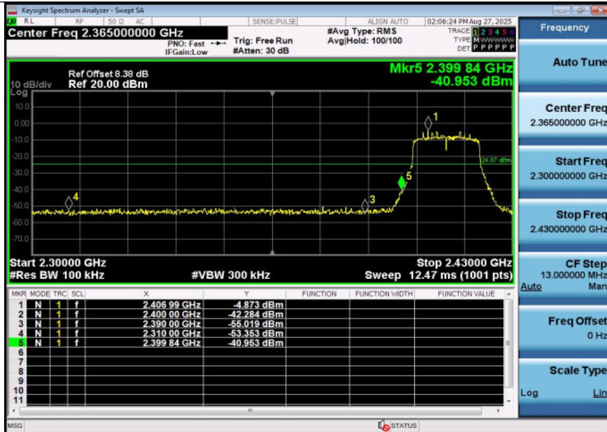
11N20SISO-Ant2-2412-PASS
