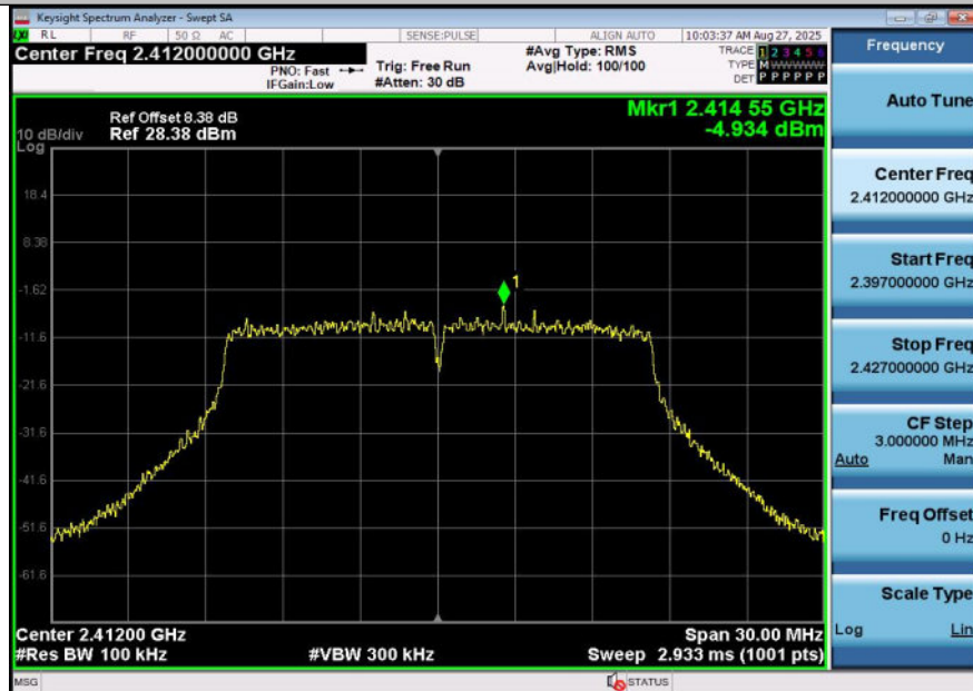
11G-Ant1-2412-0~Reference-PASS
