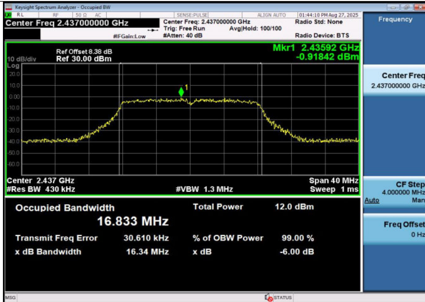
11G-Ant2-2437
