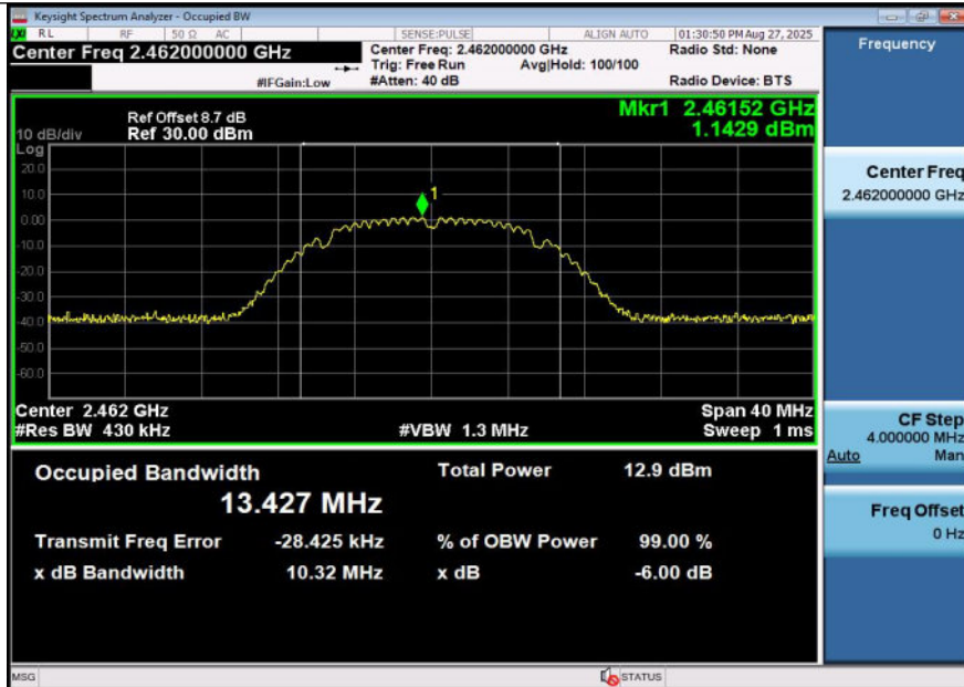
11B-Ant2-2462
