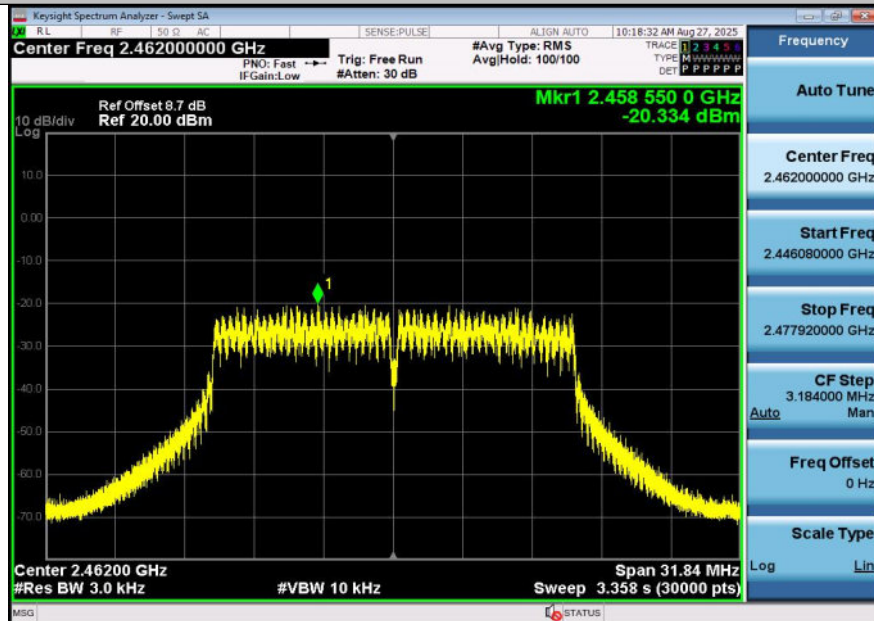
11G-Ant1-2462-PASS
