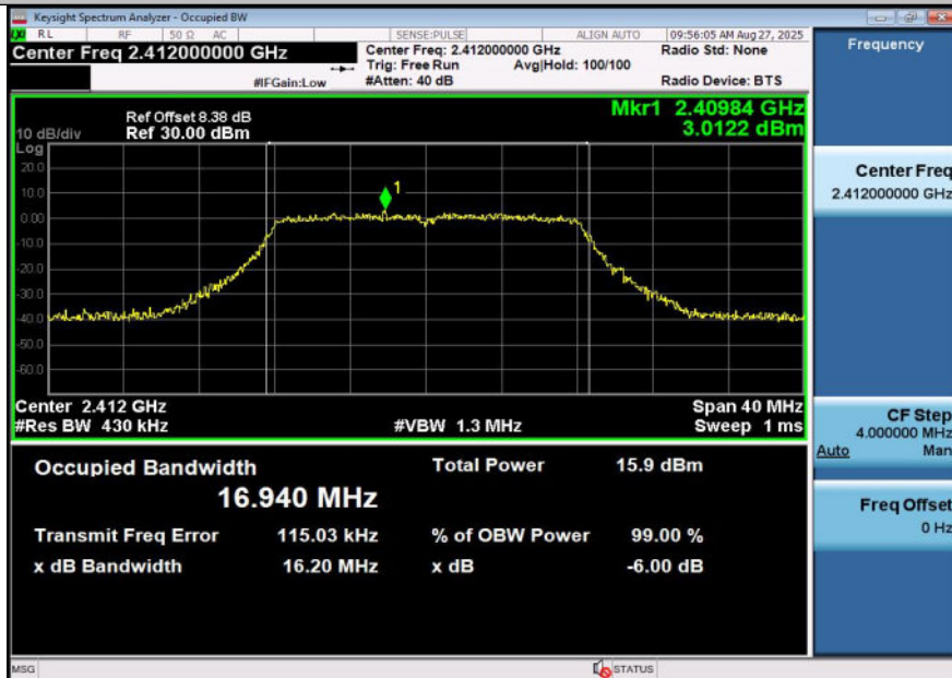
11G-Ant1-2412
