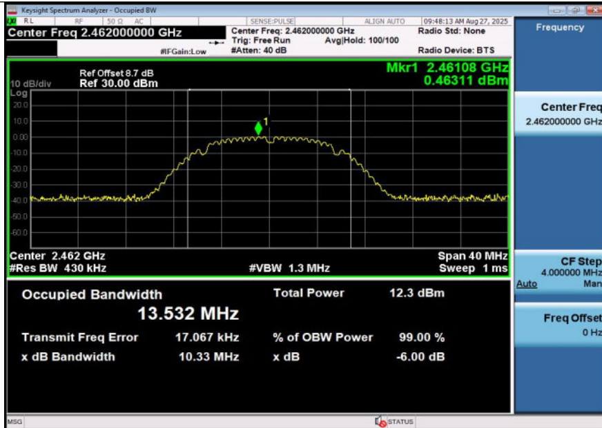
11B-Ant1-2462
