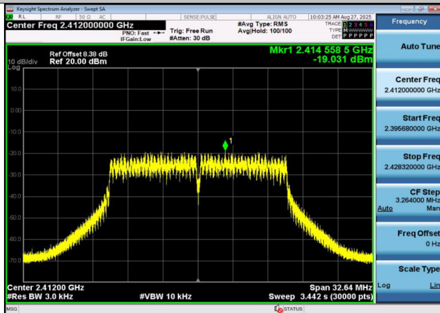
11G-Ant1-2412-PASS
