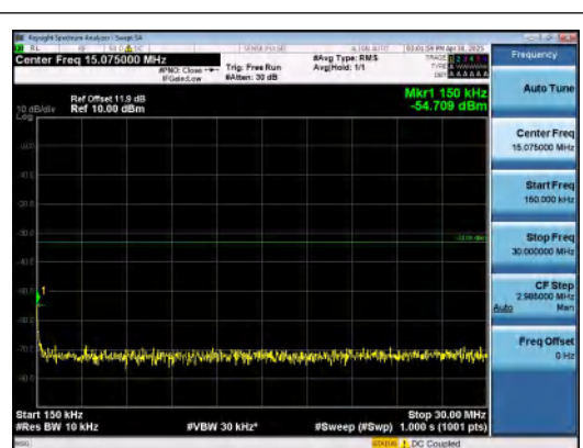
Band2-1.4MHz-QPSK-18607-1RB#0-0.15~30-P ASS
