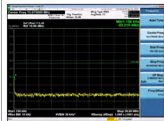
Band2-1.4MHz-QPSK-18900-1RB#5-0.15~30-P ASS
