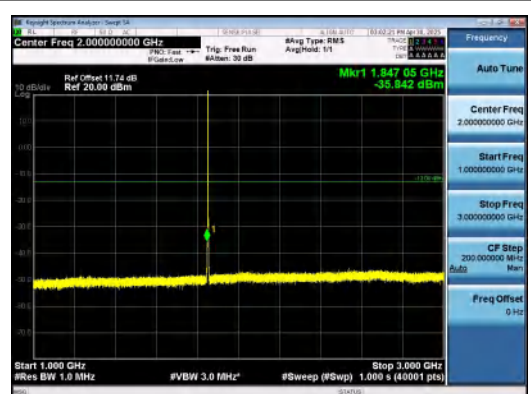
Band2-1.4MHz-QPSK-18607-1RB#0-1000~3000 -PASS
