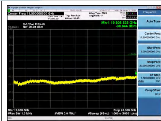
Band2-1.4MHz-QPSK-18900-1RB#0-3000~2000 0-PASS
