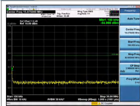
Band2-1.4MHz-16QAM-18607-1RB#0-0.15~30-P ASS
