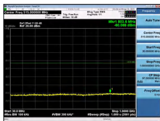
Band2-1.4MHz-QPSK-18900-1RB#5-30~1000-P ASS
