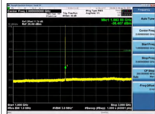
Band2-1.4MHz-QPSK-18900-1RB#5-1000~3000 -PASS
