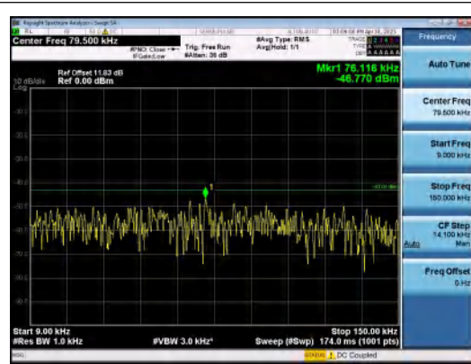
Band2-1.4MHz-QPSK-18900-1RB#5-0.009~0.15 -PASS
