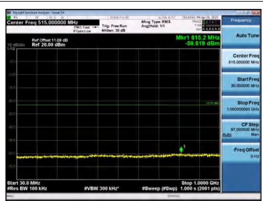
Band2-1.4MHz-16QAM-18607-1RB#0-30~1000-PASS
