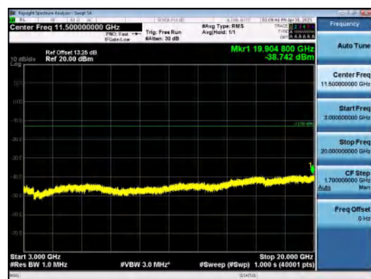
Band2-1.4MHz-QPSK-18900-1RB#5-3000~2000 0-PASS
