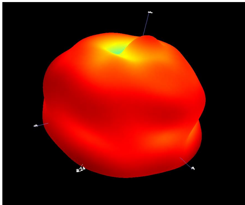
B1.5 3D Pattern for 5500MHz
