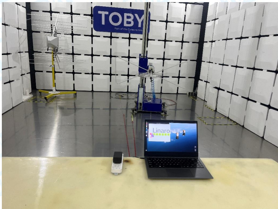
Photo of Setup for Radiated Emission (Below 1 GHz) ----GENBOOK-RK3588-X0
