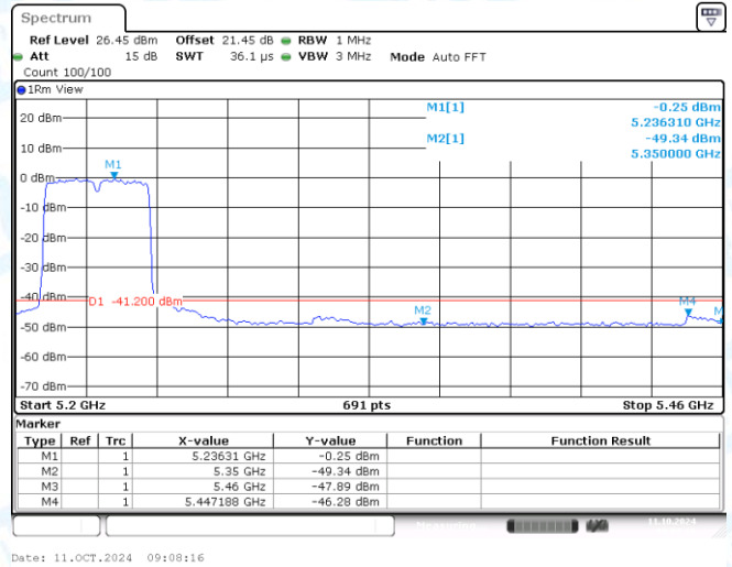
11AX40MIMO-Ant2-5230-PASS
