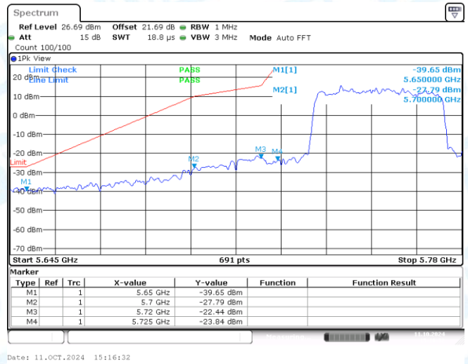
11AX40MIMO-Ant2-5755-PASS
