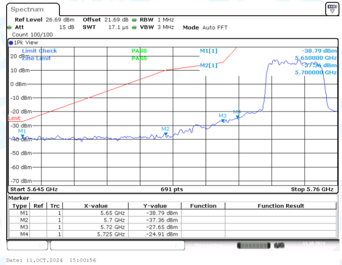
11AX20MIMO-Ant2-5745-PASS
