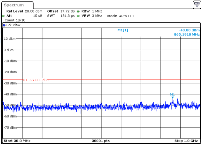
11AX80MIMO-Ant1-5775-30~1000-PASS
