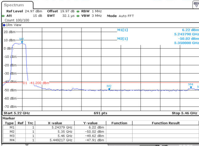
11A-CDD-Ant1-5240-PASS
