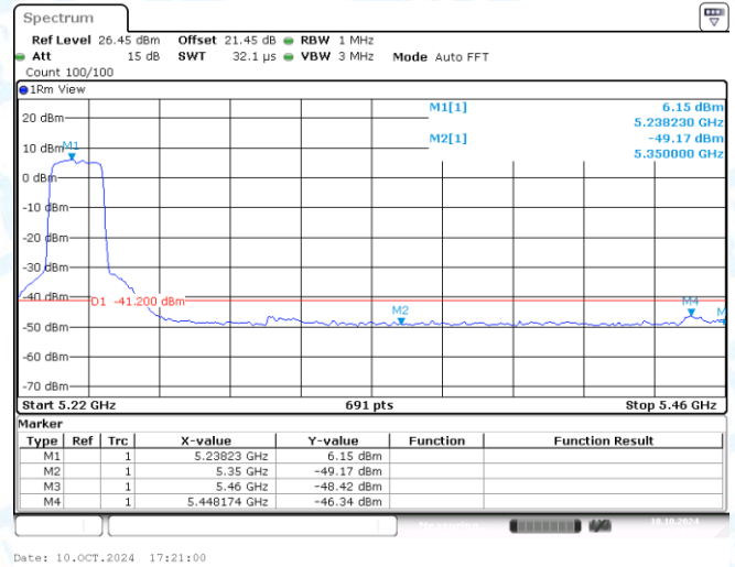
11N20MIMO-Ant2-5240-PASS
