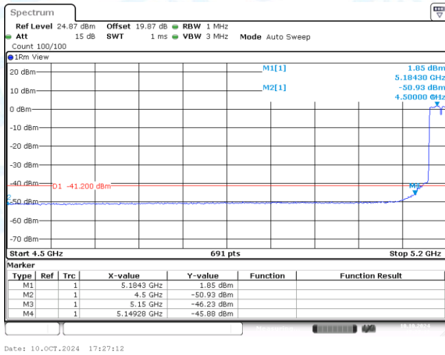
11N40MIMO-Ant1-5190-PASS
