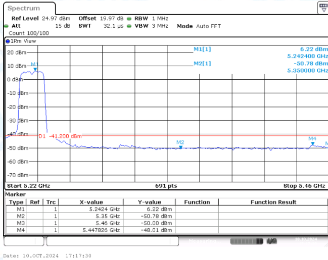
11N20MIMO-Ant1-5240-PASS
