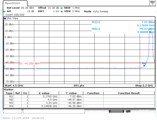
11A-CDD-Ant2-5180-PASS
