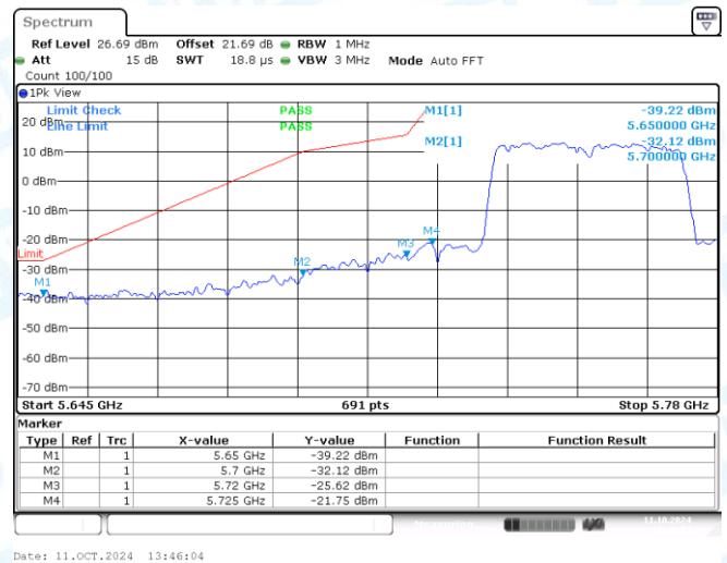
11N40MIMO-Ant2-5755-PASS
