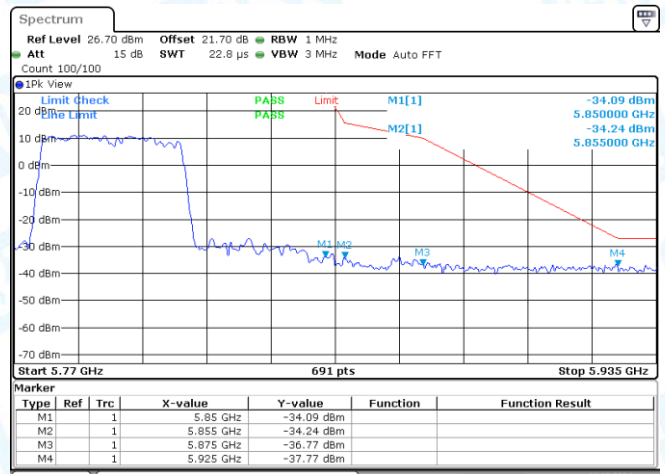
11AC40MIMO-Ant2-5755-PASS
