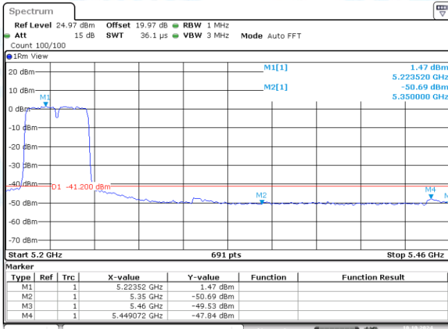
11AC40MIMO-Ant1-5230-PASS
