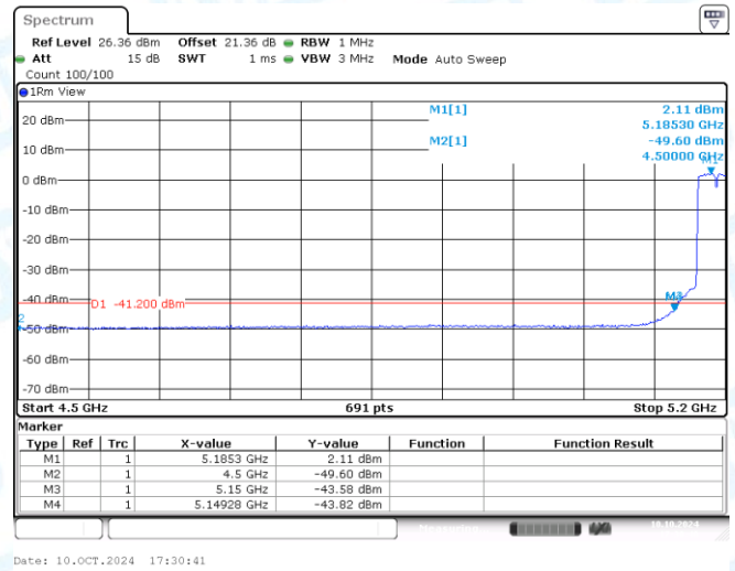
11N40MIMO-Ant2-5190-PASS
