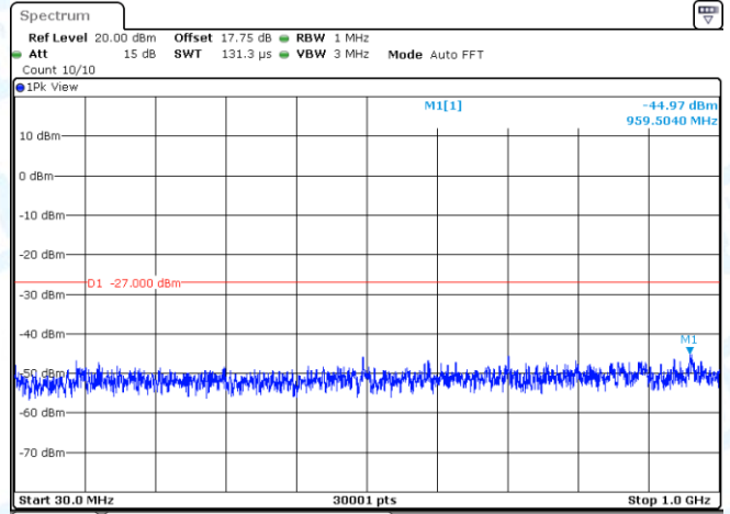
11AX40MIMO-Ant2-5755-30~1000-PASS
