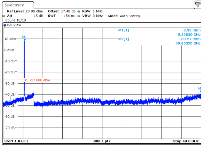
11N40MIMO-Ant1-5230-1000~40000-PASS
