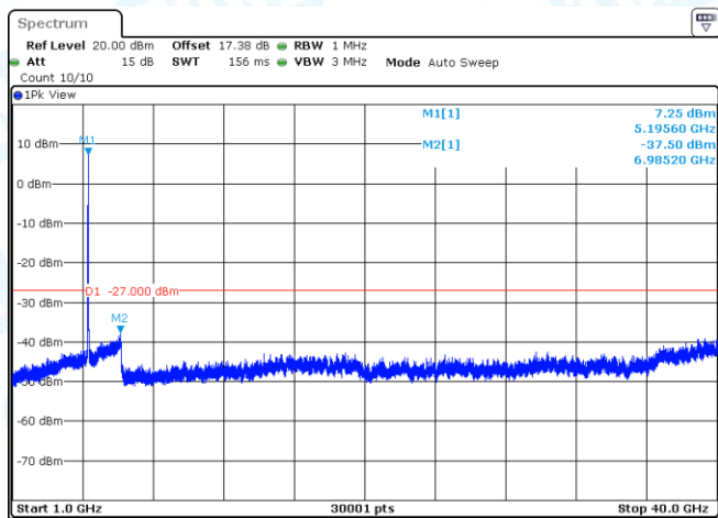
11AC40MIMO-Ant1-5190-1000~40000-PASS
