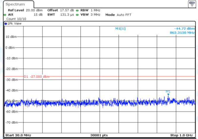
11AX20MIMO-Ant2-5240-30~1000-PASS
