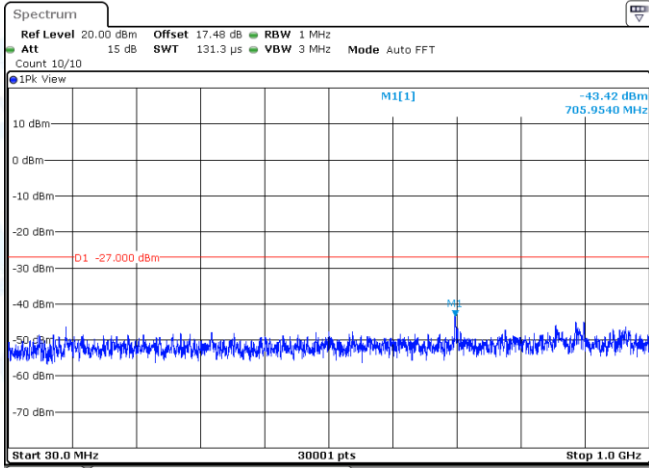
11AC20MIMO-Ant1-5240-30~1000-PASS
