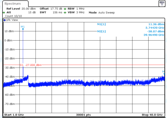
11AC20MIMO-Ant2-5745-1000~40000-PASS
