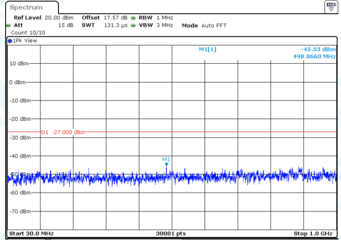
11AC20MIMO-Ant2-5240-30~1000-PASS
