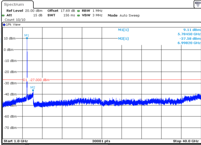
11AC40MIMO-Ant1-5795-1000~40000-PASS
