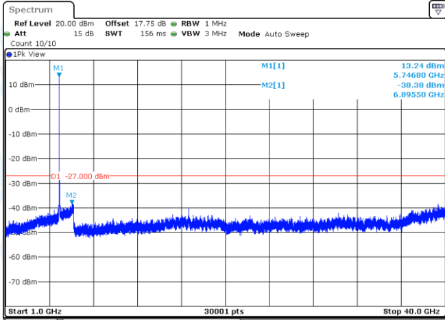
11AC20MIMO-Ant1-5745-1000~40000-PASS
