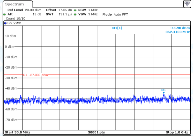
11AC20MIMO-Ant2-5825-30~1000-PASS
