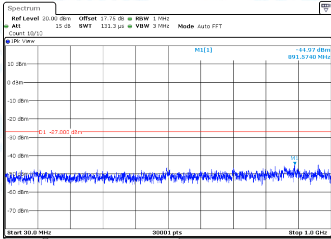
11AC40MIMO-Ant1-5755-30~1000-PASS
