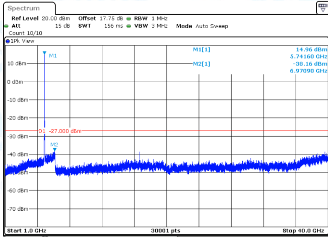
11AX20MIMO-Ant1-5745-1000~40000-PASS
