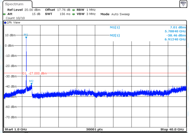
11AC40MIMO-Ant2-5795-1000~40000-PASS
