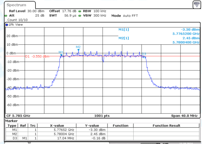
11AC20MIMO-Ant2-5785-PASS
