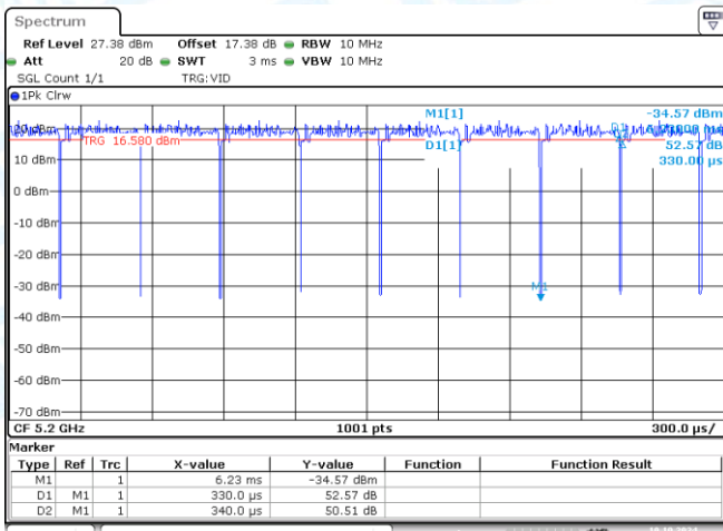
NTNV-11AC20MIMO-Ant1-5180
