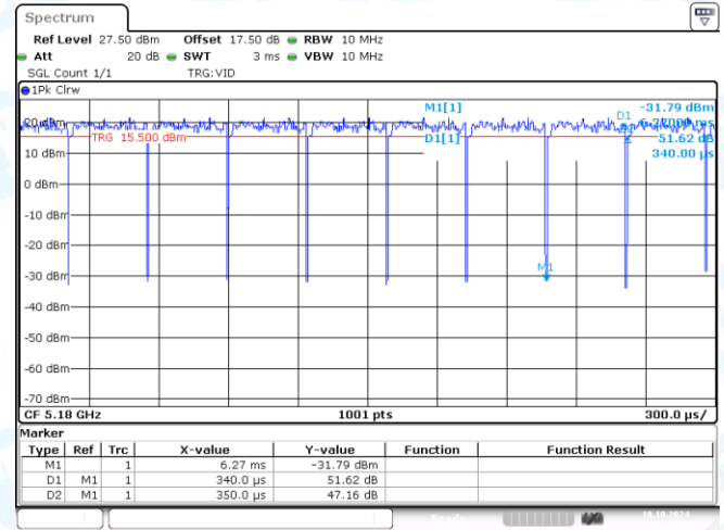
NTNV-11A-CDD-Ant2-5180
