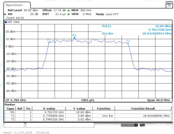
11AX20MIMO-Ant2-5785
