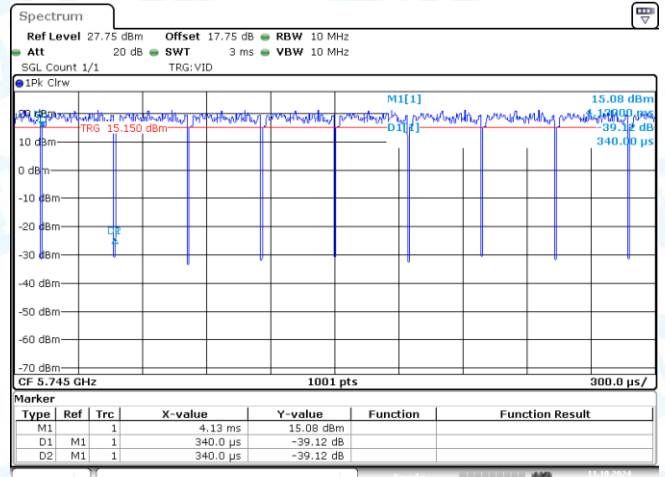
NTNV-11A-CDD-Ant2-5745
