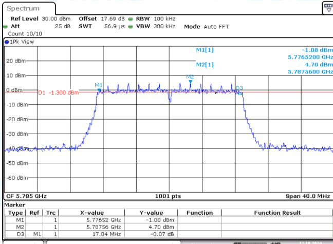
11AC20MIMO-Ant1-5785-PASS
