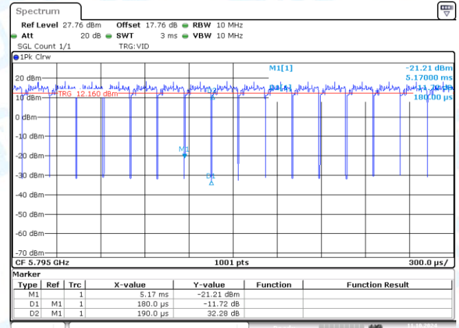
NTNV-11N40MIMO-Ant2-5795
