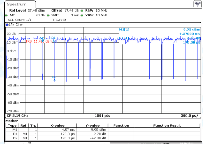
NTNV-11N40MIMO-Ant2-5190
