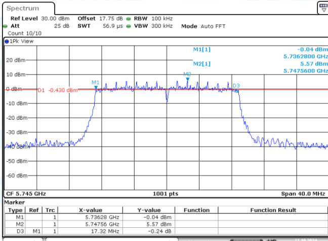
11N20MIMO-Ant1-5745-PASS
