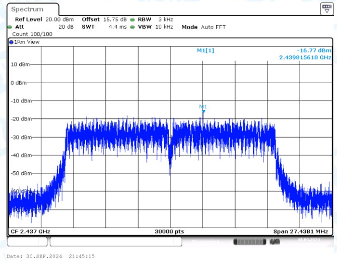
11N20MIMO-Ant2-2437-PASS
