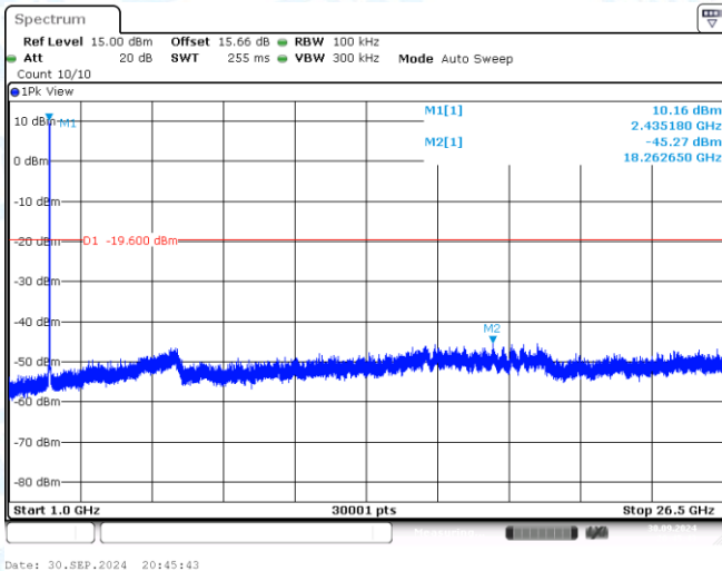
11B-CDD-Ant1-2437-1000~26500-PASS
