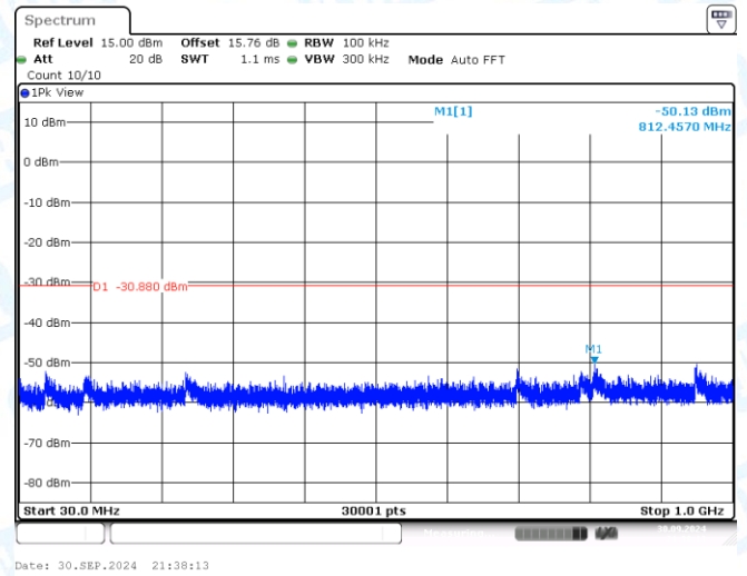
11N20MIMO-Ant2-2412-30~1000-PASS
