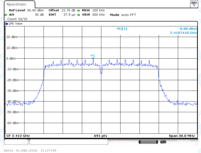
11N20MIMO-Ant2-2412-0~Reference-PASS
