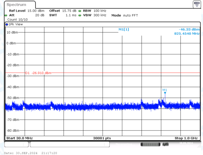
11G-CDD-Ant2-2437-30~1000-PASS
