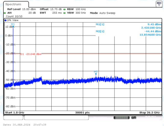
11B-CDD-Ant2-2437-1000~26500-PASS
