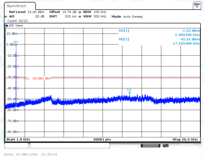
11N20MIMO-Ant2-2412-1000~26500-PASS
