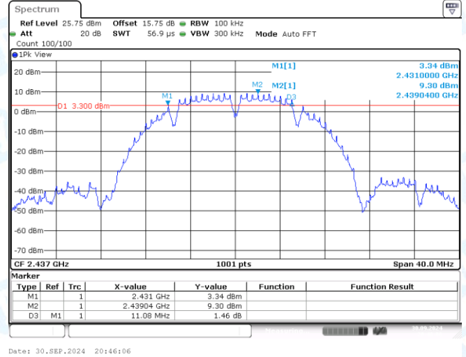
11B-CDD-Ant2-2437-PASS
