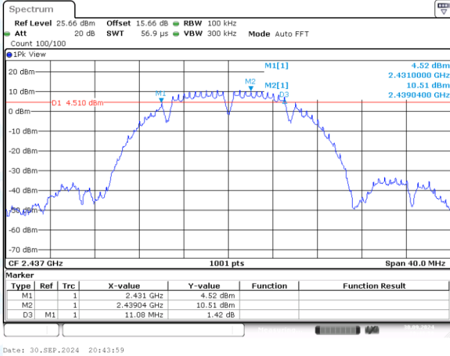
11B-CDD-Ant1-2437-PASS
