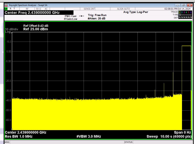
Number of Pulses in 10 seconds
