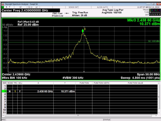
Out Of Band Emission FSK Channel 11
