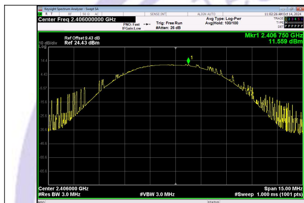
Peak Output Power FSK Channel 00
