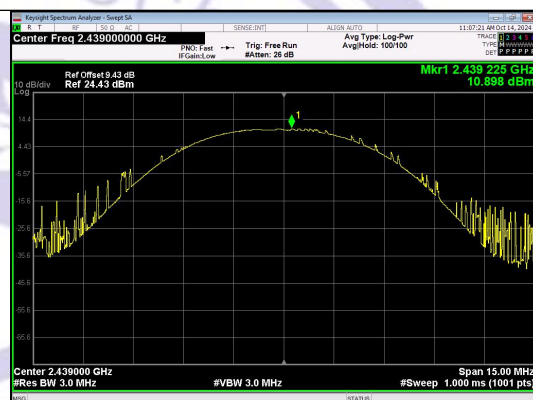
Peak Output Power FSK Channel 11
