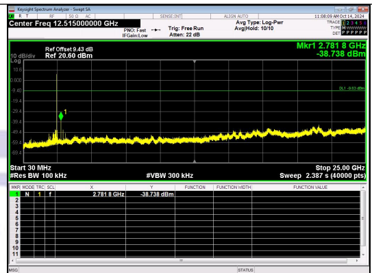
Spurious Emissions FSK Channel 11
