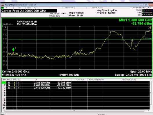
Out Of Band Emission(Left) FSK Channel Hopping
