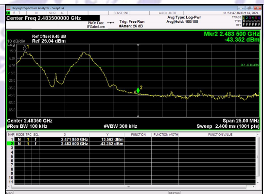
Out Of Band Emission(Right) FSK Channel Hopping
