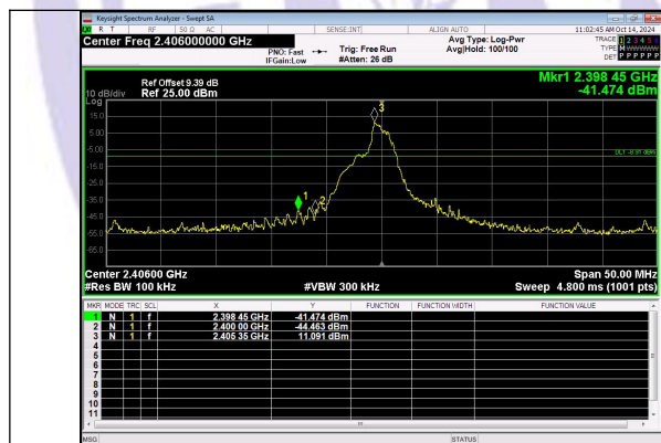
Out Of Band Emission FSK_Channel 0
