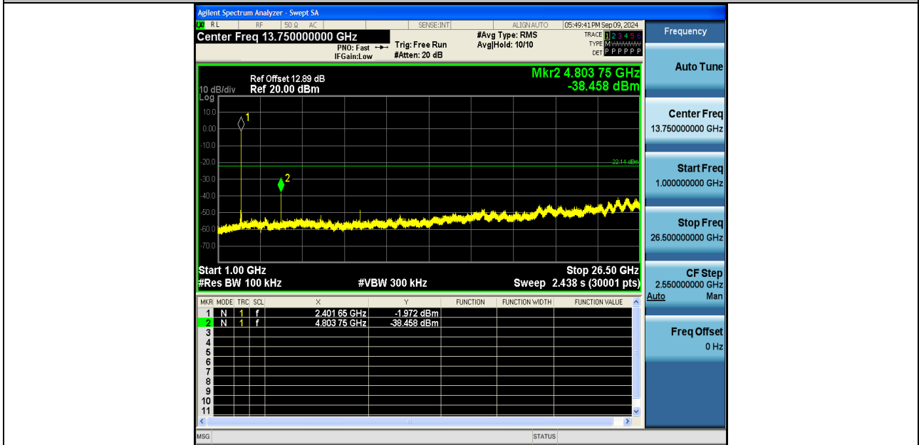
2DH5-Ant1-2402-1000~26500-PASS
