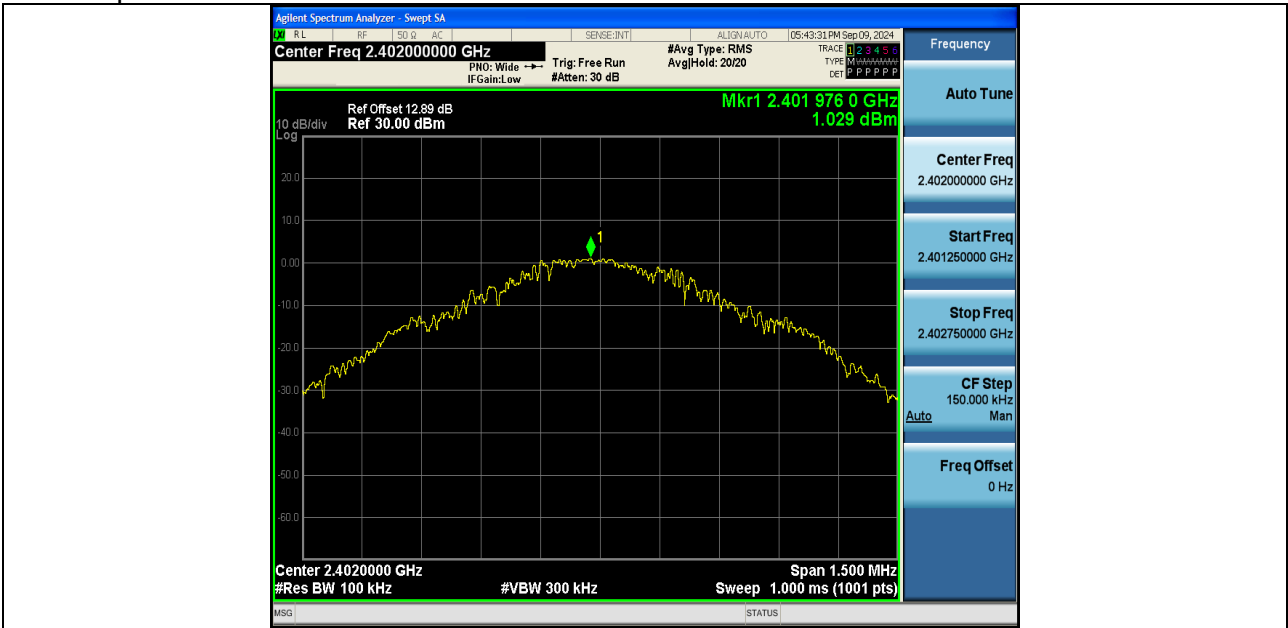
DH5-Ant1-2402-0~Reference-PASS
