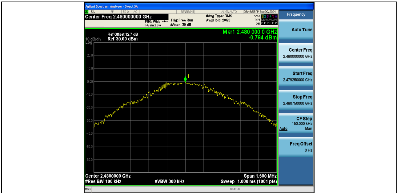
DH5-Ant1-2480-0~Reference-PASS
